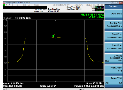
Plot 7-262 PSD SDM Diversity Antenna WF8 (40 MHz BW 802.11be(SU) - Ch.107)
