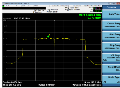
Plot 7-216 PSD SDM Primary Antenna WF5B (160 MHz BW 802.11be(SU) - Ch.143)
