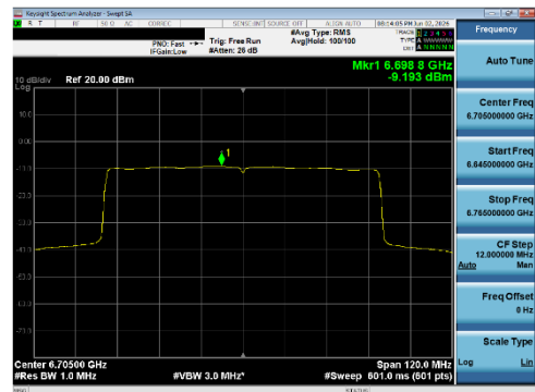
Plot 7-271 PSD SDM Diversity Antenna WF8 (80 MHz BW 802.11be(SU) - Ch.151)
