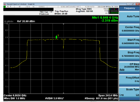
Plot 7-248 PSD CDD Diversity Antenna WF8 (160 MHz BW 802.11be(SU) - Ch.143)
