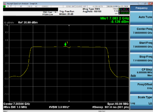
Plot 7-278 PSD SDM Diversity Antenna WF8 (40 MHz BW 802.11be(SU) - Ch.227)
