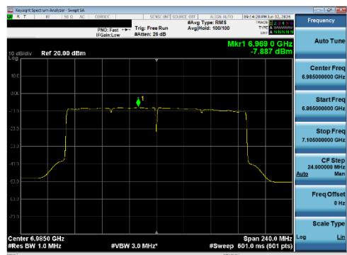
Plot 7-280 PSD SDM Diversity Antenna WF8 (160 MHz BW 802.11be(SU) - Ch.207)
