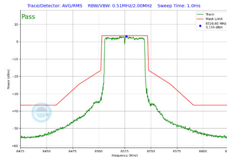
Plot 7-286 In-Band Emission Plot Antenna WF5T (40 MHz BW 802.11be(SU) (UNII Band 6) - Ch.115)
