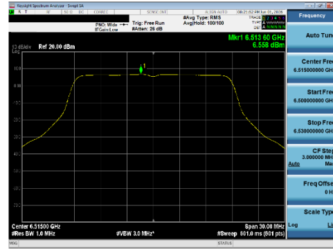
Plot 7-237 PSD CDD Diversity Antenna WF8 (20 MHz BW 802.11a - Ch.113)
