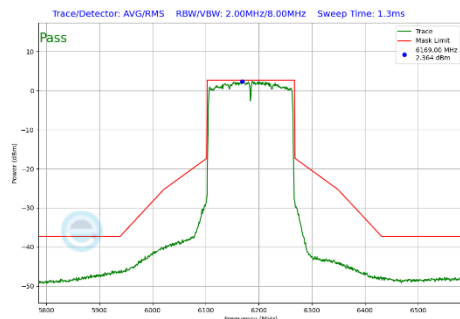
Plot 7-284 In-Band Emission Plot Antenna WF5T (160 MHz BW 802.11be(SU) (UNII Band 5) - Ch.47)
