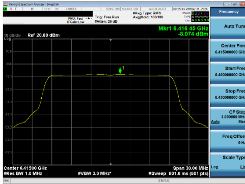
Plot 7-249 PSD SDM Diversity Antenna WF5T (20 MHz BW 802.11be(SU) - Ch.93)
