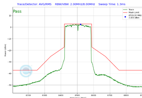
Plot 7-288 In-Band Emission Plot Antenna WF5T (160 MHz BW 802.11be(SU) (UNII Band 6) - Ch.111)
