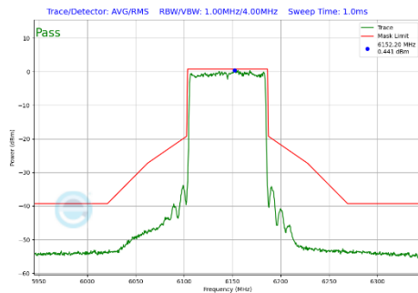
Plot 7-311 In-Band Emission Plot Antenna WF5B (80 MHz BW 802.11be(SU) (UNII Band 5) - Ch.39)
