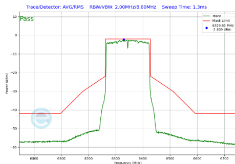
Plot 7-296 In-Band Emission Plot Antenna WF5T (160 MHz BW 802.11be(SU) (UNII Band 5) - Ch.79)
