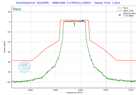
Plot 7-313 In-Band Emission Plot Antenna WF5B (20 MHz BW 802.11a (UNII Band 6) - Ch.105)
