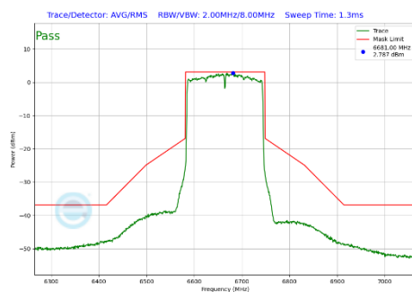
Plot 7-292 In-Band Emission Plot Antenna WF5T (160 MHz BW 802.11be(SU) (UNII Band 7) - Ch.143)
