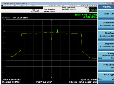
Plot 7-244 PSD CDD Diversity Antenna WF5T (160 MHz BW 802.11be(SU) - Ch.143)
