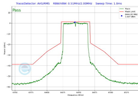
Plot 7-314 In-Band Emission Plot Antenna WF5B (40 MHz BW 802.11be(SU) (UNII Band 6) - Ch.99)
