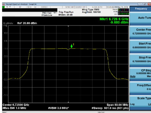
Plot 7-210 PSD SDM Primary Antenna WF5T (40 MHz BW 802.11be(SU) - Ch.155)
