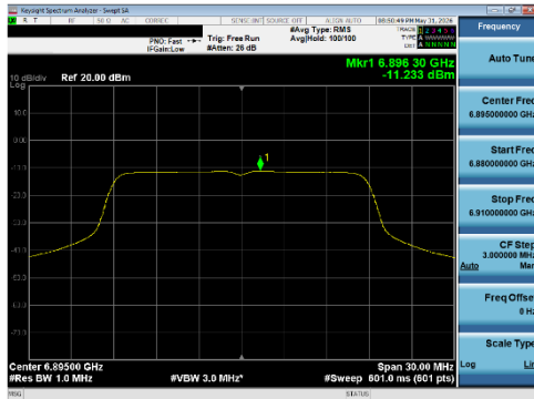
Plot 7-217 PSD CDD Primary Antenna WF5T (20 MHz BW 802.11a - Ch.189)
