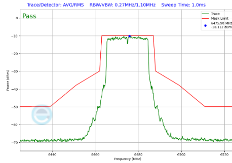
Plot 7-325 In-Band Emission Plot Antenna WF5B (20 MHz BW 802.11be(SU) (UNII Band 6) - Ch.105)
