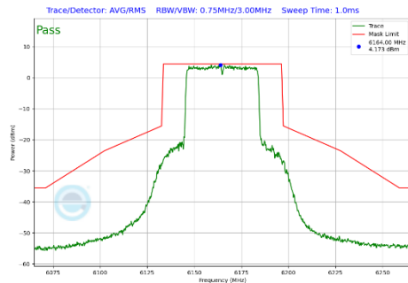
Plot 7-282 In-Band Emission Plot Antenna WF5T (40 MHz BW 802.11be(SU) (UNII Band 5) - Ch.43)
