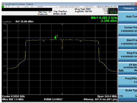
Plot 7-236 PSD CDD Diversity Antenna WF5T (160 MHz BW 802.11be(SU) - Ch.111)
