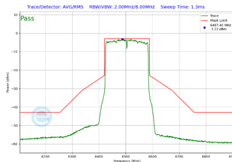
Plot 7-300 In-Band Emission Plot Antenna WF5T (160 MHz BW 802.11be(SU) (UNII Band 6) - Ch.111)
