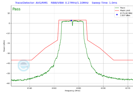
Plot 7-281 In-Band Emission Plot Antenna WF5T (20 MHz BW 802.11a (UNII Band 5) - Ch.45)
