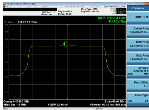
Plot 7-254 PSD SDM Diversity Antenna WF8 (40 MHz BW 802.11be(SU) - Ch.91)
