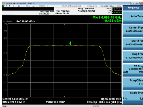
Plot 7-209 PSD SDM Primary Antenna WF5T (20 MHz BW 802.11be(SU) - Ch.149)
