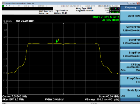
Plot 7-218 PSD SDM Primary Antenna WF5T (40 MHz BW 802.11be(SU) - Ch.227)
