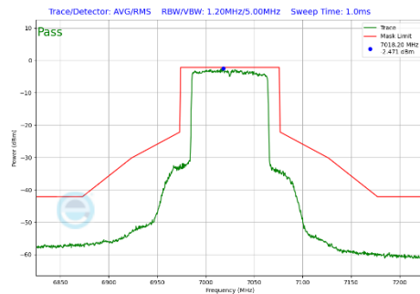
Plot 7-335 In-Band Emission Plot Antenna WF5B (80 MHz BW 802.11be(SU) (UNII Band 8) - Ch.215)
