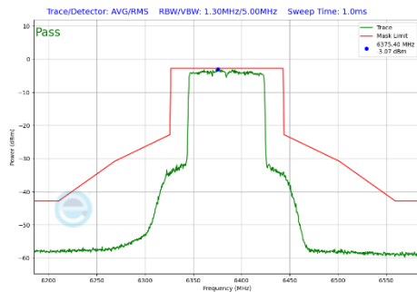
Plot 7-323 In-Band Emission Plot Antenna WF5B (80 MHz BW 802.11be(SU) (UNII Band 5) - Ch.87)
