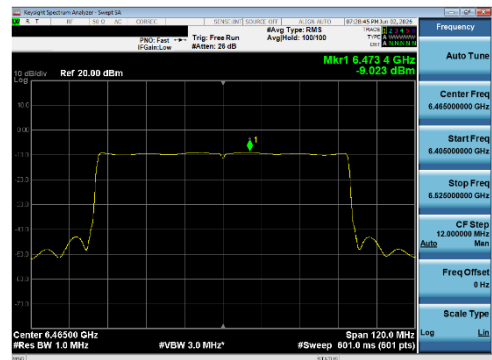
Plot 7-263 PSD SDM Diversity Antenna WF8 (80 MHz BW 802.11be(SU) - Ch.103)
