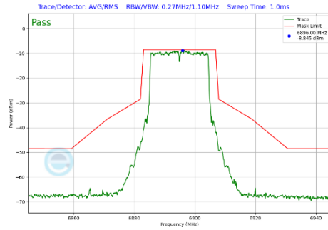
Plot 7-333 In-Band Emission Plot Antenna WF5B (20 MHz BW 802.11be(SU) (UNII Band 8) - Ch.189)
