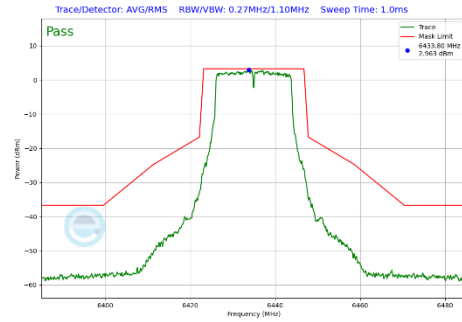
Plot 7-285 In-Band Emission Plot Antenna WF5T (20 MHz BW 802.11a (UNII Band 6) - Ch.97)
