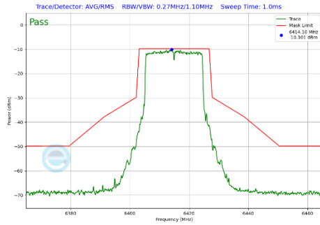
Plot 7-293 In-Band Emission Plot Antenna WF5T (20 MHz BW 802.11be(SU) (UNII Band 5) - Ch.93)
