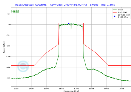
Plot 7-320 In-Band Emission Plot Antenna WF5B (160 MHz BW 802.11be(SU) (UNII Band 7) - Ch.143)
