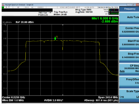
Plot 7-228 PSD CDD Diversity Antenna WF5T (160 MHz BW 802.11be(SU) - Ch.15)
