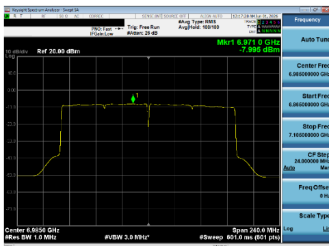
Plot 7-276 PSD SDM Diversity Antenna WF5T (160 MHz BW 802.11be(SU) - Ch.207)
