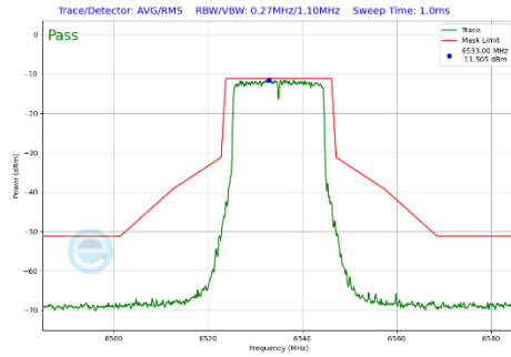
Plot 7-301 In-Band Emission Plot Antenna WF5T (20 MHz BW 802.11be(SU) (UNII Band 7) - Ch.117)
