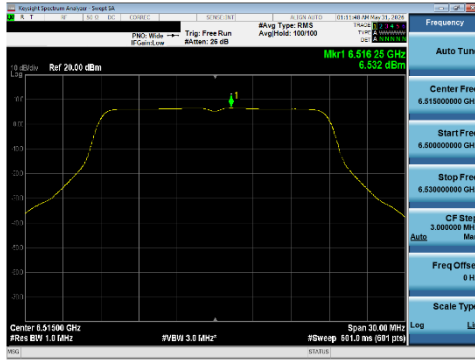
Plot 7-233 PSD CDD Diversity Antenna WF5T (20 MHz BW 802.11a - Ch.113)
