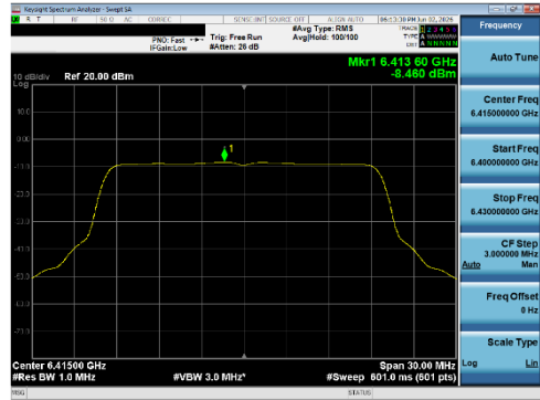
Plot 7-253 PSD SDM Diversity Antenna WF8 (20 MHz BW 802.11be(SU) - Ch.93)
