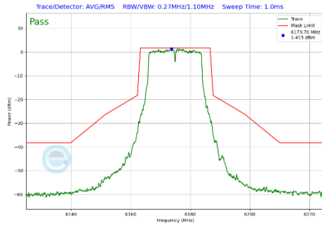
Plot 7-309 In-Band Emission Plot Antenna WF5B (20 MHz BW 802.11a (UNII Band 5) - Ch.45)
