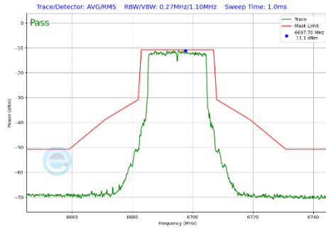
Plot 7-329 In-Band Emission Plot Antenna WF5B (20 MHz BW 802.11be(SU) (UNII Band 7) - Ch.149)
