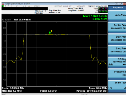
Plot 7-227 PSD CDD Diversity Antenna WF5T (80 MHz BW 802.11be(SU) - Ch.7)
