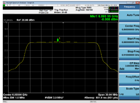
Plot 7-277 PSD SDM Diversity Antenna WF8 (20 MHz BW 802.11be(SU) - Ch.189)
