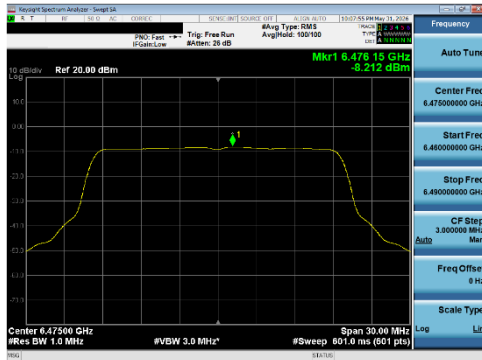
Plot 7-257 PSD SDM Diversity Antenna WF5T (20 MHz BW 802.11be(SU) - Ch.105)
