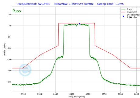
Plot 7-315 In-Band Emission Plot Antenna WF5B (80 MHz BW 802.11be(SU) (UNII Band 6) - Ch.103)
