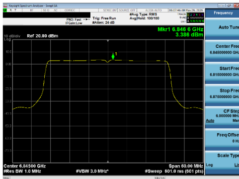
Plot 7-242 PSD CDD Diversity Antenna WF5T (40 MHz BW 802.11be(SU) - Ch.179)
