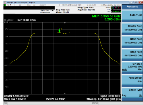
Plot 7-229 PSD CDD Diversity Antenna WF8 (20 MHz BW 802.11a - Ch.1)
