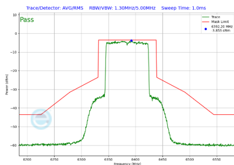
Plot 7-295 In-Band Emission Plot Antenna WF5T (80 MHz BW 802.11be(SU) (UNII Band 5) - Ch.87)
