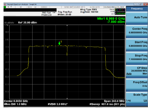
Plot 7-224 PSD SDM Primary Antenna WF5B (160 MHz BW 802.11be(SU) - Ch.207)
