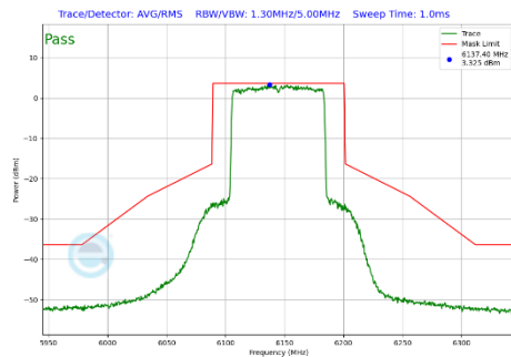
Plot 7-283 In-Band Emission Plot Antenna WF5T (80 MHz BW 802.11be(SU) (UNII Band 5) - Ch.39)
