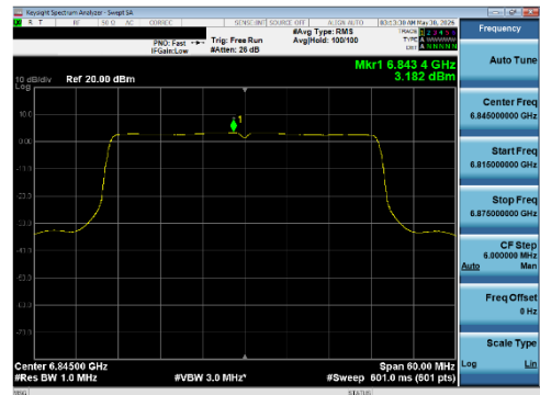
Plot 7-246 PSD CDD Diversity Antenna WF8 (40 MHz BW 802.11be(SU) - Ch.179)
