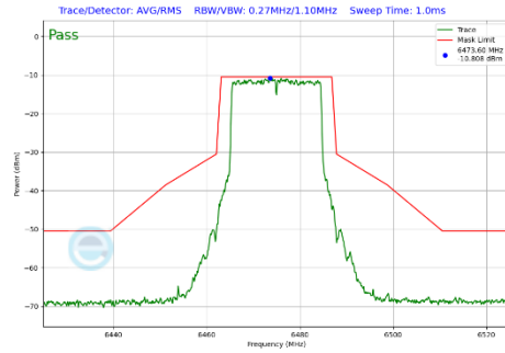
Plot 7-297 In-Band Emission Plot Antenna WF5T (20 MHz BW 802.11be(SU) (UNII Band 6) - Ch.105)
