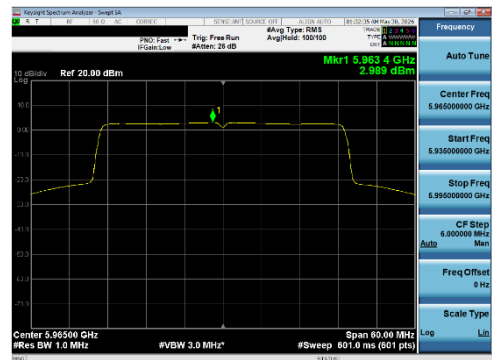
Plot 7-230 PSD CDD Diversity Antenna WF8 (40 MHz BW 802.11be(SU) - Ch.3)
