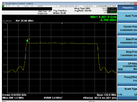
Plot 7-219 PSD SDM Primary Antenna WF5T (80 MHz BW 802.11be(SU) - Ch.199)
