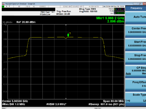
Plot 7-226 PSD CDD Diversity Antenna WF5T (40 MHz BW 802.11be(SU) - Ch.3)
