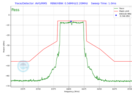
Plot 7-322 In-Band Emission Plot Antenna WF5B (40 MHz BW 802.11be(SU) (UNII Band 5) - Ch.91)
