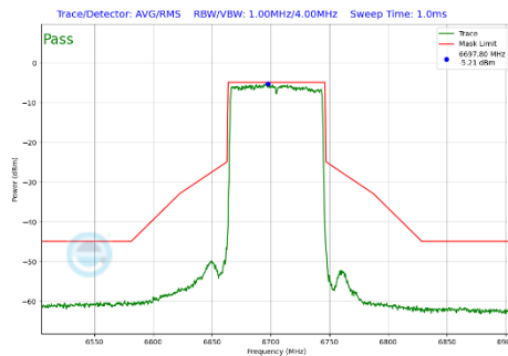
Plot 7-331 In-Band Emission Plot Antenna WF5B (80 MHz BW 802.11be(SU) (UNII Band 7) - Ch.151)
