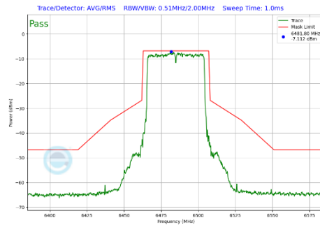
Plot 7-326 In-Band Emission Plot Antenna WF5B (40 MHz BW 802.11be(SU) (UNII Band 6) - Ch.107)
