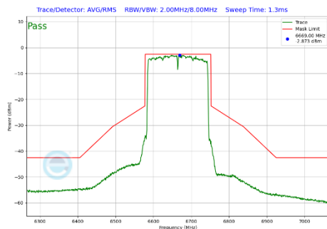
Plot 7-332 In-Band Emission Plot Antenna WF5B (160 MHz BW 802.11be(SU) (UNII Band 7) - Ch.143)
