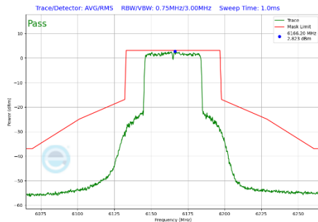
Plot 7-310 In-Band Emission Plot Antenna WF5B (40 MHz BW 802.11be(SU) (UNII Band 5) - Ch.43)
