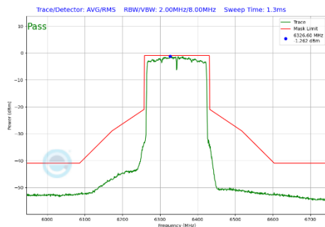
Plot 7-324 In-Band Emission Plot Antenna WF5B (160 MHz BW 802.11be(SU) (UNII Band 5) - Ch.79)
