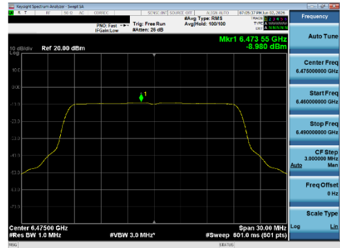
Plot 7-261 PSD SDM Diversity Antenna WF8 (20 MHz BW 802.11be(SU) - Ch.105)
