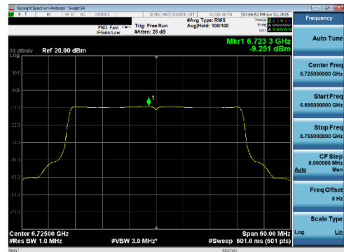
Plot 7-270 PSD SDM Diversity Antenna WF8 (40 MHz BW 802.11be(SU) - Ch.155)
