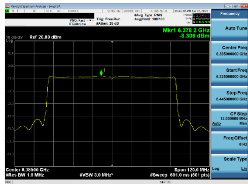
Plot 7-255 PSD SDM Diversity Antenna WF8 (80 MHz BW 802.11be(SU) - Ch.87)
