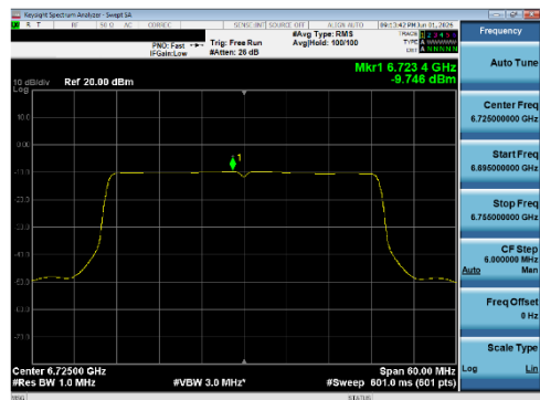
Plot 7-214 PSD SDM Primary Antenna WF5B (40 MHz BW 802.11be(SU) - Ch.155)
