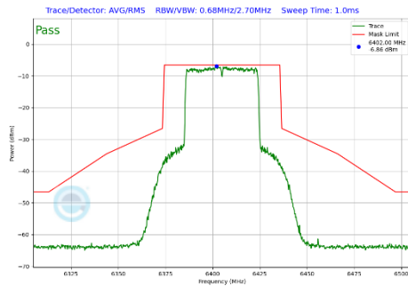
Plot 7-294 In-Band Emission Plot Antenna WF5T (40 MHz BW 802.11be(SU) (UNII Band 5) - Ch.91)
