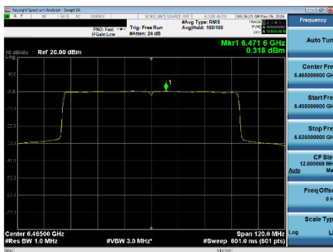
Plot 7-235 PSD CDD Diversity Antenna WF5T (80 MHz BW 802.11be(SU) - Ch.103)
