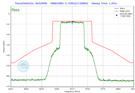
Plot 7-330 In-Band Emission Plot Antenna WF5B (40 MHz BW 802.11be(SU) (UNII Band 7) - Ch.155)
