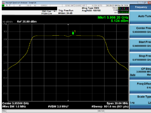
Plot 7-225 PSD CDD Diversity Antenna WF5T (20 MHz BW 802.11a - Ch.1)
