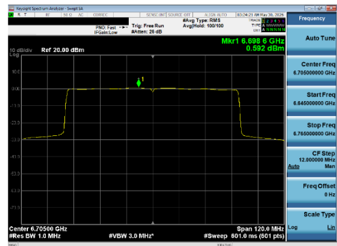
Plot 7-247 PSD CDD Diversity Antenna WF8 (80 MHz BW 802.11be(SU) - Ch.151)
