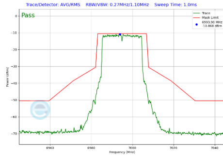
Plot 7-305 In-Band Emission Plot Antenna WF5T (20 MHz BW 802.11be(SU) (UNII Band 8) - Ch.209)
