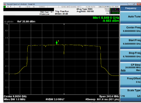
Plot 7-272 PSD SDM Diversity Antenna WF8 (160 MHz BW 802.11be(SU) - Ch.143)
