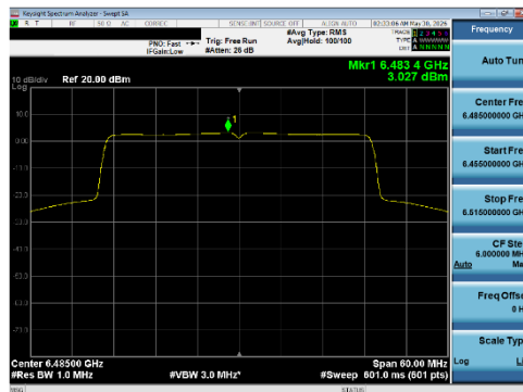
Plot 7-238 PSD CDD Diversity Antenna WF8 (40 MHz BW 802.11be(SU) - Ch.107)
