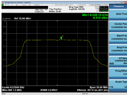
Plot 7-265 PSD SDM Diversity Antenna WF5T (20 MHz BW 802.11be(SU) - Ch.117)
