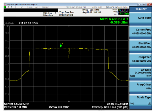
Plot 7-264 PSD SDM Diversity Antenna WF8 (160 MHz BW 802.11be(SU) - Ch.111)
