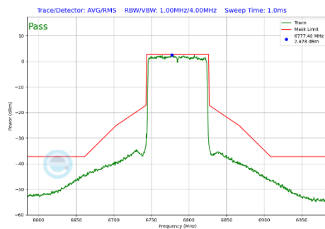
Plot 7-291 In-Band Emission Plot Antenna WF5T (80 MHz BW 802.11be(SU) (UNII Band 7) - Ch.167)
