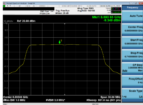
Plot 7-213 PSD SDM Primary Antenna WF5B (20 MHz BW 802.11be(SU) - Ch.149)
