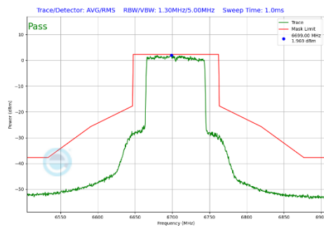
Plot 7-319 In-Band Emission Plot Antenna WF5B (80 MHz BW 802.11be(SU) (UNII Band 7) - Ch.151)
