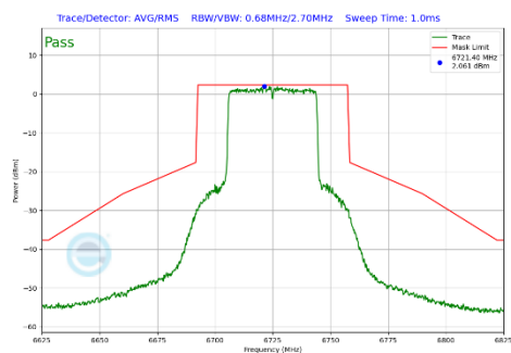
Plot 7-318 In-Band Emission Plot Antenna WF5B (40 MHz BW 802.11be(SU) (UNII Band 7) - Ch.155)
