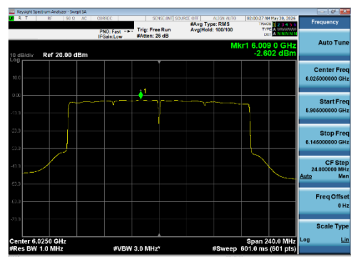
Plot 7-232 PSD CDD Diversity Antenna WF8 (160 MHz BW 802.11be(SU) - Ch.15)
