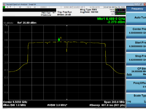
Plot 7-240 PSD CDD Diversity Antenna WF8 (160 MHz BW 802.11be(SU) - Ch.111)
