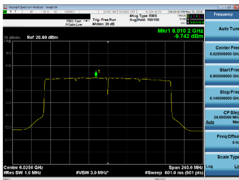
Plot 7-252 PSD SDM Diversity Antenna WF5T (160 MHz BW 802.11be(SU) - Ch.15)
