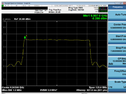
Plot 7-275 PSD SDM Diversity Antenna WF5T (80 MHz BW 802.11be(SU) - Ch.199)
