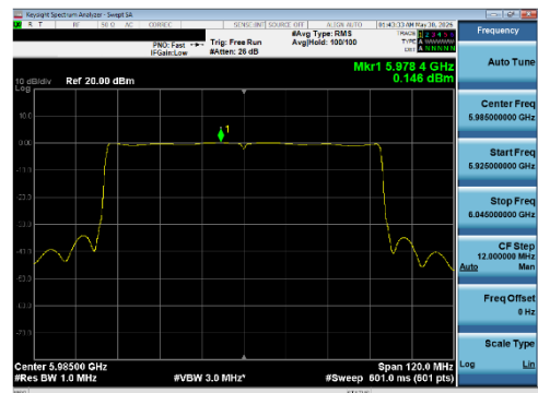
Plot 7-231 PSD CDD Diversity Antenna WF8 (80 MHz BW 802.11be(SU) - Ch.7)
