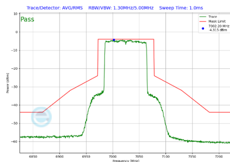
Plot 7-307 In-Band Emission Plot Antenna WF5T (80 MHz BW 802.11be(SU) (UNII Band 8) - Ch.215)
