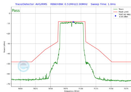
Plot 7-306 In-Band Emission Plot Antenna WF5T (40 MHz BW 802.11be(SU) (UNII Band 8) - Ch.227)
