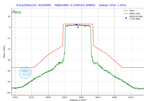
Plot 7-290 In-Band Emission Plot Antenna WF5T (40 MHz BW 802.11be(SU) (UNII Band 7) - Ch.179)
