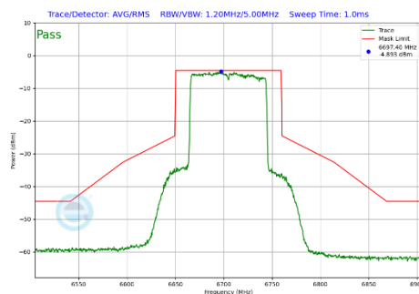
Plot 7-303 In-Band Emission Plot Antenna WF5T (80 MHz BW 802.11be(SU) (UNII Band 7) - Ch.151)
