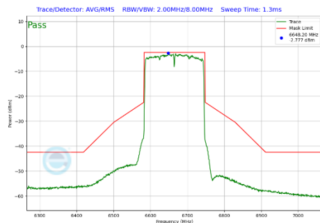
Plot 7-304 In-Band Emission Plot Antenna WF5T (160 MHz BW 802.11be(SU) (UNII Band 7) - Ch.143)
