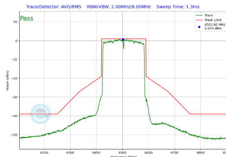
Plot 7-316 In-Band Emission Plot Antenna WF5B (160 MHz BW 802.11be(SU) (UNII Band 6) - Ch.111)
