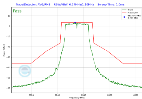
Plot 7-289 In-Band Emission Plot Antenna WF5T (20 MHz BW 802.11a (UNII Band 7) - Ch.181)
