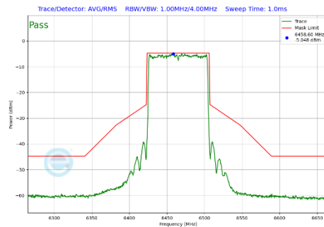
Plot 7-327 In-Band Emission Plot Antenna WF5B (80 MHz BW 802.11be(SU) (UNII Band 6) - Ch.103)
