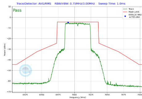
Plot 7-334 In-Band Emission Plot Antenna WF5B (40 MHz BW 802.11be(SU) (UNII Band 8) - Ch.211)
