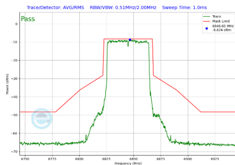
Plot 7-302 In-Band Emission Plot Antenna WF5T (40 MHz BW 802.11be(SU) (UNII Band 7) - Ch.179)
