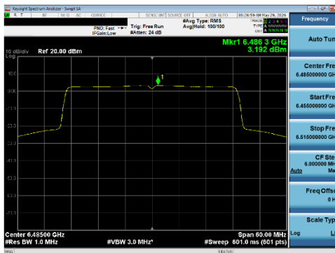
Plot 7-234 PSD CDD Diversity Antenna WF5T (40 MHz BW 802.11be(SU) - Ch.107)
