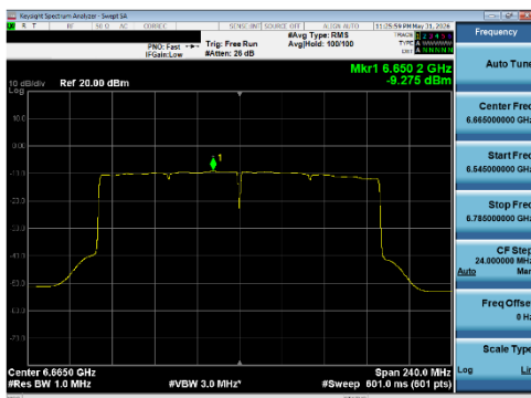
Plot 7-268 PSD SDM Diversity Antenna WF5T (160 MHz BW 802.11be(SU) - Ch.143)
