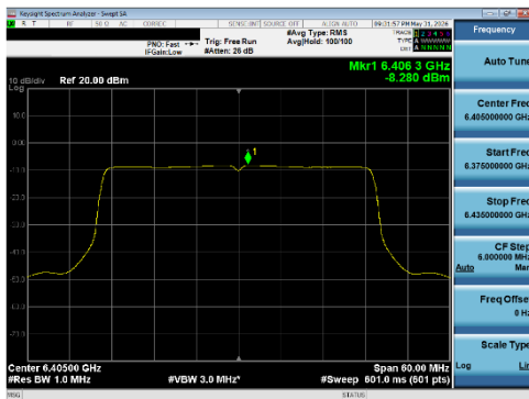
Plot 7-250 PSD SDM Diversity Antenna WF5T (40 MHz BW 802.11be(SU) - Ch.91)
