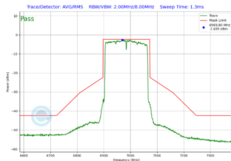
Plot 7-308 In-Band Emission Plot Antenna WF5T (160 MHz BW 802.11be(SU) (UNII Band 8) - Ch.207)
