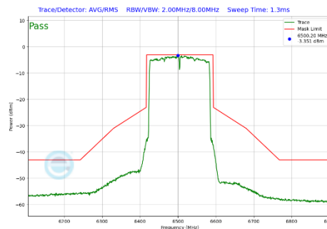
Plot 7-328 In-Band Emission Plot Antenna WF5B (160 MHz BW 802.11be(SU) (UNII Band 6) - Ch.111)
