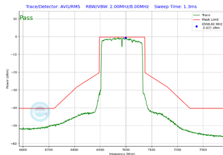
Plot 7-336 In-Band Emission Plot Antenna WF5B (160 MHz BW 802.11be(SU) (UNII Band 8) - Ch.207)
