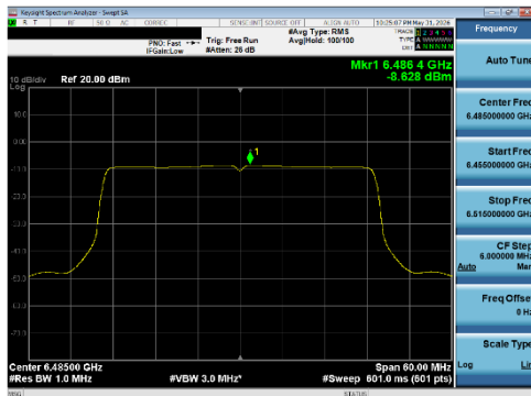
Plot 7-258 PSD SDM Diversity Antenna WF5T (40 MHz BW 802.11be(SU) - Ch.107)
