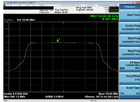
Plot 7-269 PSD SDM Diversity Antenna WF8 (20 MHz BW 802.11be(SU) - Ch.117)
