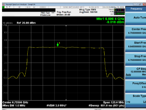
Plot 7-211 PSD SDM Primary Antenna WF5T (80 MHz BW 802.11be(SU) - Ch.151)
