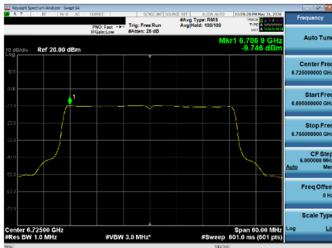
Plot 7-266 PSD SDM Diversity Antenna WF5T (40 MHz BW 802.11be(SU) - Ch.155)
