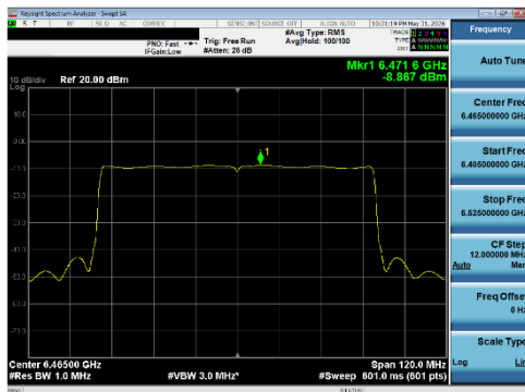
Plot 7-259 PSD SDM Diversity Antenna WF5T (80 MHz BW 802.11be(SU) - Ch.103)
