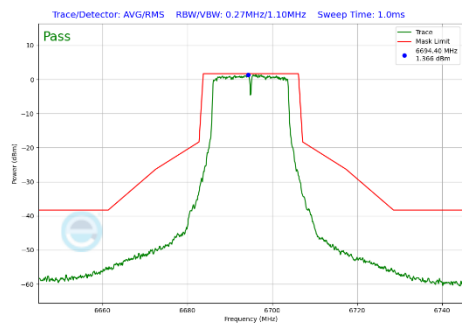
Plot 7-317 In-Band Emission Plot Antenna WF5B (20 MHz BW 802.11a (UNII Band 7) - Ch.149)
