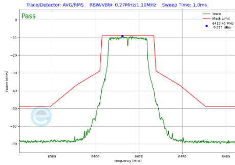
Plot 7-321 In-Band Emission Plot Antenna WF5B (20 MHz BW 802.11a (UNII Band 5) - Ch.93)
