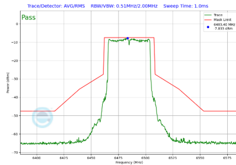
Plot 7-298 In-Band Emission Plot Antenna WF5T (40 MHz BW 802.11be(SU) (UNII Band 6) - Ch.107)
