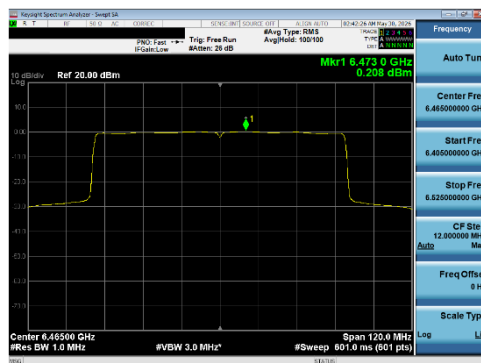
Plot 7-239 PSD CDD Diversity Antenna WF8 (80 MHz BW 802.11be(SU) - Ch.103)
