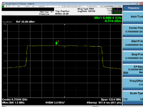
Plot 7-267 PSD SDM Diversity Antenna WF5T (80 MHz BW 802.11be(SU) - Ch.151)
