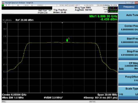
Plot 7-273 PSD SDM Diversity Antenna WF5T (20 MHz BW 802.11be(SU) - Ch.189)
