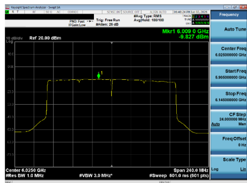
Plot 7-256 PSD SDM Diversity Antenna WF8 (160 MHz BW 802.11be(SU) - Ch.15)
