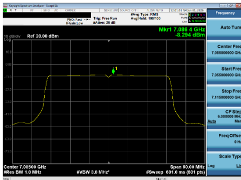
Plot 7-274 PSD SDM Diversity Antenna WF5T (40 MHz BW 802.11be(SU) - Ch.227)
