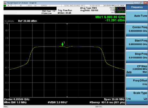
Plot 7-221 PSD CDD Primary Antenna WF5B (20 MHz BW 802.11a - Ch.189)
