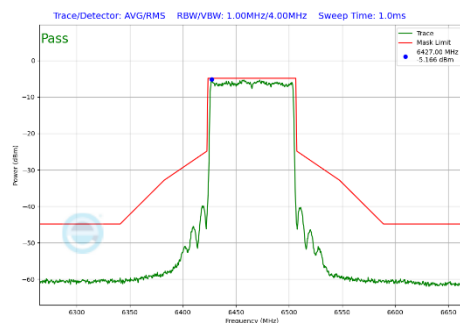
Plot 7-299 In-Band Emission Plot Antenna WF5T (80 MHz BW 802.11be(SU) (UNII Band 6) - Ch.103)
