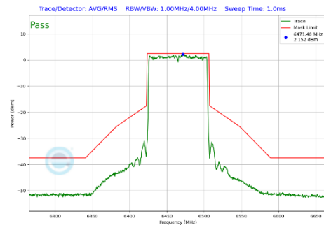
Plot 7-287 In-Band Emission Plot Antenna WF5T (80 MHz BW 802.11be(SU) (UNII Band 6) - Ch.103)
