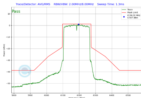
Plot 7-312 In-Band Emission Plot Antenna WF5B (160 MHz BW 802.11be(SU) (UNII Band 5) - Ch.47)
