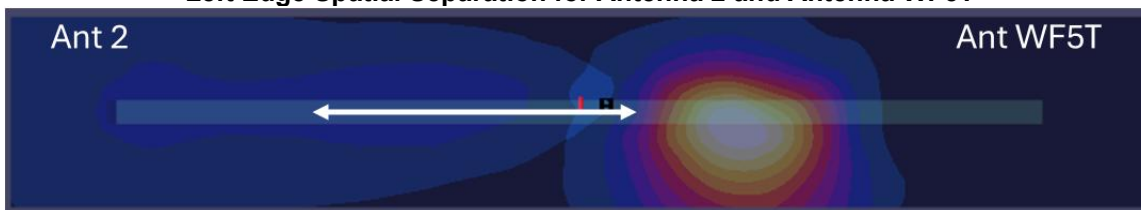
Figure F-46 Left Edge Spatial Separation for Antenna 2 and Antenna WF5T
