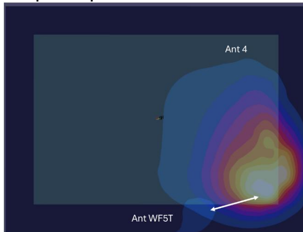
Figure F-19 Back Side Spatial Separation for Antenna 4 and Antenna WF5T
