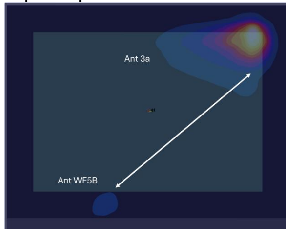
Figure F-16 Back Side Spatial Separation for Antenna 3a and Antenna WF5B
