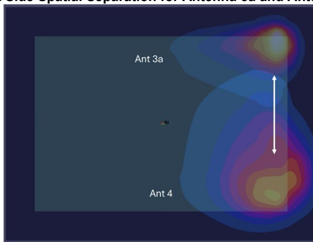
Figure F-14 Back Side Spatial Separation for Antenna 3a and Antenna 4
