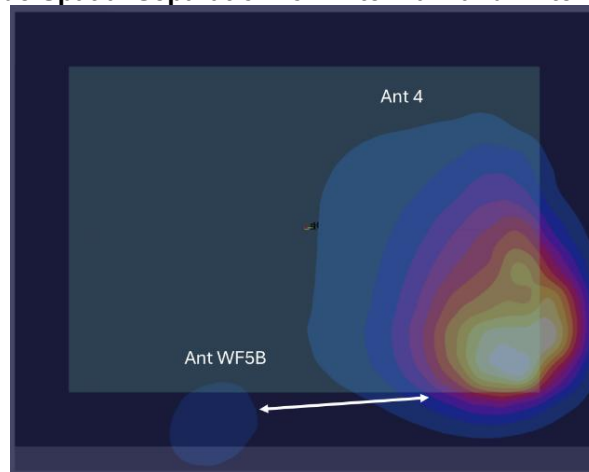
Figure F-20 Back Side Spatial Separation for Antenna 4 and Antenna WF5B
