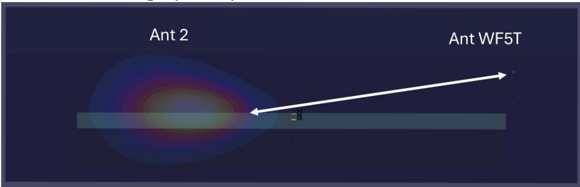
Figure F-26 Bottom Edge Spatial Separation for Antenna 2 and Antenna WF5T
