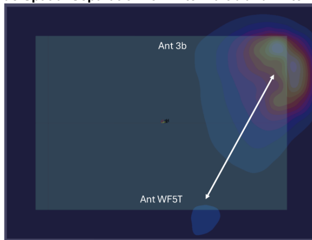
Figure F-17 Back Side Spatial Separation for Antenna 3b and Antenna WF5T
