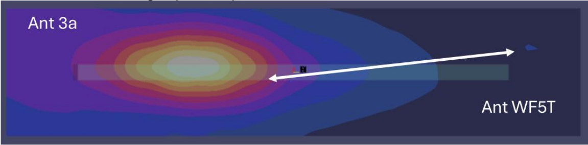
Figure F-27 Bottom Edge Spatial Separation for Antenna 3a and Antenna WF5T
