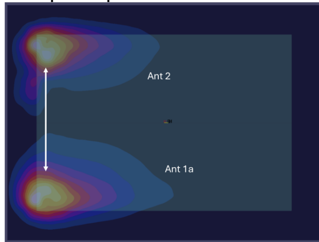
Back Side Spatial Separation for Antenna 1a and Antenna 2
