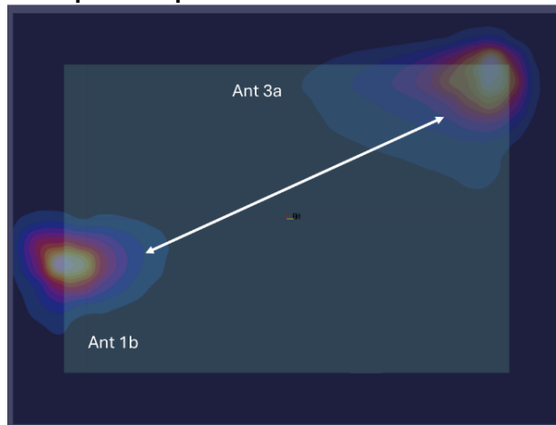
Figure F-7 Back Side Spatial Separation for Antenna 1b and Antenna 3a
