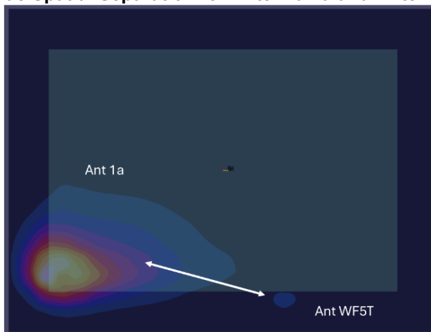
Figure F-5 Back Side Spatial Separation for Antenna 1a and Antenna WF5T
