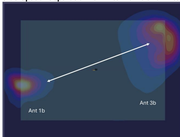
Figure F-8 Back Side Spatial Separation for Antenna 1b and Antenna 3b
