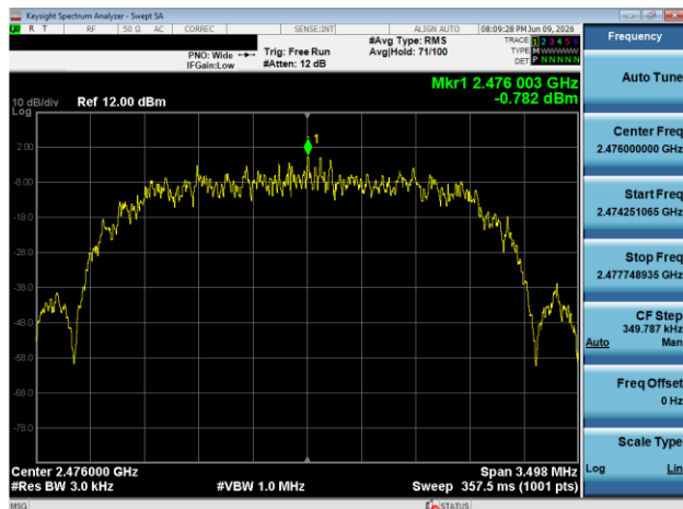
Plot 7-63. Power Spectral Density Plot Antenna 3A (Bluetooth (HDR4), 4Mbps, ePA - Ch. 73)
