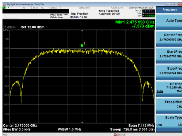
Plot 7-111. Power Spectral Density Plot Antenna 1A (Bluetooth (XHDRPM6), 6Mbps, ePA - Ch. 73)
