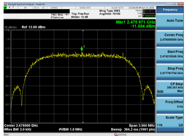
Plot 7-108. Power Spectral Density Plot Antenna 1A (Bluetooth (HDRPS2), 2Mbps, iPA – Ch. 73)
