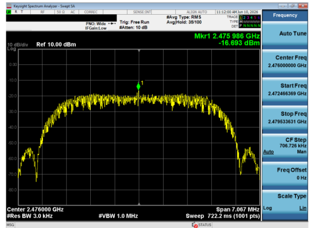
Plot 7-120. Power Spectral Density Plot Antenna 1A (Bluetooth (HDRPM16), 16Mbps, iPA – Ch. 73)
