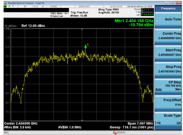
Plot 7-100. Power Spectral Density Plot Antenna 1A (Bluetooth (HDR8), 8Mbps, iPA – Ch. 1)
