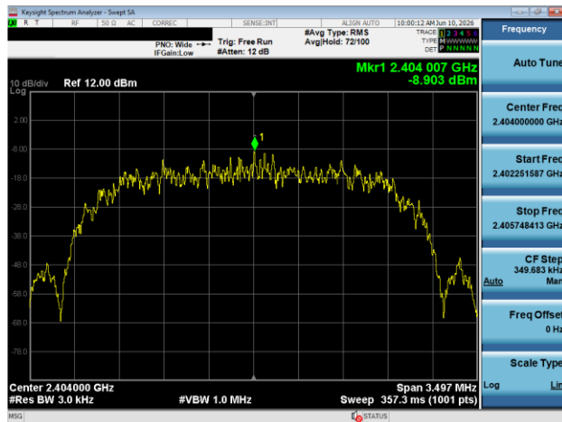
Plot 7-128. Power Spectral Density Plot Tx BF Antenna 1A (Bluetooth (HDR4), 4Mbps, iPA - Ch. 1)
