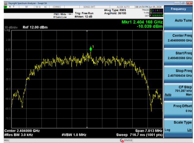
Plot 7-70. Power Spectral Density Plot Antenna 3A (Bluetooth) (HDR8), 8Mbps, iPA - Ch. 1)
