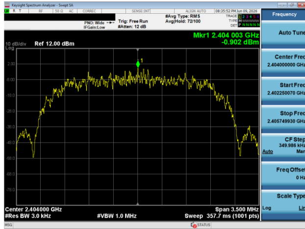
Plot 7-121. Power Spectral Density Plot TxBF Antenna 3A (Bluetooth (HDR4), 4Mbps, ePA - Ch. 1)
