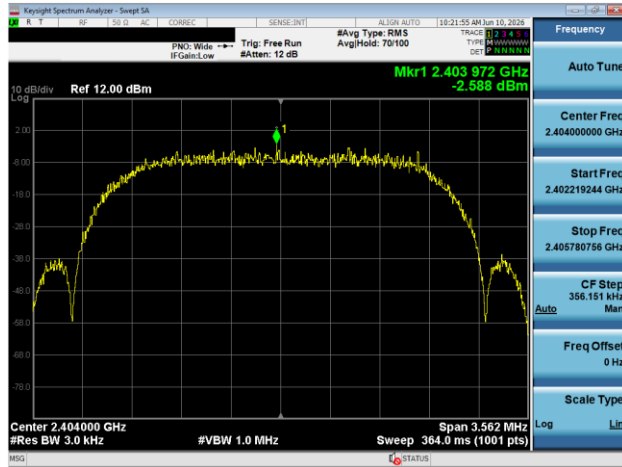
Plot 7-103. Power Spectral Density Plot Antenna 1A (Bluetooth (HDRPS2), 2Mbps, ePA – Ch. 1)
