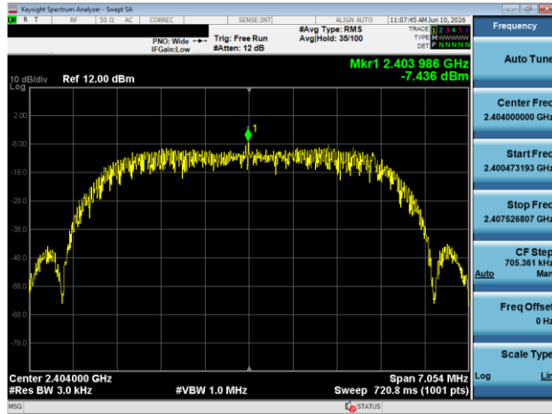
Plot 7-115. Power Spectral Density Plot Antenna 1A (Bluetooth (HDRPM16), 16Mbps, ePA – Ch. 1)
