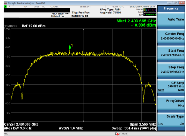
Plot 7-76. Power Spectral Density Plot Antenna 3A (Bluetooth (HDRPS2), 2Mbps, iPA – Ch. 1)
