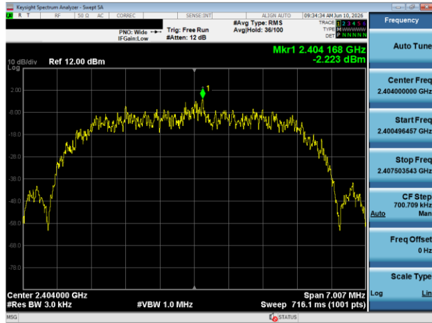
Plot 7-97. Power Spectral Density Plot Antenna 1A (Bluetooth (HDR8), 8Mbps, ePA – Ch. 1)
