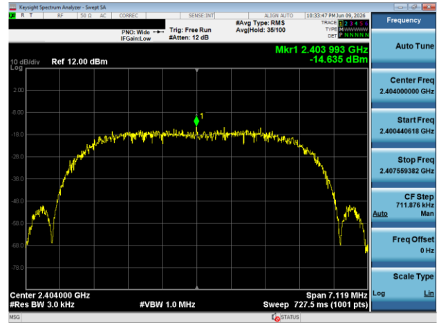
Plot 7-82. Power Spectral Density Plot Antenna 3A (Bluetooth (XHDRPM6), 6Mbps, iPA - Ch. 1)
