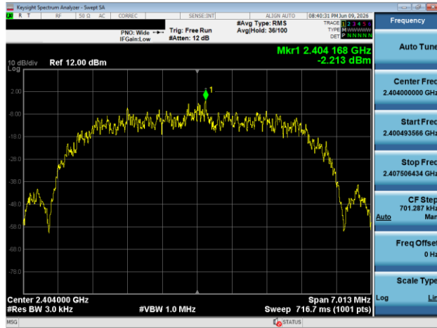
Plot 7-133. Power Spectral Density Plot TxBF Antenna 3A (Bluetooth (HDR8), 8Mbps, ePA - Ch. 1)
