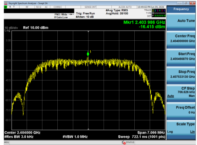
Plot 7-88. Power Spectral Density Plot Antenna 3A (Bluetooth (HDRPM16), 16Mbps, iPA – Ch. 1)
