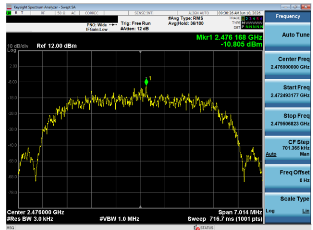
Plot 7-102. Power Spectral Density Plot Antenna 1A (Bluetooth (HDR8), 8Mbps, iPA – Ch. 73)
