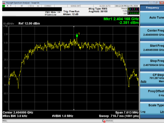
Plot 7-67. Power Spectral Density Plot Antenna 3A (Bluetooth) (HDR8), 8Mbps, ePA - Ch. 1)
