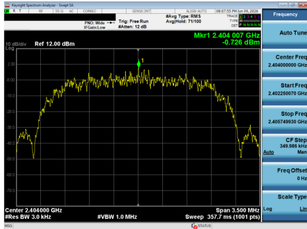
Plot 7-61. Power Spectral Density Plot Antenna 3A (Bluetooth (HDR), 4Mbps, ePA - Ch. 1)
