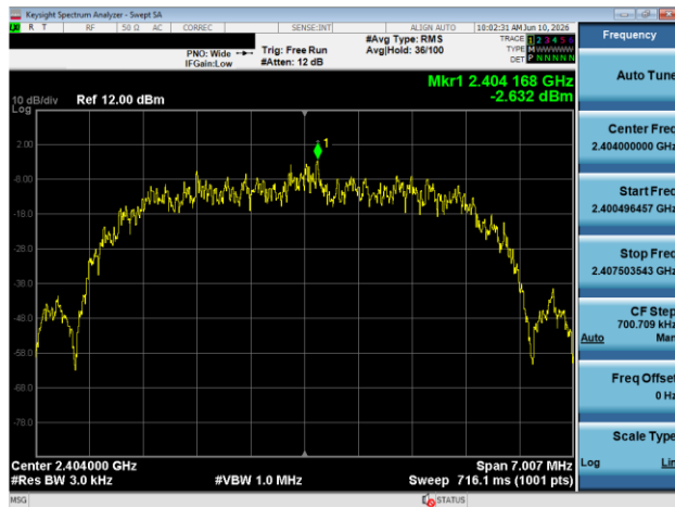
Plot 7-134. Power Spectral Density Plot TxBF Antenna 1A (Bluetooth (HDR8), 8Mbps, ePA - Ch. 1)
