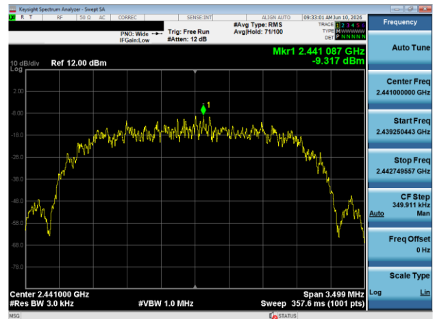
Plot 7-95. Power Spectral Density Plot Antenna 1A (Bluetooth (HDR4), 4Mbps, iPA – Ch. 38)
