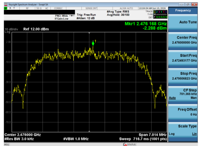
Plot 7-138. Power Spectral Density Plot TxBF Antenna 1A (Bluetooth (HDR8), 8Mbps, ePA - Ch. 73)
