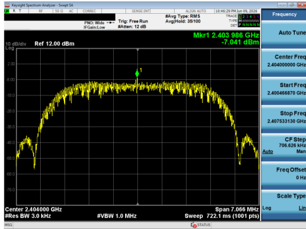
Plot 7-85. Power Spectral Density Plot Antenna 3A (Bluetooth (HDRPM16), 16Mbps, ePA – Ch. 1)
