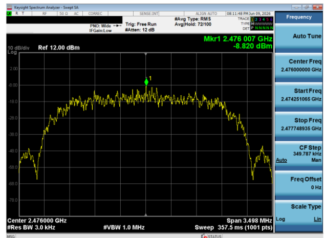
Plot 7-66. Power Spectral Density Plot Antenna 3A (Bluetooth (HDR4), 4Mbps, iPA - Ch. 73)
