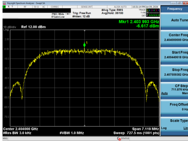
Plot 7-79. Power Spectral Density Plot Antenna 3A (Bluetooth (XHDRPM6), 6Mbps, ePA - Ch. 1)
