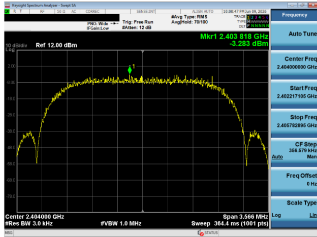
Plot 7-73. Power Spectral Density Plot Antenna 3A (Bluetooth (HDRPS2), 2Mbps, ePA – Ch. 1)
