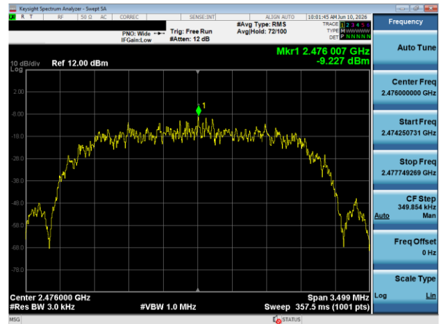
Plot 7-132. Power Spectral Density Plot Tx BF Antenna 1A (Bluetooth (HDR4), 4Mbps, iPA - Ch. 73)
