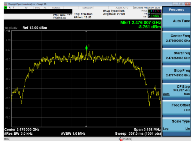
Plot 7-131. Power Spectral Density Plot Tx BF Antenna 3A (Bluetooth (HDR4), 4Mbps, iPA - Ch. 73)
