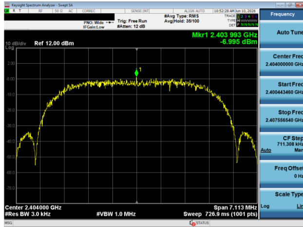
Plot 7-109. Power Spectral Density Plot Antenna 1A (Bluetooth (XHDRPM6), 6Mbps, ePA - Ch. 1)
