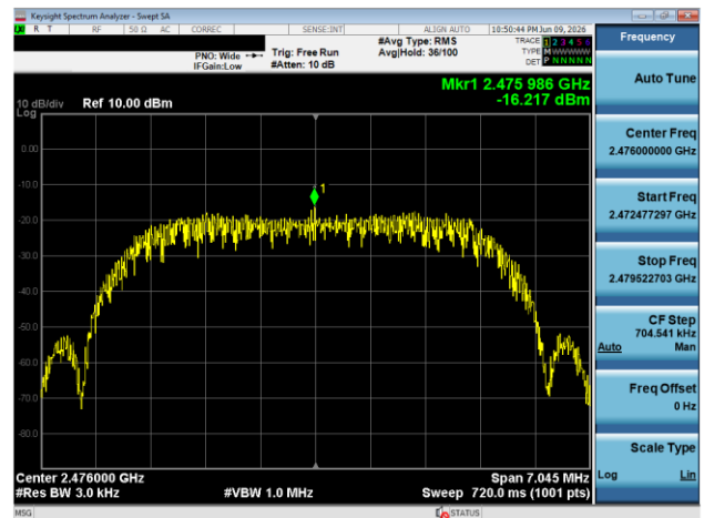
Plot 7-90. Power Spectral Density Plot Antenna 3A (Bluetooth (HDRPM16), 16Mbps, iPA – Ch. 73)
