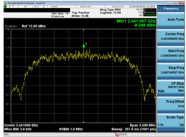
Plot 7-130. Power Spectral Density Plot Tx BF Antenna 1A (Bluetooth (HDR4), 4Mbps, iPA - Ch. 38)
