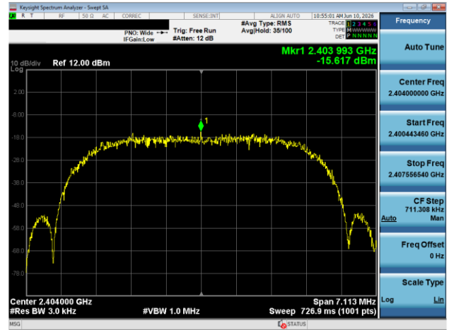
Plot 7-112. Power Spectral Density Plot Antenna 1A (Bluetooth (XHDRPM6), 6Mbps, iPA - Ch. 1)
