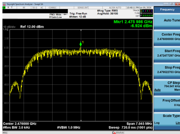
Plot 7-87. Power Spectral Density Plot Antenna 3A (Bluetooth (HDRPM16), 16Mbps, ePA – Ch. 73)
