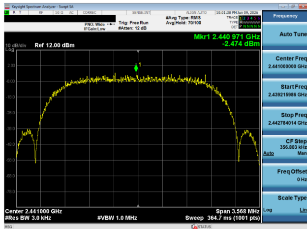
Plot 7-74. Power Spectral Density Plot Antenna 3A (Bluetooth (HDRPS2), 2Mbps, ePA – Ch. 38)
