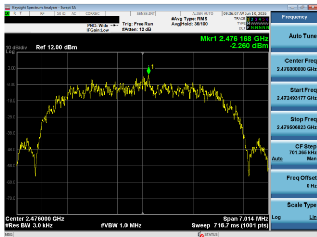
Plot 7-99. Power Spectral Density Plot Antenna 1A (Bluetooth (HDR8), 8Mbps, ePA – Ch. 73)
