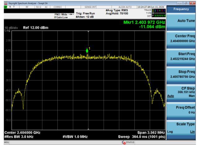
Plot 7-106. Power Spectral Density Plot Antenna 1A (Bluetooth (HDRPS2), 2Mbps, iPA – Ch. 1)
