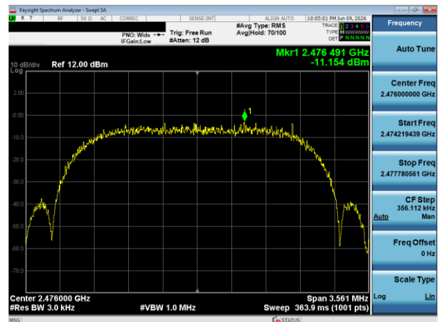
Plot 7-78. Power Spectral Density Plot Antenna 3A (Bluetooth (HDRPS2), 2Mbps, iPA – Ch. 73)
