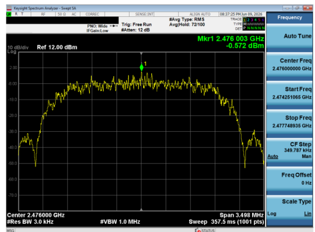
Plot 7-125. Power Spectral Density Plot TxBF Antenna 3A (Bluetooth (HDR4), 4Mbps, ePA - Ch. 73)
