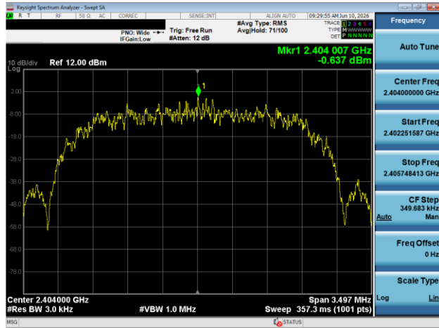
Plot 7-91. Power Spectral Density Plot Antenna 1A (Bluetooth (HDR4), 4Mbps, ePA – Ch. 1)
