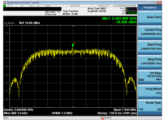
Plot 7-118. Power Spectral Density Plot Antenna 1A (Bluetooth (HDRPM16), 16Mbps, iPA – Ch. 1)
