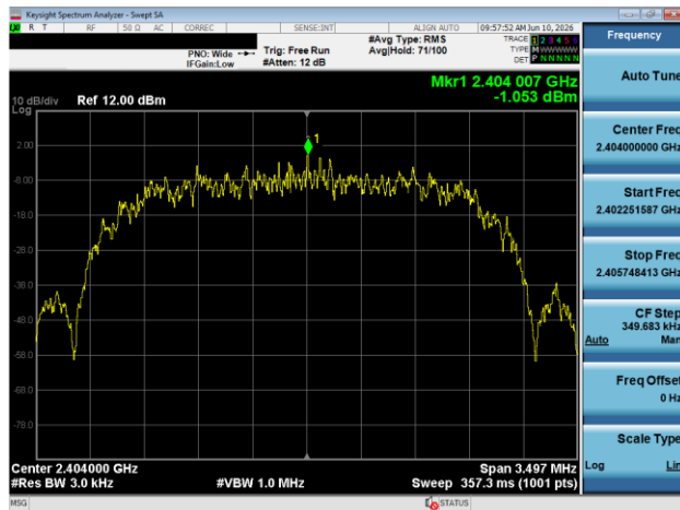
Plot 7-122. Power Spectral Density Plot TxBF Antenna 1A (Bluetooth (HDR4), 4Mbps, ePA - Ch. 1)
