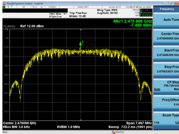
Plot 7-117. Power Spectral Density Plot Antenna 1A (Bluetooth (HDRPM16), 16Mbps, ePA – Ch. 73)
