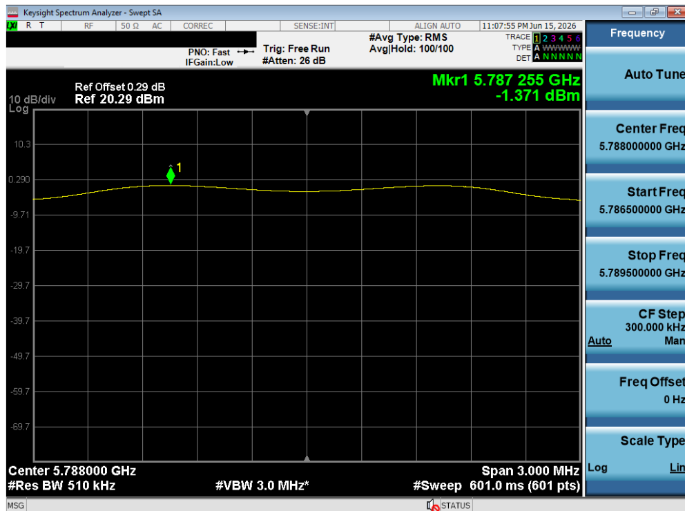
Plot 7-477. PSD TxBF Diversity Antenna 1B (NB UNII HDT4, iPA – 5788 MHz)
