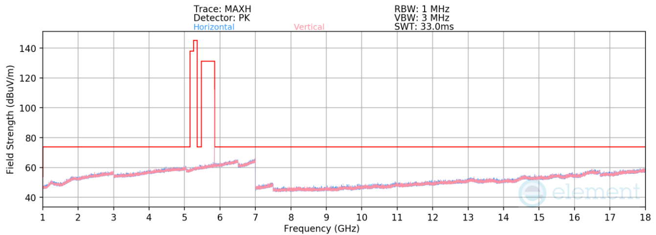
Plot 7-521. Radiated Spurious Emissions 1-18GHz TxBF Diversity (HDR4 ePA – 5844 MHz)
