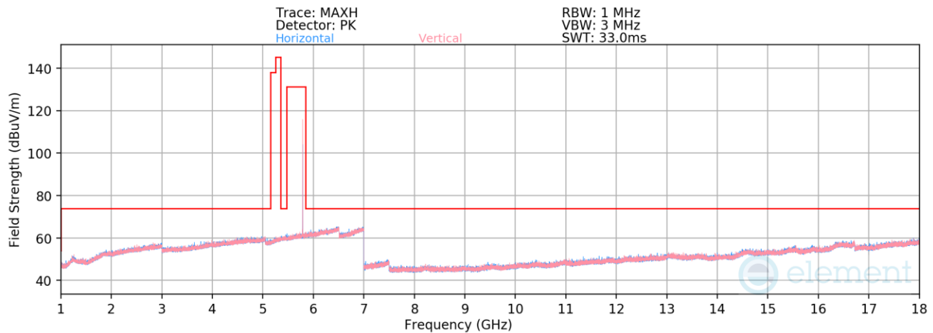
Plot 7-495. Radiated Spurious Emissions 1-18GHz TxBF Primary (HDR4 ePA – 5788 MHz)
