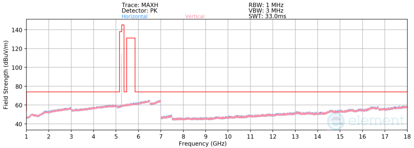
Plot 7-493. Radiated Spurious Emissions 1-18GHz TxBF Primary (HDR4 ePA – 5245 MHz)
