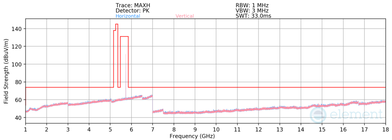
Plot 7-518. Radiated Spurious Emissions 1-18GHz TxBF Diversity (HDR4 ePA – 5733 MHz)
