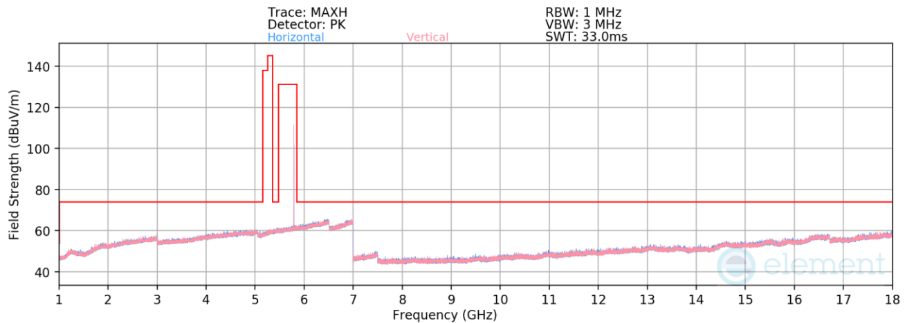
Plot 7-519. Radiated Spurious Emissions 1-18GHz TxBF Diversity (HDR4 ePA – 5788 MHz)
