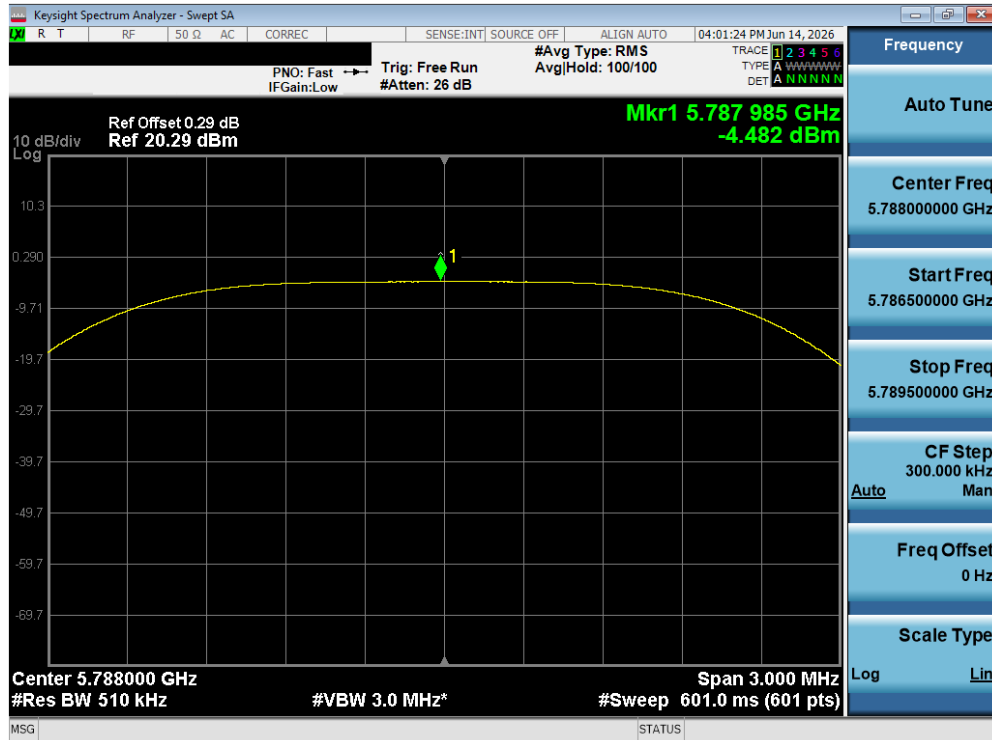
Plot 7-476. PSD TxBF Diversity Antenna 5T (NB UNII HDT4, iPA – 5788 MHz)
