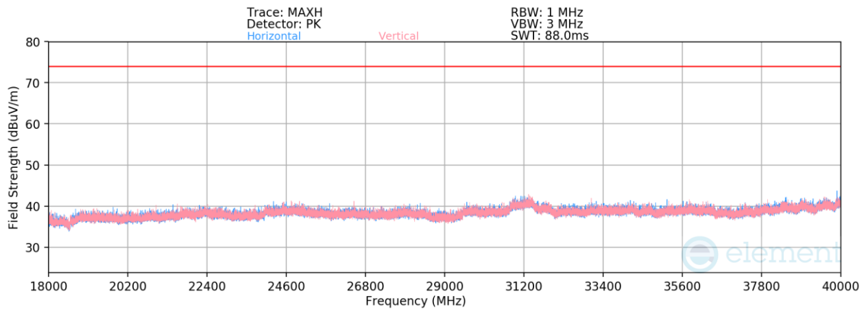
Plot 7-496. Radiated Spurious Emissions Above 18GHz (HDR4 ePA – 5788 MHz)
