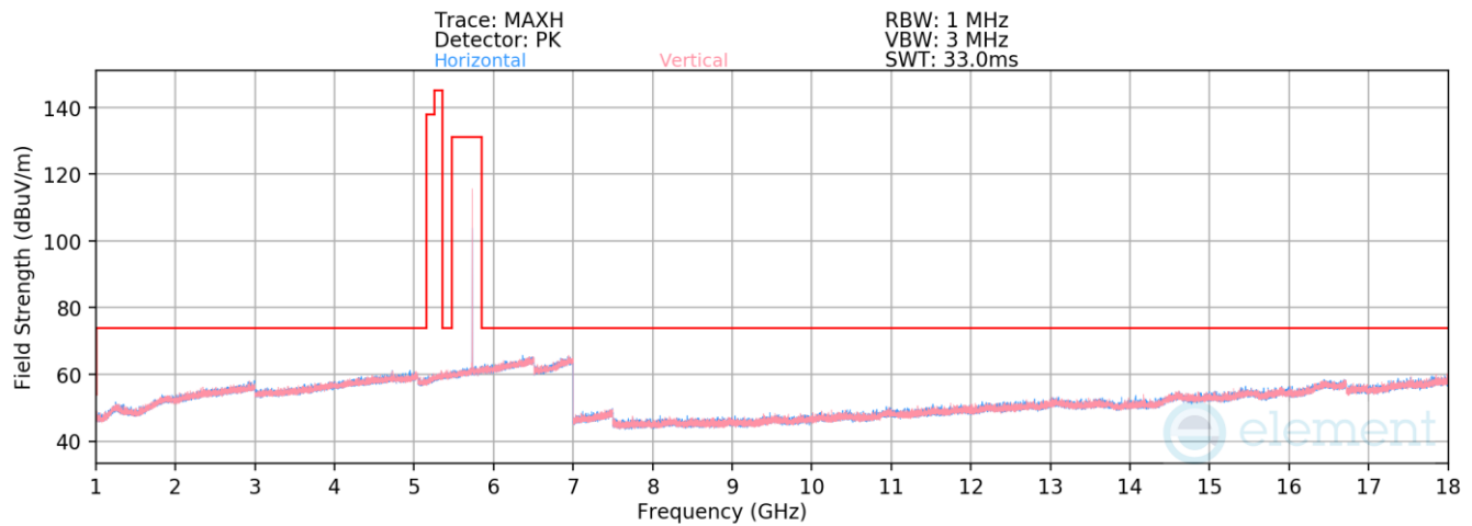
Plot 7-494. Radiated Spurious Emissions 1-18GHz TxBF Primary (HDR4 ePA – 5733 MHz)
