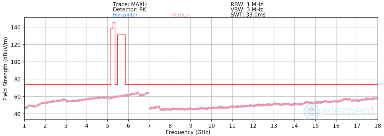
Plot 7-514. Radiated Spurious Emissions 1-18GHz TxBF Diversity (HDR4 ePA – 5162 MHz)
