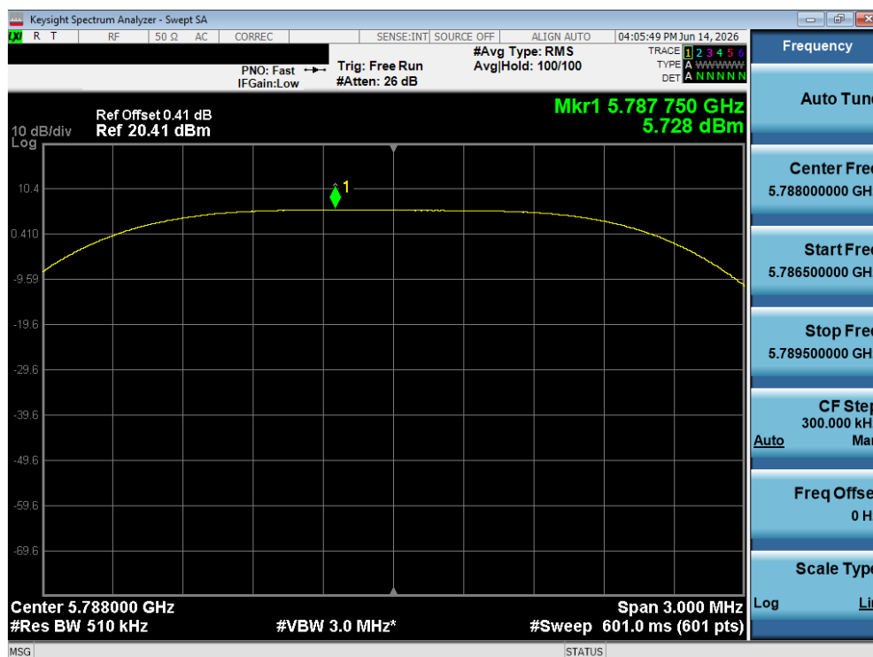
Plot 7-478. PSD TxBF Diversity Antenna 5T (NB UNII HDT6, ePA – 5788 MHz)
