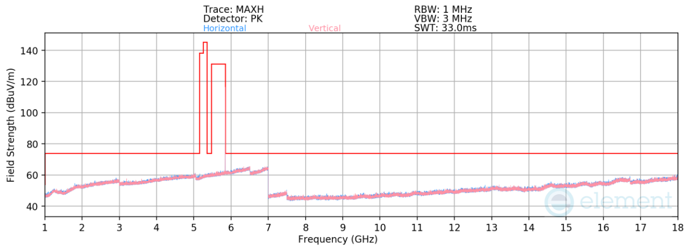
Plot 7-497. Radiated Spurious Emissions 1-18GHz TxBF Primary (HDR4 ePA – 5844 MHz)
