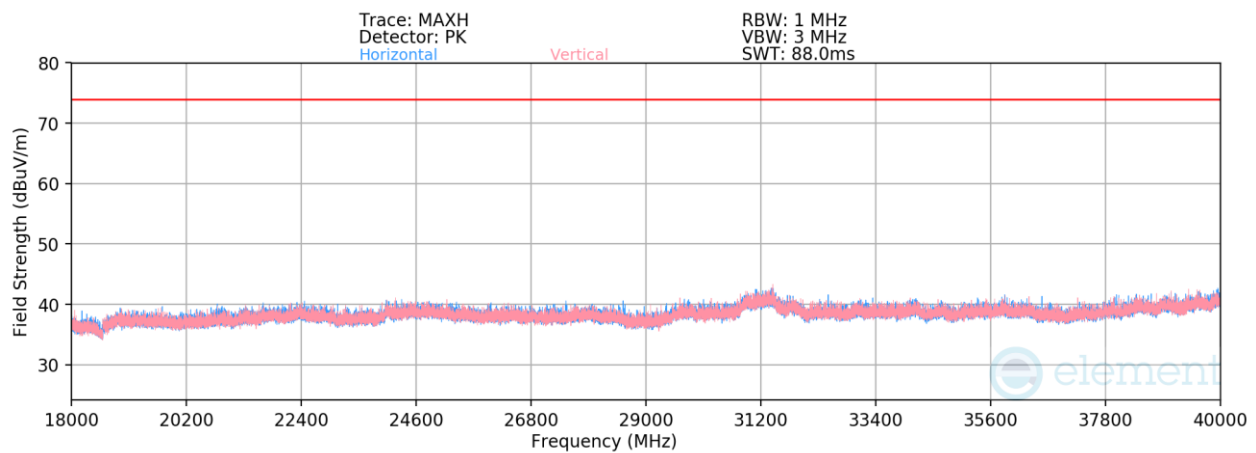
Plot 7-516. Radiated Spurious Emissions Above 18GHz (HDR4 ePA – 5203 MHz)
