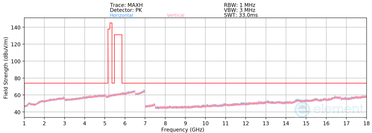
Plot 7-491. Radiated Spurious Emissions 1-18GHz TxBF Primary (HDR4 ePA – 5203 MHz)
