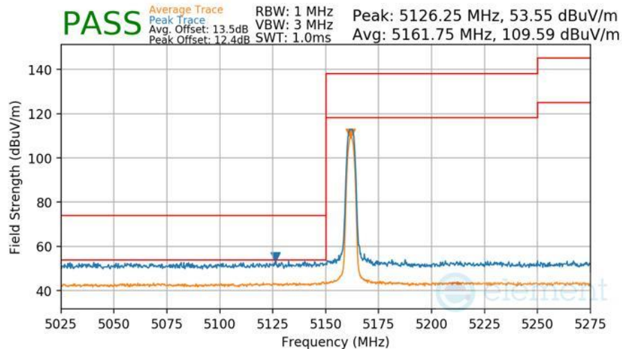
Plot 7-533 Radiated Lower Band Edge Measurement Antenna 5T
