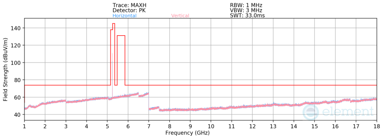
Plot 7-517. Radiated Spurious Emissions 1-18GHz TxBF Diversity (HDR4 ePA – 5245 MHz)
