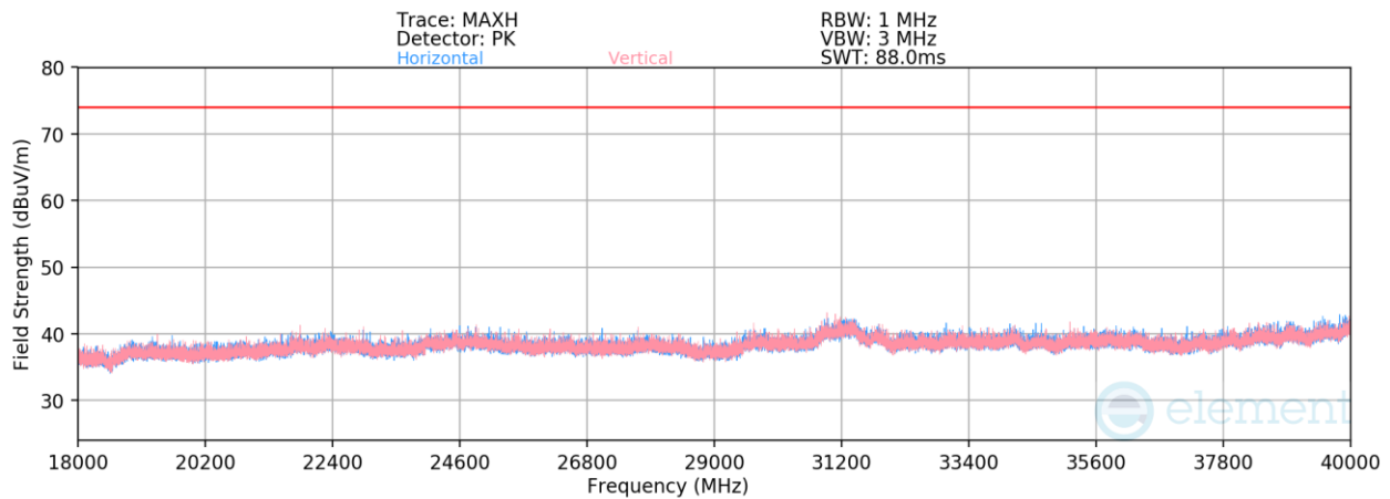
Plot 7-500. Radiated Spurious Emissions Above 18GHz (LE1M ePA – 5203 MHz)
