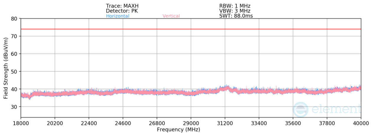
Plot 7-484. Radiated Spurious Emissions Above 18GHz (BDR GFSK ePA – 5203 MHz)
