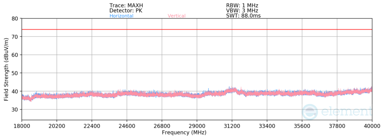
Plot 7-492. Radiated Spurious Emissions Above 18GHz (HDR4 ePA – 5203 MHz)
