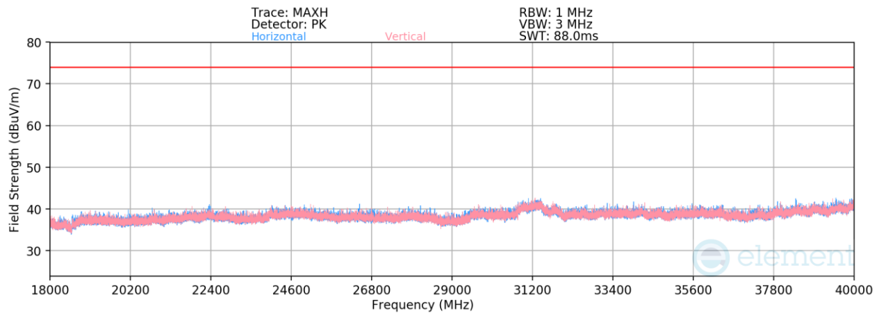
Plot 7-520. Radiated Spurious Emissions Above 18GHz (HDR4 ePA – 5788 MHz)
