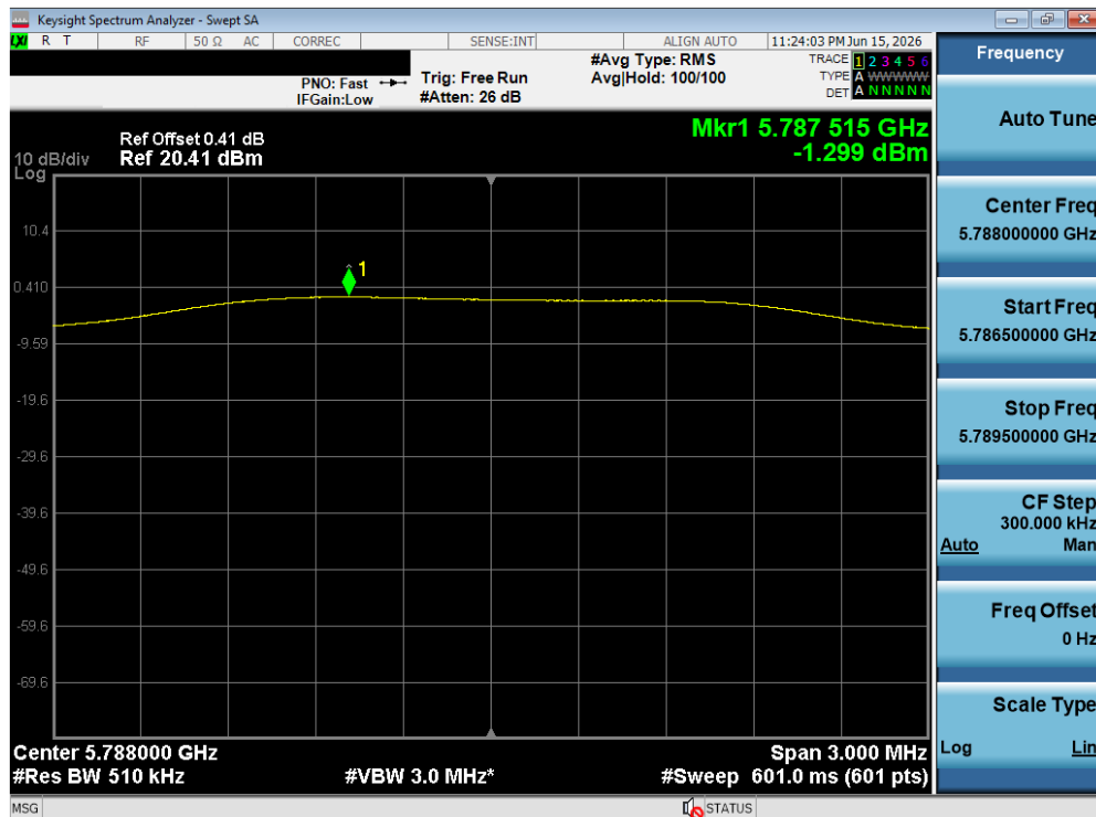
Plot 7-481. PSD TxBF Diversity Antenna 1B (NB UNII HDT6, iPA – 5788 MHz)
