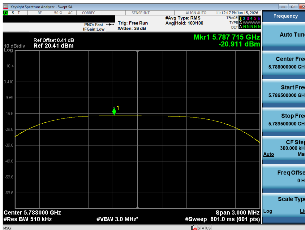
Plot 7-479. PSD TxBF Diversity Antenna 1B (NB UNII HDT6, ePA – 5788 MHz)
