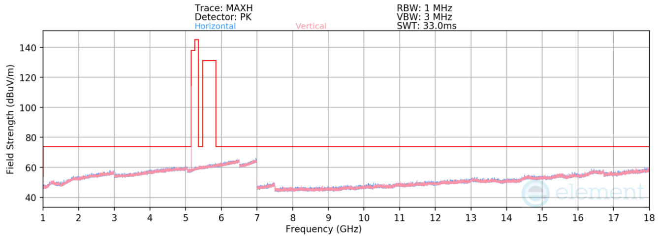
Plot 7-490. Radiated Spurious Emissions 1-18GHz TxBF Primary (HDR4 ePA – 5162 MHz)
