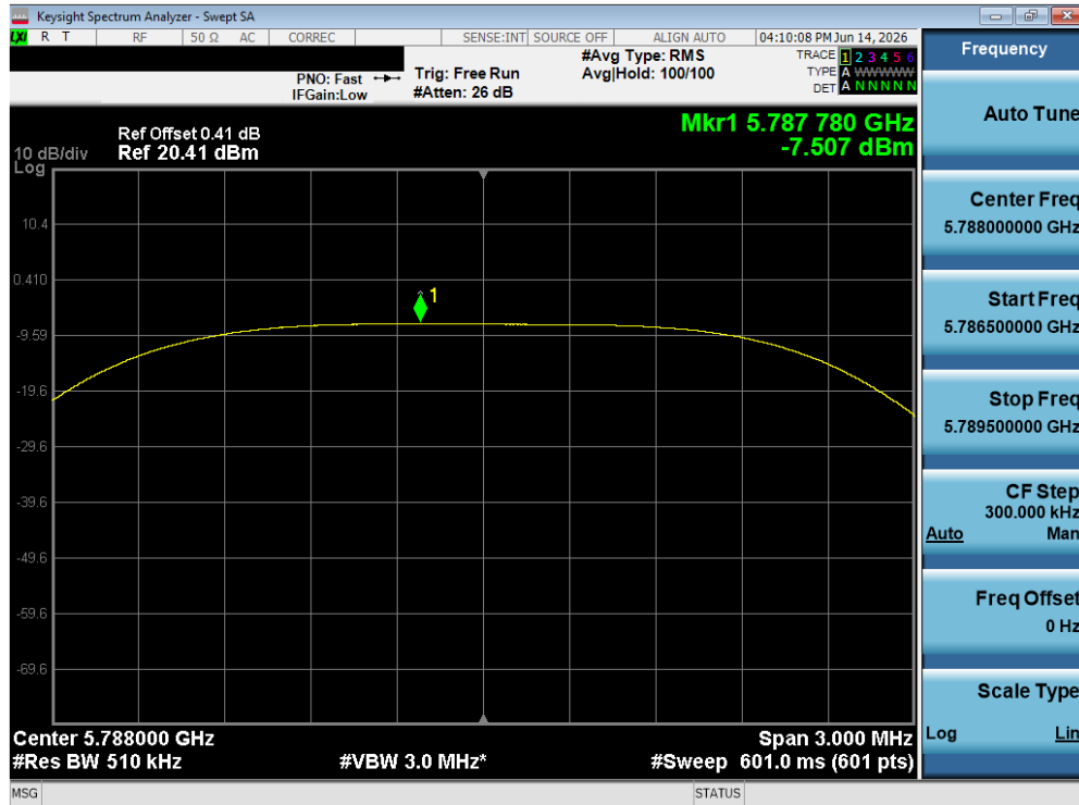
Plot 7-480. PSD TxBF Diversity Antenna 5T (NB UNII HDT6, iPA – 5788 MHz)
