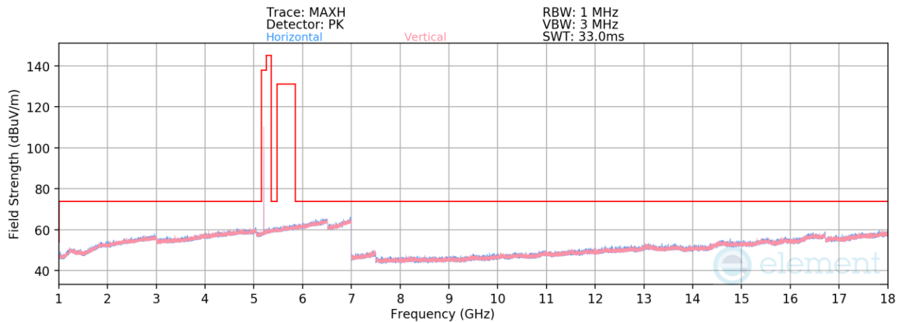
Plot 7-515. Radiated Spurious Emissions 1-18GHz TxBF Diversity (HDR4 ePA – 5203 MHz)
