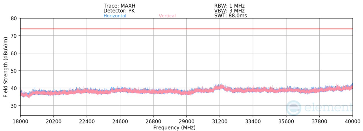
Plot 7-508. Radiated Spurious Emissions Above 18GHz (BDR GFSK ePA – 5203 MHz)
