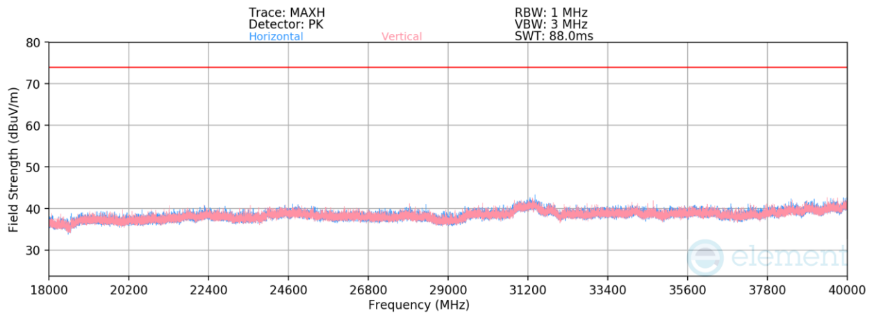
Plot 7-512. Radiated Spurious Emissions Above 18GHz (BDR GFSK ePA – 5788 MHz)
