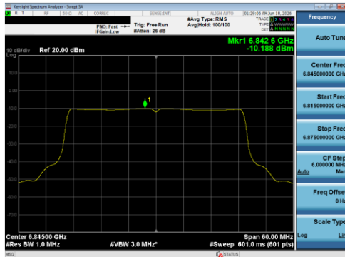
Plot 7-90 PSD Antenna 1B (40 MHz BW 802.11be(SU) - Ch.179)
