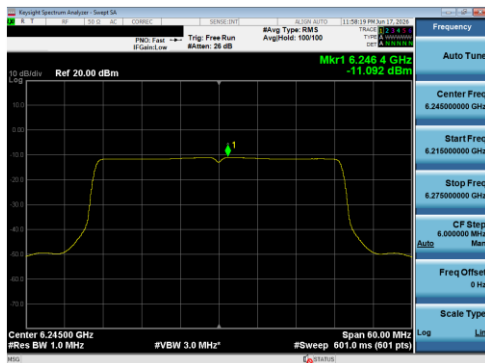
Plot 7-82 PSD Antenna 1B (40 MHz BW 802.11be(SU) - Ch.59)
