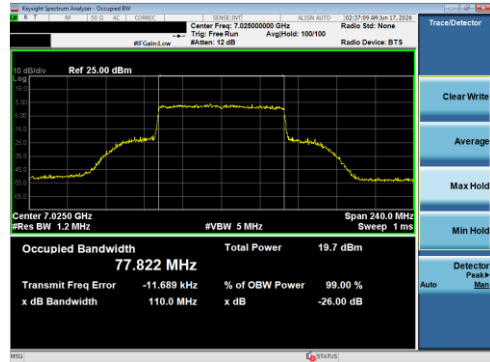
Plot 7-31 26 dB BW & 99% OBW Antenna 5B (80 MHz BW 802.11be(SU) - Ch.215)
