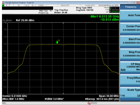
Plot 7-53 PSD Antenna 5T (20 MHz BW 802.11be(SU) - Ch.113)
