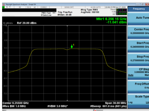
Plot 7-81 PSD Antenna 1B (20 MHz BW 802.11a - Ch.61)
