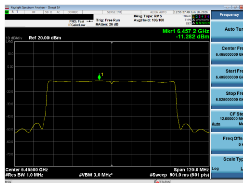
Plot 7-87 PSD Antenna 1B (80 MHz BW 802.11be(SU) - Ch.103)
