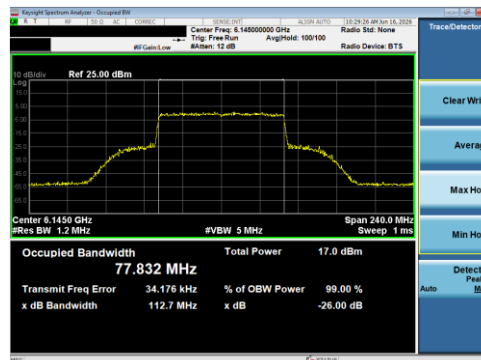
Plot 7-3 26 dB BW & 99% OBW Antenna 5T (80 MHz BW 802.11be(SU) - Ch.39)
