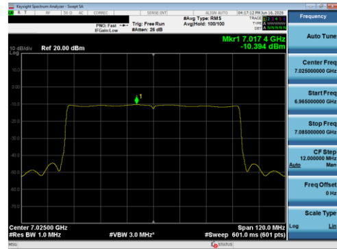
Plot 7-63 PSD Antenna 5T (80 MHz BW 802.11be(SU) - Ch.215)
