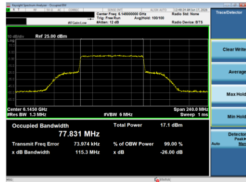
Plot 7-19 26 dB BW & 99% OBW Antenna 5B (80 MHz BW 802.11be(SU) - Ch.39)
