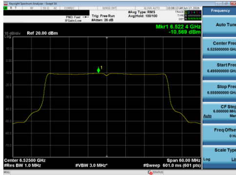
Plot 7-70 PSD Antenna 5B (40 MHz BW 802.11be(SU) - Ch.115)
