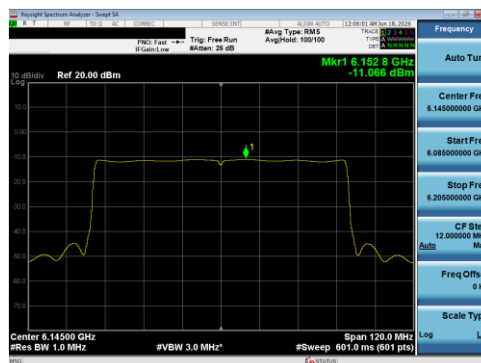
Plot 7-83 PSD Antenna 1B (80 MHz BW 802.11be(SU) - Ch.39)
