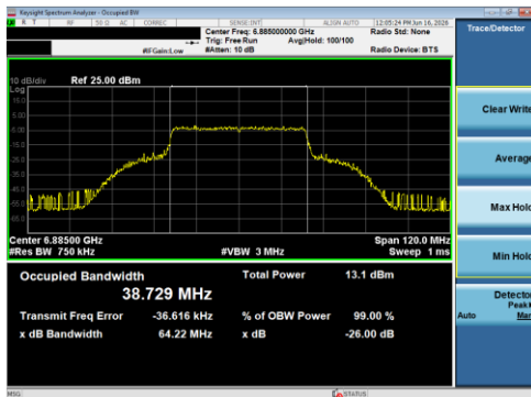
Plot 7-14 26 dB BW & 99% OBW Antenna 5T (40 MHz BW 802.11be(SU) - Ch.187)
