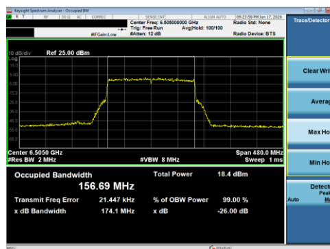
Plot 7-40 26 dB BW & 99% OBW Antenna 1B (160 MHz BW 802.11be(SU) - Ch.111)
