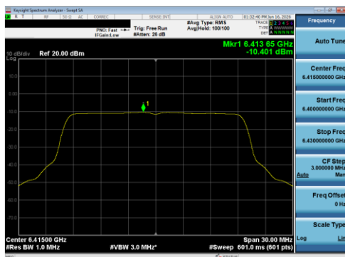
Plot 7-49 PSD Antenna 5T (20 MHz BW 802.11be(SU) - Ch.93)
