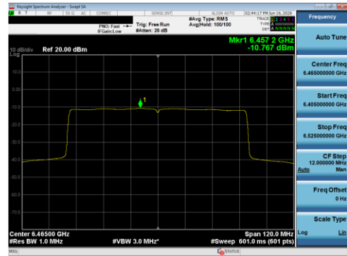
Plot 7-55 PSD Antenna 5T (80 MHz BW 802.11be(SU) - Ch.103)
