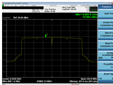
Plot 7-76 PSD Antenna 5B (160 MHz BW 802.11be(SU) - Ch.175)
