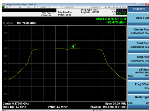
Plot 7-57 PSD Antenna 5T (20 MHz BW 802.11a - Ch.185)
