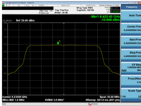
Plot 7-69 PSD Antenna 5B (20 MHz BW 802.11be(SU) - Ch.97)
