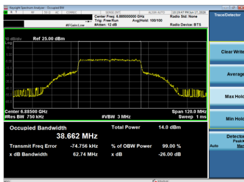
Plot 7-46 26 dB BW & 99% OBW Antenna 1B (40 MHz BW 802.11be(SU) - Ch.187)
