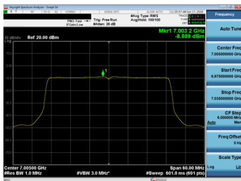
Plot 7-78 PSD Antenna 5B (40 MHz BW 802.11be(SU) - Ch.211)
