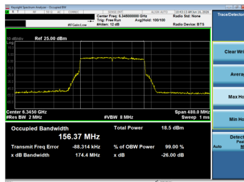
Plot 7-4 26 dB BW & 99% OBW Antenna 5T (160 MHz BW 802.11be(SU) - Ch.79)
