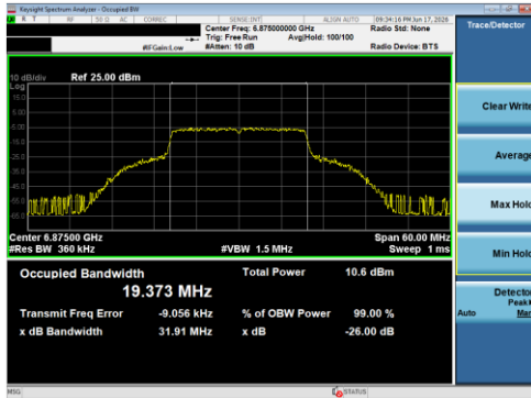
Plot 7-41 26 dB BW & 99% OBW Antenna 1B (20 MHz BW 802.11be(SU) - Ch.185)
