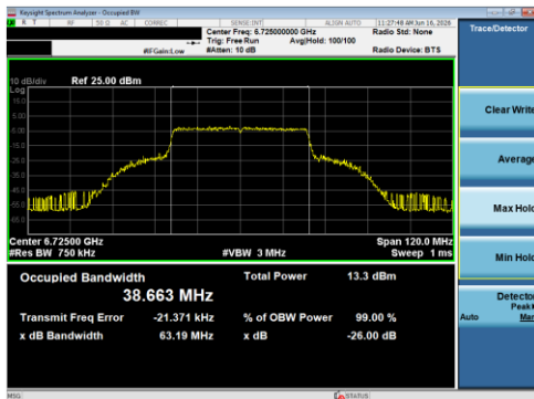
Plot 7-10 26 dB BW & 99% OBW Antenna 5T (40 MHz BW 802.11be(SU) - Ch.155)
