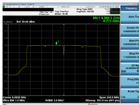
Plot 7-80 PSD Antenna 5B (160 MHz BW 802.11be(SU) - Ch.207)
