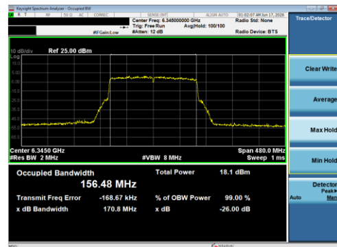
Plot 7-20 26 dB BW & 99% OBW Antenna 5B (160 MHz BW 802.11be(SU) - Ch.79)
