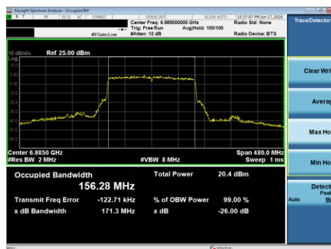
Plot 7-48 26 dB BW & 99% OBW Antenna 1B (160 MHz BW 802.11be(SU) - Ch.207)
