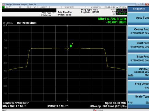
Plot 7-74 PSD Antenna 5B (40 MHz BW 802.11be(SU) - Ch.155)
