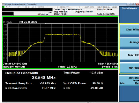
Plot 7-6 26 dB BW & 99% OBW Antenna 5T (40 MHz BW 802.11be(SU) - Ch.99)
