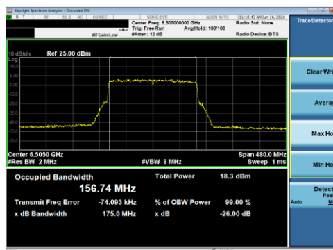
Plot 7-8 26 dB BW & 99% OBW Antenna 5T (160 MHz BW 802.11be(SU) - Ch.111)
