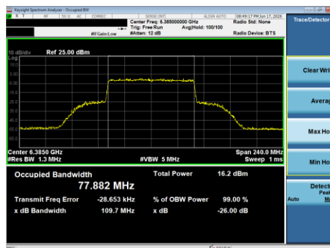
Plot 7-35 26 dB BW & 99% OBW Antenna 1B (80 MHz BW 802.11be(SU) - Ch.87)
