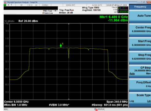
Plot 7-72 PSD Antenna 5B (160 MHz BW 802.11be(SU) - Ch.111)
