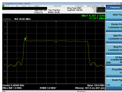
Plot 7-67 PSD Antenna 5B (80 MHz BW 802.11be(SU) - Ch.87)
