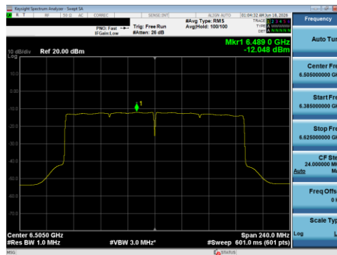
Plot 7-88 PSD Antenna 1B (160 MHz BW 802.11be(SU) - Ch.111)
