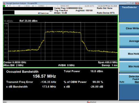
Plot 7-16 26 dB BW & 99% OBW Antenna 5T (160 MHz BW 802.11be(SU) - Ch.207)
