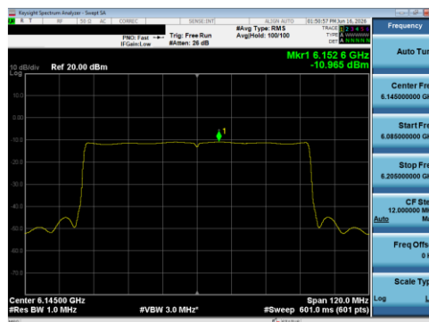
Plot 7-51 PSD Antenna 5T (80 MHz BW 802.11be(SU) - Ch.39)
