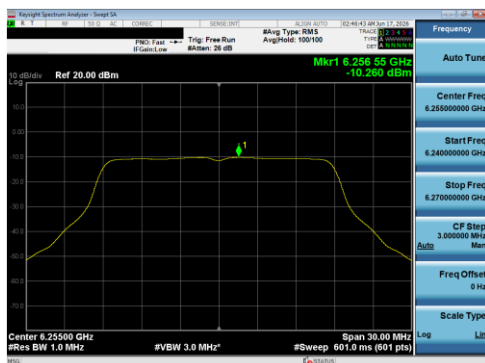
Plot 7-65 PSD Antenna 5B (20 MHz BW 802.11a - Ch.61)
