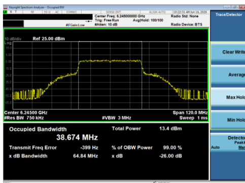
Plot 7-2 26 dB BW & 99% OBW Antenna 5T (40 MHz BW 802.11be(SU) - Ch.59)
