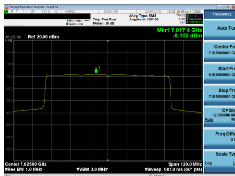
Plot 7-79 PSD Antenna 5B (80 MHz BW 802.11be(SU) - Ch.215)
