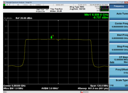
Plot 7-91 PSD Antenna 1B (80 MHz BW 802.11be(SU) - Ch.183)
