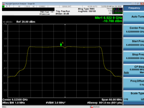
Plot 7-86 PSD Antenna 1B (40 MHz BW 802.11be(SU) - Ch.115)
