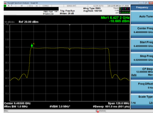
Plot 7-71 PSD Antenna 5B (80 MHz BW 802.11be(SU) - Ch.103)
