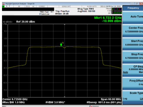
Plot 7-58 PSD Antenna 5T (40 MHz BW 802.11be(SU) - Ch.155)
