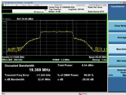
Plot 7-17 26 dB BW & 99% OBW Antenna 5B (20 MHz BW 802.11be(SU) - Ch.33)
