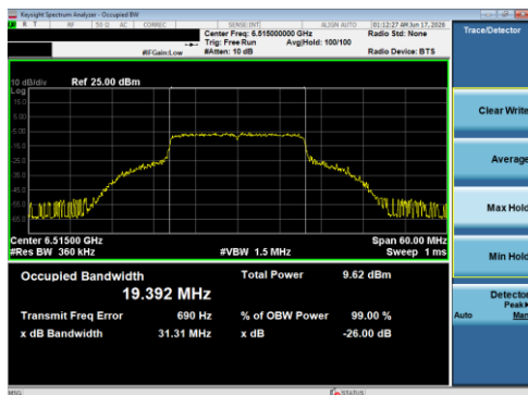
Plot 7-21 26 dB BW & 99% OBW Antenna 5B (20 MHz BW 802.11be(SU) - Ch.113)
