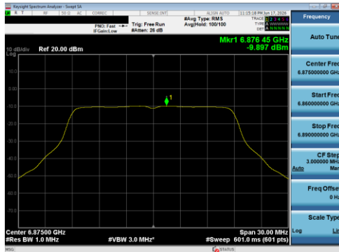
Plot 7-89 PSD Antenna 1B (20 MHz BW 802.11a - Ch.185)
