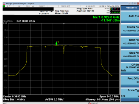
Plot 7-52 PSD Antenna 5T (160 MHz BW 802.11be(SU) - Ch.79)
