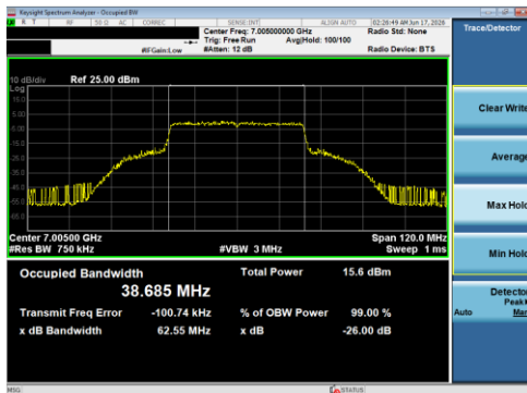
Plot 7-30 26 dB BW & 99% OBW Antenna 5B (40 MHz BW 802.11be(SU) - Ch.211)
