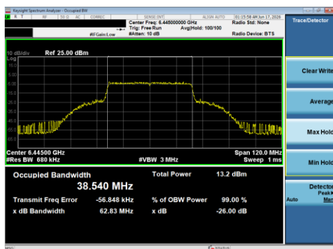
Plot 7-22 26 dB BW & 99% OBW Antenna 5B (40 MHz BW 802.11be(SU) - Ch.99)
