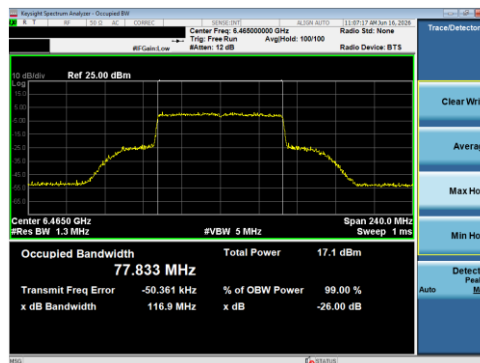
Plot 7-7 26 dB BW & 99% OBW Antenna 5T (80 MHz BW 802.11be(SU) - Ch.103)
