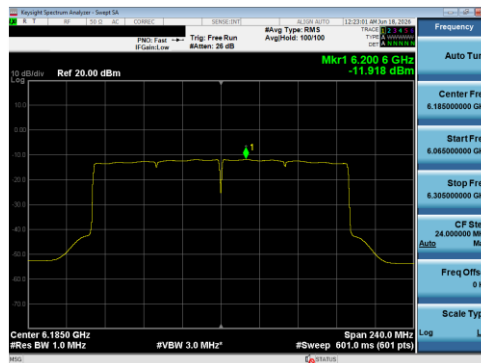
Plot 7-84 PSD Antenna 1B (160 MHz BW 802.11be(SU) - Ch.47)
