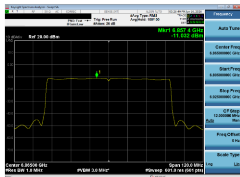
Plot 7-59 PSD Antenna 5T (80 MHz BW 802.11be(SU) - Ch.183)
