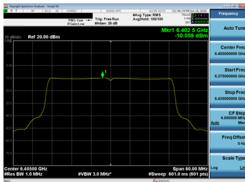
Plot 7-50 PSD Antenna 5T (40 MHz BW 802.11be(SU) - Ch.91)
