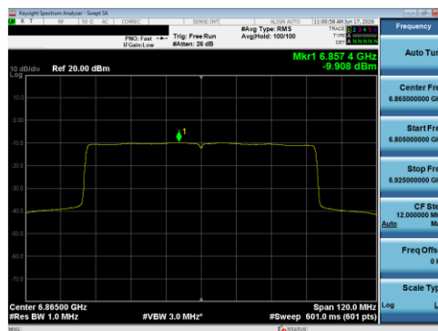
Plot 7-75 PSD Antenna 5B (80 MHz BW 802.11be(SU) - Ch.183)
