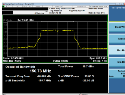
Plot 7-24 26 dB BW & 99% OBW Antenna 5B (160 MHz BW 802.11be(SU) - Ch.111)
