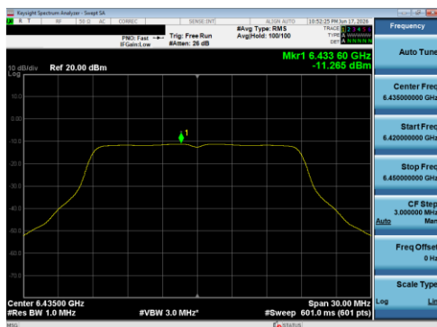
Plot 7-85 PSD Antenna 1B (20 MHz BW 802.11a - Ch.97)
