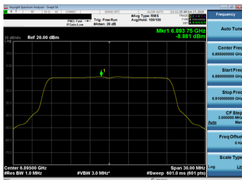
Plot 7-77 PSD Antenna 5B (20 MHz BW 802.11be(SU) - Ch.189)
