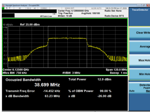
Plot 7-34 26 dB BW & 99% OBW Antenna 1B (40 MHz BW 802.11be(SU) - Ch.35)
