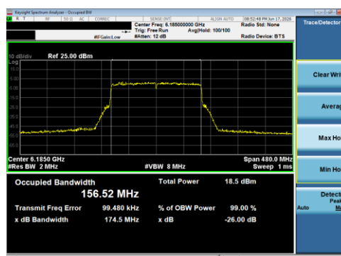
Plot 7-36 26 dB BW & 99% OBW Antenna 1B (160 MHz BW 802.11be(SU) - Ch.47)
