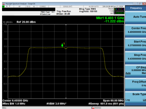
Plot 7-66 PSD Antenna 5B (40 MHz BW 802.11be(SU) - Ch.91)
