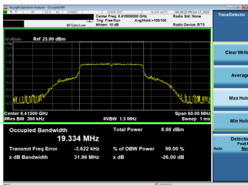
Plot 7-33 26 dB BW & 99% OBW Antenna 1B (20 MHz BW 802.11be(SU) - Ch.93)
