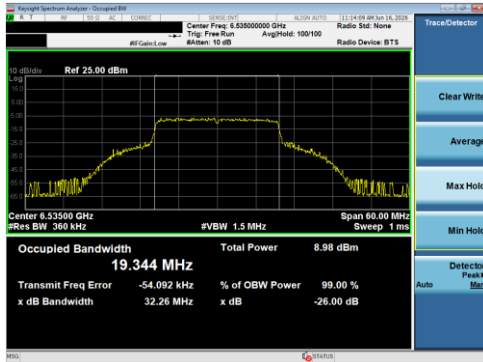
Plot 7-9 26 dB BW & 99% OBW Antenna 5T (20 MHz BW 802.11be(SU) - Ch.117)
