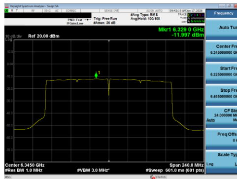
Plot 7-68 PSD Antenna 5B (160 MHz BW 802.11be(SU) - Ch.79)
