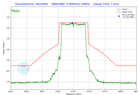
Plot 7-226 In-Band Emission Plot SDM Primary Antenna 5T (40 MHz BW 802.11be(SU) (UNII Band 7) - Ch.155)
