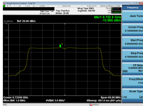
Plot 7-118 PSD SDM Primary Antenna 5B (40 MHz BW 802.11be(SU) - Ch.155)
