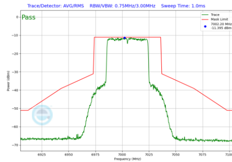
Plot 7-174 In-Band Emission Plot Antenna 5T (40 MHz BW 802.11be(SU) (UNII Band 8) - Ch.211)
