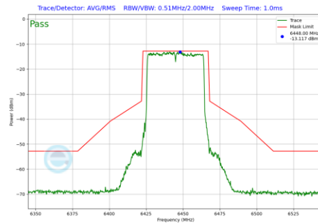
Plot 7-166 In-Band Emission Plot Antenna 5T (40 MHz BW 802.11be(SU) (UNII Band 6) - Ch.99)
