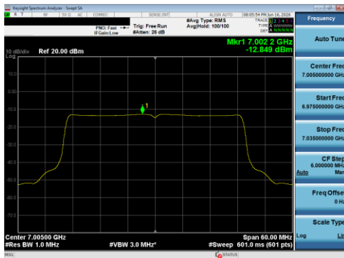
Plot 7-122 PSD SDM Primary Antenna 5T (40 MHz BW 802.11be(SU) - Ch.211)
