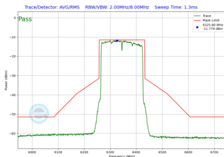
Plot 7-212 In-Band Emission Plot SDM Primary Antenna 5T (160 MHz BW 802.11be(SU) (UNII Band 5) - Ch.79)
