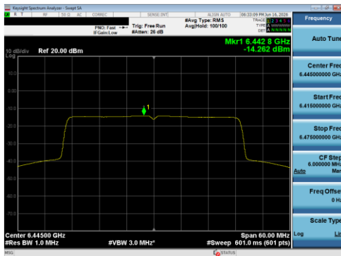
Plot 7-106 PSD SDM Primary Antenna 5T (40 MHz BW 802.11be(SU) - Ch.99)
