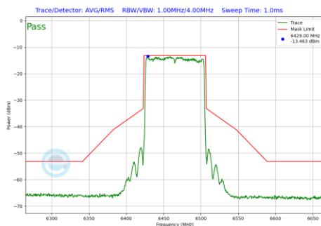
Plot 7-219 In-Band Emission Plot SDM Primary Antenna 5T (80 MHz BW 802.11be(SU) (UNII Band 6) - Ch.103)
