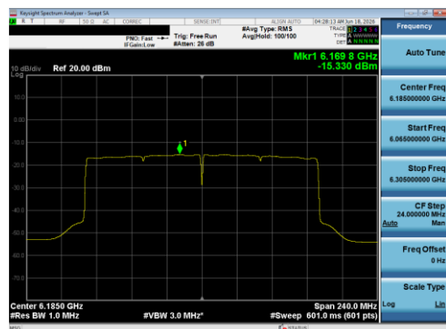
Plot 7-136 PSD CDD Diversity Antenna 1B (160 MHz BW 802.11be(SU) - Ch.47)
