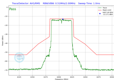
Plot 7-178 In-Band Emission Plot Antenna 5B (40 MHz BW 802.11be(SU) (UNII Band 5) - Ch.91)
