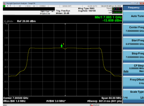
Plot 7-158 PSD CDD Diversity Antenna 1B (40 MHz BW 802.11be(SU) - Ch.211)
