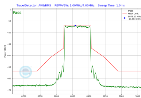
Plot 7-231 In-Band Emission Plot SDM Primary Antenna 5B (80 MHz BW 802.11be(SU) (UNII Band 7) - Ch.183)
