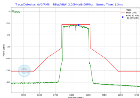
Plot 7-228 In-Band Emission Plot SDM Primary Antenna 5T (160 MHz BW 802.11be(SU) (UNII Band 7) - Ch.175)
