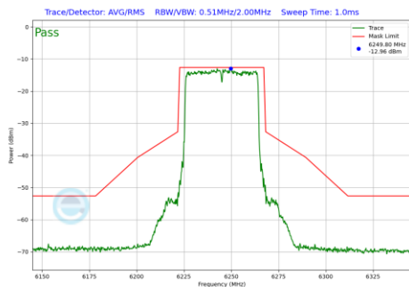
Plot 7-194 In-Band Emission Plot Antenna 1B (40 MHz BW 802.11be(SU) (UNII Band 5) - Ch.59)
