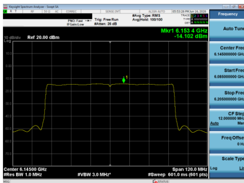
Plot 7-131 PSD CDD Diversity Antenna 5T (80 MHz BW 802.11be(SU) - Ch.39)
