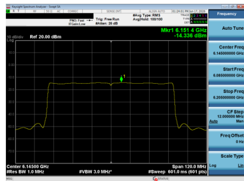
Plot 7-103 PSD SDM Primary Antenna 5B (80 MHz BW 802.11be(SU) - Ch.39)
