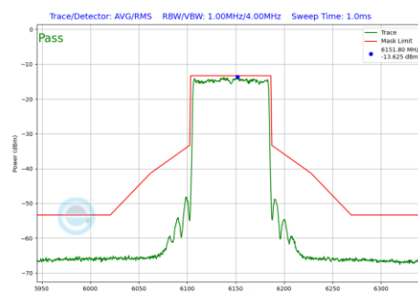
Plot 7-215 In-Band Emission Plot SDM Primary Antenna 5B (80 MHz BW 802.11be(SU) (UNII Band 5) - Ch.39)
