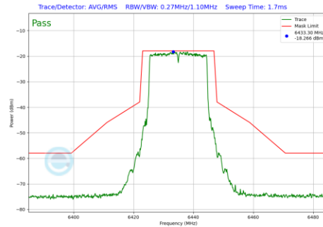
Plot 7-221 In-Band Emission Plot SDM Primary Antenna 5B (20 MHz BW 802.11be(SU) (UNII Band 6) - Ch.97)
