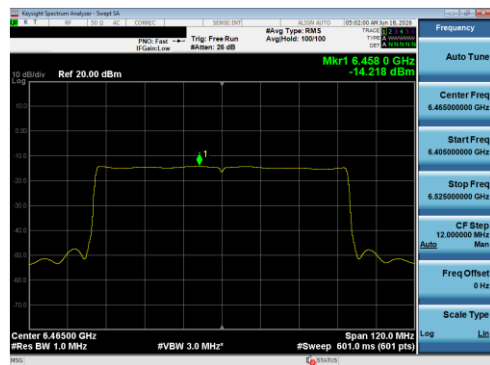
Plot 7-143 PSD CDD Diversity Antenna 1B (80 MHz BW 802.11be(SU) - Ch.103)
