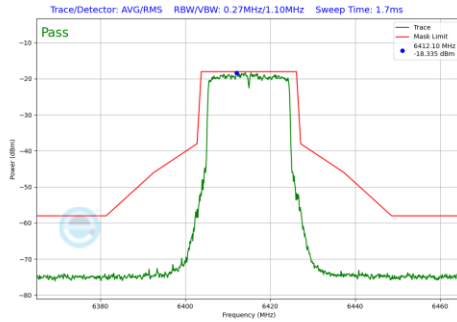
Plot 7-209 In-Band Emission Plot SDM Primary Antenna 5T (20 MHz BW 802.11be(SU) (UNII Band 5) - Ch.93)
