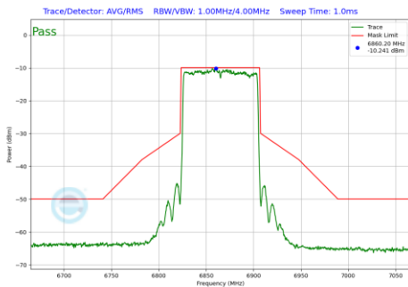
Plot 7-171 In-Band Emission Plot Antenna 5T (80 MHz BW 802.11be(SU) (UNII Band 7) - Ch.183)
