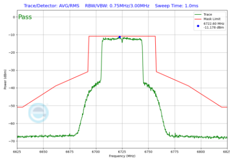
Plot 7-170 In-Band Emission Plot Antenna 5T (40 MHz BW 802.11be(SU) (UNII Band 7) - Ch.155)
