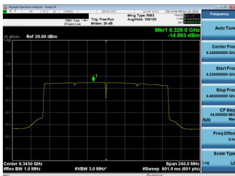
Plot 7-100 PSD SDM Primary Antenna 5T (160 MHz BW 802.11be(SU) - Ch.79)
