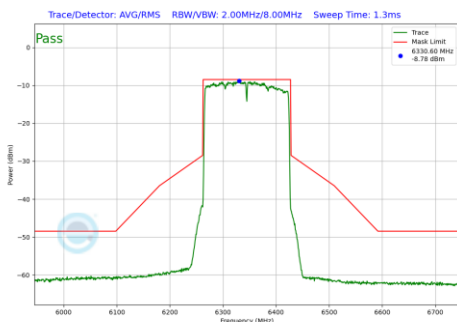
Plot 7-180 In-Band Emission Plot Antenna 5B (160 MHz BW 802.11be(SU) (UNII Band 5) - Ch.79)
