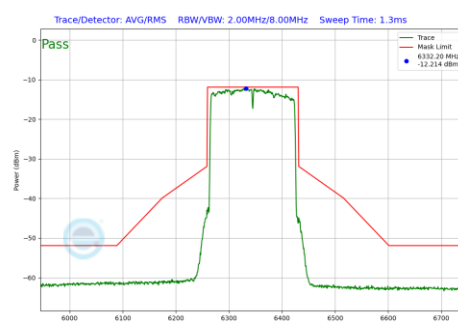
Plot 7-216 In-Band Emission Plot SDM Primary Antenna 5B (160 MHz BW 802.11be(SU) (UNII Band 5) - Ch.79)
