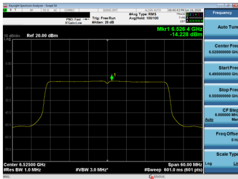
Plot 7-138 PSD CDD Diversity Antenna 5T (40 MHz BW 802.11be(SU) - Ch.115)
