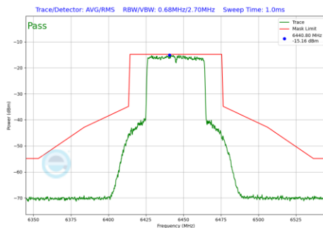
Plot 7-218 In-Band Emission Plot SDM Primary Antenna 5T (40 MHz BW 802.11be(SU) (UNII Band 6) - Ch.99)
