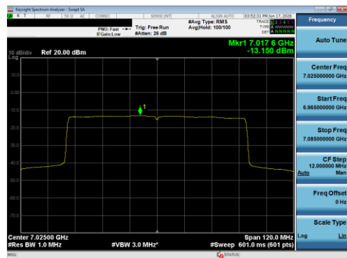
Plot 7-127 PSD SDM Primary Antenna 5B (80 MHz BW 802.11be(SU) - Ch.215)
