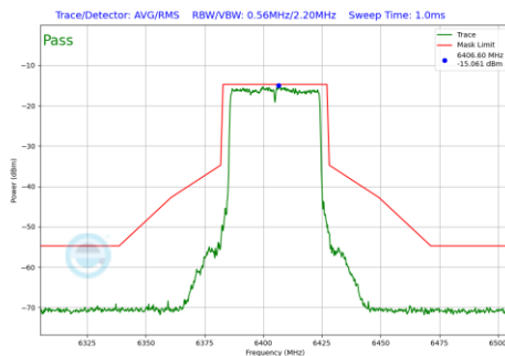
Plot 7-210 In-Band Emission Plot SDM Primary Antenna 5T (40 MHz BW 802.11be(SU) (UNII Band 5) - Ch.91)
