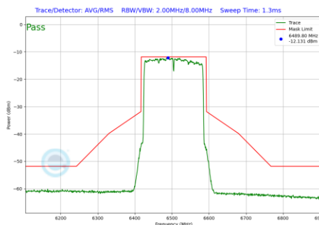
Plot 7-220 In-Band Emission Plot SDM Primary Antenna 5T (160 MHz BW 802.11be(SU) (UNII Band 6) - Ch.111)
