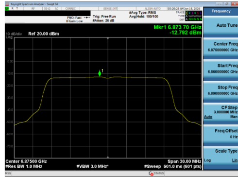
Plot 7-149 PSD CDD Diversity Antenna 1B (20 MHz BW 802.11be(SU) - Ch.185)
