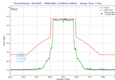
Plot 7-198 In-Band Emission Plot Antenna 1B (40 MHz BW 802.11be(SU) (UNII Band 6) - Ch.115)
