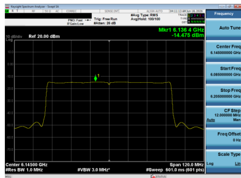
Plot 7-135 PSD CDD Diversity Antenna 1B (80 MHz BW 802.11be(SU) - Ch.39)
