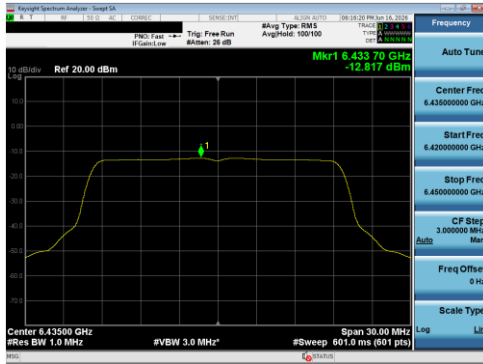
Plot 7-137 PSD CDD Diversity Antenna 5T (20 MHz BW 802.11be(SU) - Ch.97)
