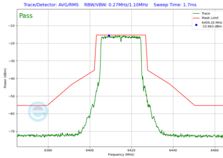
Plot 7-161 In-Band Emission Plot Antenna 5T (20 MHz BW 802.11be(SU) (UNII Band 5) - Ch.93)
