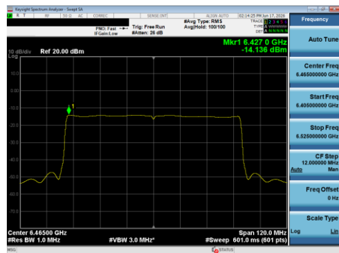
Plot 7-111 PSD SDM Primary Antenna 5B (80 MHz BW 802.11be(SU) - Ch.103)
