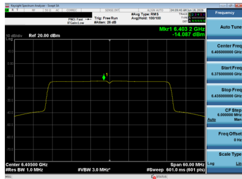
Plot 7-134 PSD CDD Diversity Antenna 1B (40 MHz BW 802.11be(SU) - Ch.91)
