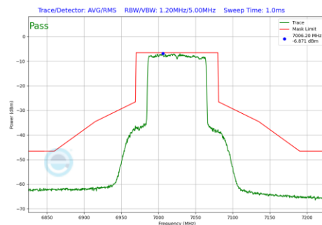
Plot 7-191 In-Band Emission Plot Antenna 5B (80 MHz BW 802.11be(SU) (UNII Band 8) - Ch.215)
