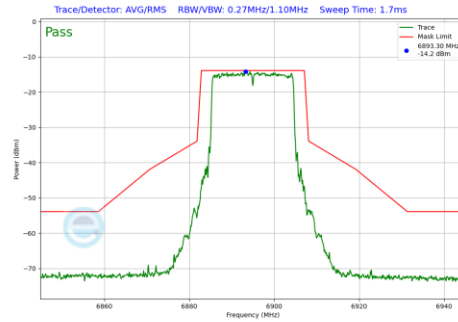
Plot 7-205 In-Band Emission Plot Antenna 1B (20 MHz BW 802.11be(SU) (UNII Band 8) - Ch.189)
