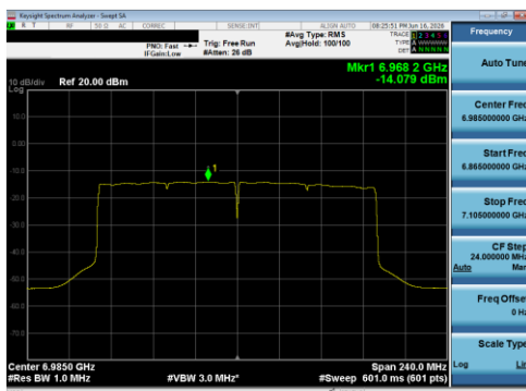
Plot 7-156 PSD CDD Diversity Antenna 5T (160 MHz BW 802.11be(SU) - Ch.207)
