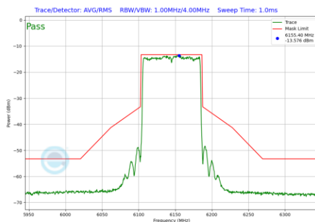
Plot 7-211 In-Band Emission Plot SDM Primary Antenna 5T (80 MHz BW 802.11be(SU) (UNII Band 5) - Ch.39)
