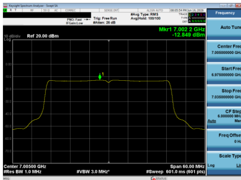
Plot 7-154 PSD CDD Diversity Antenna 5T (40 MHz BW 802.11be(SU) - Ch.211)
