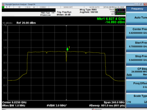
Plot 7-148 PSD CDD Diversity Antenna 5T (160 MHz BW 802.11be(SU) - Ch.175)
