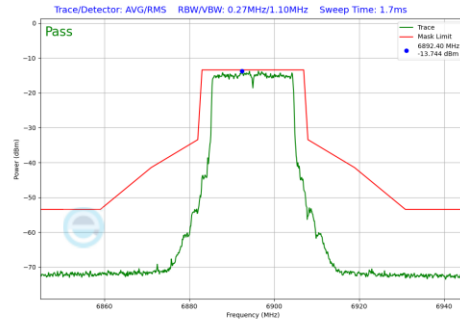
Plot 7-189 In-Band Emission Plot Antenna 5B (20 MHz BW 802.11be(SU) (UNII Band 8) - Ch.189)
