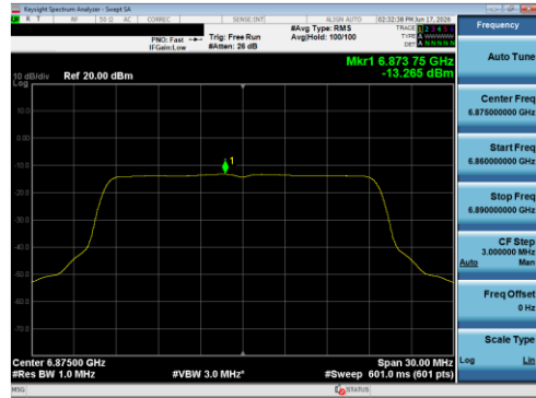
Plot 7-117 PSD SDM Primary Antenna 5B (20 MHz BW 802.11be(SU) - Ch.185)
