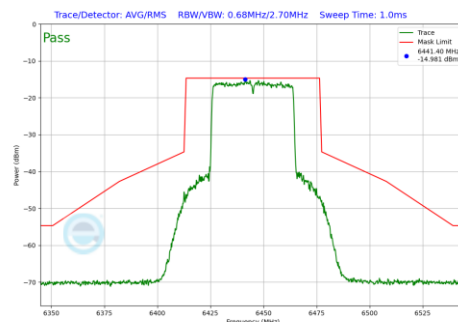
Plot 7-222 In-Band Emission Plot SDM Primary Antenna 5B (40 MHz BW 802.11be(SU) (UNII Band 6) - Ch.99)
