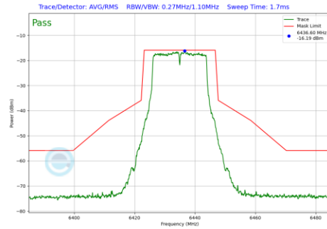
Plot 7-197 In-Band Emission Plot Antenna 1B (20 MHz BW 802.11a (UNII Band 6) - Ch.97)
