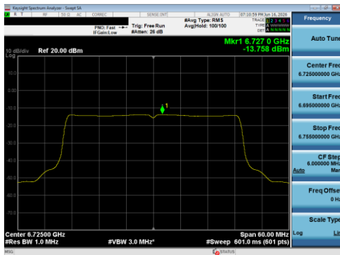
Plot 7-146 PSD CDD Diversity Antenna 5T (40 MHz BW 802.11be(SU) - Ch.155)
