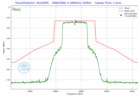
Plot 7-185 In-Band Emission Plot Antenna 5B (20 MHz BW 802.11be(SU) (UNII Band 7) - Ch.185)
