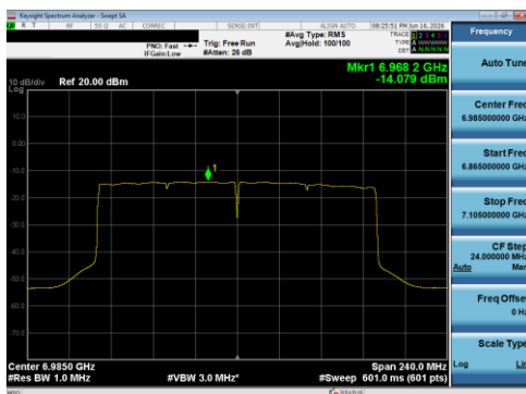
Plot 7-124 PSD SDM Primary Antenna 5T (160 MHz BW 802.11be(SU) - Ch.207)
