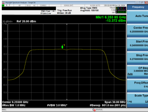
Plot 7-129 PSD CDD Diversity Antenna 5T (20 MHz BW 802.11be(SU) - Ch.61)
