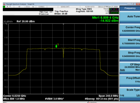
Plot 7-120 PSD SDM Primary Antenna 5B (160 MHz BW 802.11be(SU) - Ch.175)
