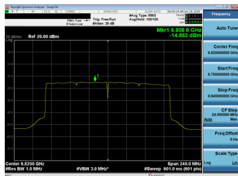
Plot 7-152 PSD CDD Diversity Antenna 1B (160 MHz BW 802.11be(SU) - Ch.175)
