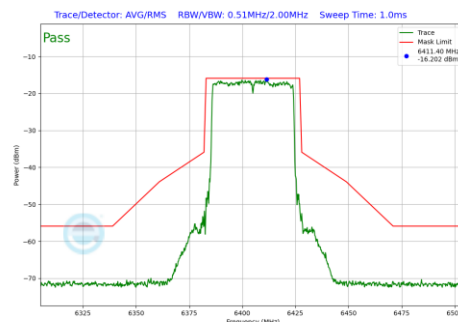
Plot 7-214 In-Band Emission Plot SDM Primary Antenna 5B (40 MHz BW 802.11be(SU) (UNII Band 5) - Ch.91)
