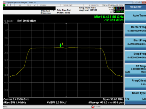
Plot 7-141 PSD CDD Diversity Antenna 1B (20 MHz BW 802.11be(SU) - Ch.97)
