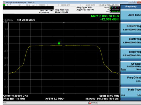
Plot 7-125 PSD SDM Primary Antenna 5B (20 MHz BW 802.11be(SU) - Ch.189)
