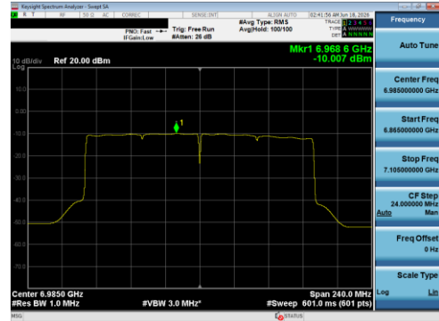
Plot 7-96 PSD Antenna 1B (160 MHz BW 802.11be(SU) - Ch.207)
