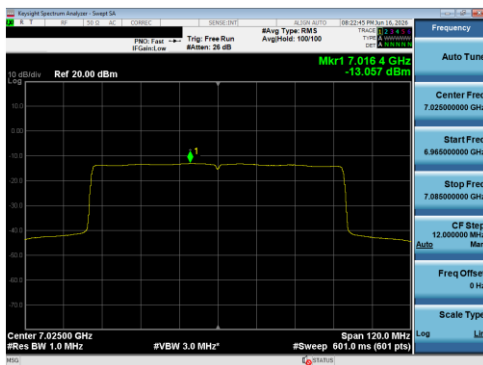
Plot 7-123 PSD SDM Primary Antenna 5T (80 MHz BW 802.11be(SU) - Ch.215)
