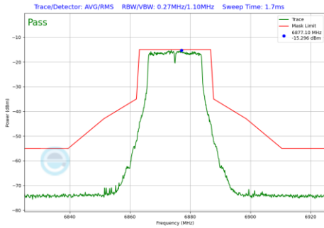
Plot 7-169 In-Band Emission Plot Antenna 5T (20 MHz BW 802.11a (UNII Band 7) - Ch.185)
