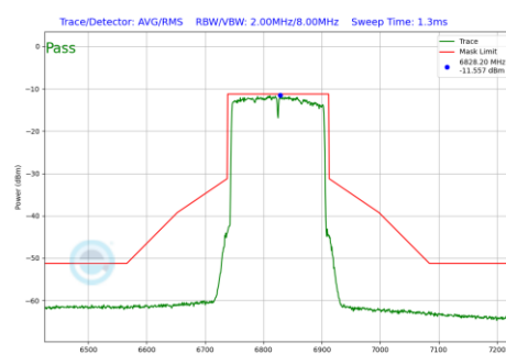
Plot 7-232 In-Band Emission Plot SDM Primary Antenna 5B (160 MHz BW 802.11be(SU) (UNII Band 7) - Ch.175)
