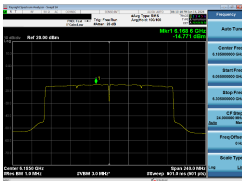
Plot 7-132 PSD CDD Diversity Antenna 5T (160 MHz BW 802.11be(SU) - Ch.47)
