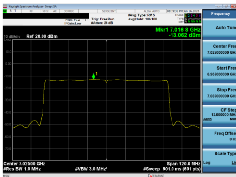
Plot 7-155 PSD CDD Diversity Antenna 5T (80 MHz BW 802.11be(SU) - Ch.215)
