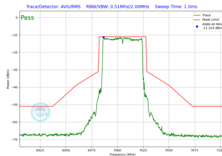
Plot 7-206 In-Band Emission Plot Antenna 1B (40 MHz BW 802.11be(SU) (UNII Band 8) - Ch.211)
