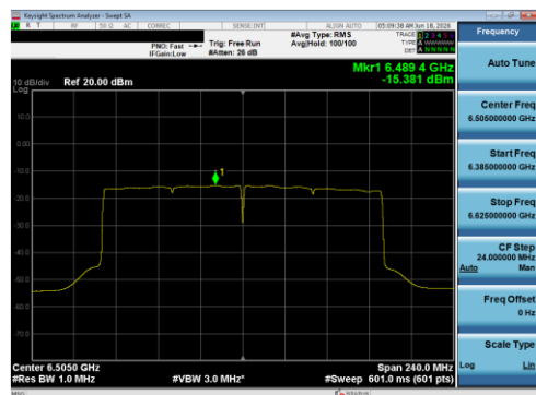
Plot 7-144 PSD CDD Diversity Antenna 1B (160 MHz BW 802.11be(SU) - Ch.111)
