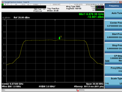
Plot 7-113 PSD SDM Primary Antenna 5T (20 MHz BW 802.11be(SU) - Ch.185)
