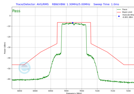
Plot 7-207 In-Band Emission Plot Antenna 1B (80 MHz BW 802.11be(SU) (UNII Band 8) - Ch.215)
