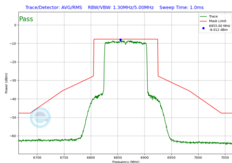
Plot 7-187 In-Band Emission Plot Antenna 5B (80 MHz BW 802.11be(SU) (UNII Band 7) - Ch.183)
