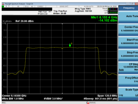
Plot 7-99 PSD SDM Primary Antenna 5T (80 MHz BW 802.11be(SU) - Ch.39)
