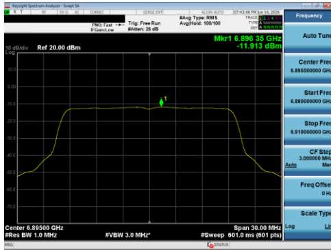
Plot 7-121 PSD SDM Primary Antenna 5T (20 MHz BW 802.11be(SU) - Ch.189)
