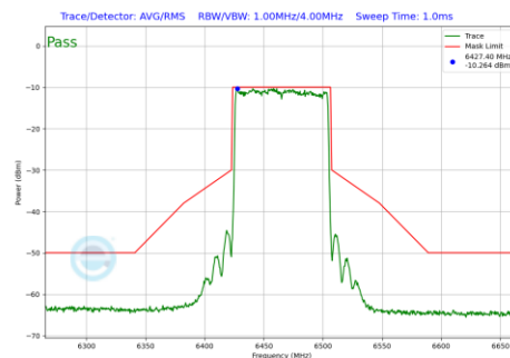
Plot 7-183 In-Band Emission Plot Antenna 5B (80 MHz BW 802.11be(SU) (UNII Band 6) - Ch.103)
