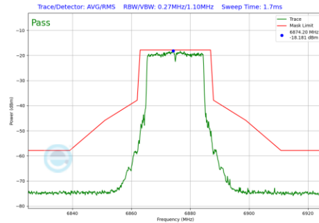
Plot 7-229 In-Band Emission Plot SDM Primary Antenna 5B (20 MHz BW 802.11be(SU) (UNII Band 7) - Ch.185)
