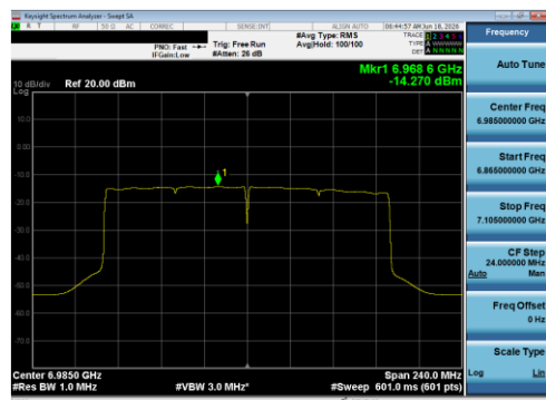
Plot 7-160 PSD CDD Diversity Antenna 1B (160 MHz BW 802.11be(SU) - Ch.207)
