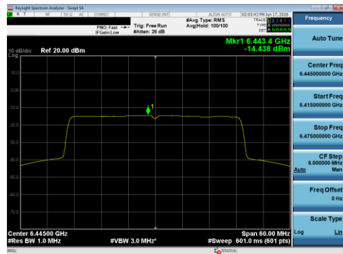
Plot 7-110 PSD SDM Primary Antenna 5B (40 MHz BW 802.11be(SU) - Ch.99)
