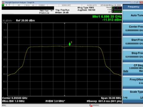
Plot 7-153 PSD CDD Diversity Antenna 5T (20 MHz BW 802.11be(SU) - Ch.189)
