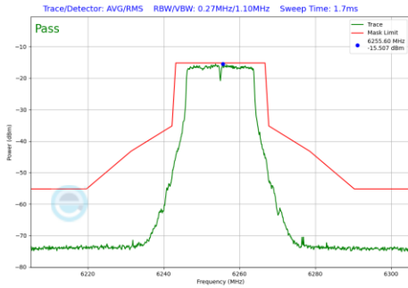
Plot 7-177 In-Band Emission Plot Antenna 5B (20 MHz BW 802.11a (UNII Band 5) - Ch.61)
