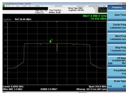
Plot 7-128 PSD SDM Primary Antenna 5B (160 MHz BW 802.11be(SU) - Ch.207)
