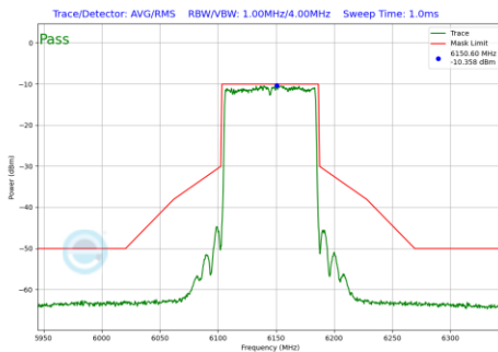
Plot 7-163 In-Band Emission Plot Antenna 5T (80 MHz BW 802.11be(SU) (UNII Band 5) - Ch.39)
