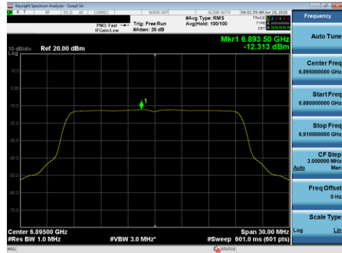
Plot 7-157 PSD CDD Diversity Antenna 1B (20 MHz BW 802.11be(SU) - Ch.189)
