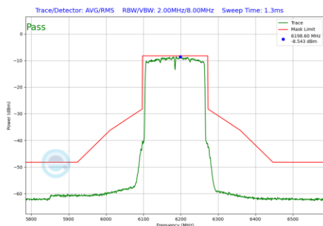
Plot 7-196 In-Band Emission Plot Antenna 1B (160 MHz BW 802.11be(SU) (UNII Band 5) - Ch.47)
