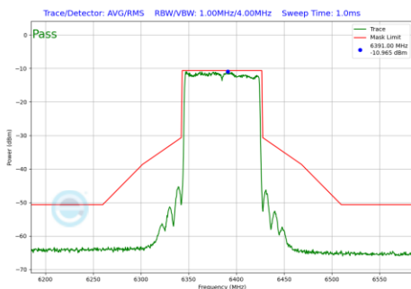
Plot 7-179 In-Band Emission Plot Antenna 5B (80 MHz BW 802.11be(SU) (UNII Band 5) - Ch.87)
