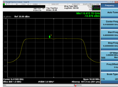
Plot 7-101 PSD SDM Primary Antenna 5B (20 MHz BW 802.11be(SU) - Ch.93)
