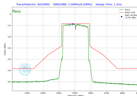
Plot 7-184 In-Band Emission Plot Antenna 5B (160 MHz BW 802.11be(SU) (UNII Band 6) - Ch.111)
