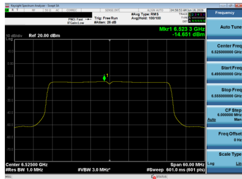
Plot 7-142 PSD CDD Diversity Antenna 1B (40 MHz BW 802.11be(SU) - Ch.115)
