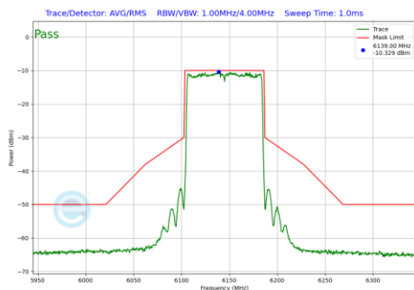
Plot 7-195 In-Band Emission Plot Antenna 1B (80 MHz BW 802.11be(SU) (UNII Band 5) - Ch.39)
