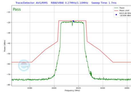
Plot 7-213 In-Band Emission Plot SDM Primary Antenna 5B (20 MHz BW 802.11be(SU) (UNII Band 5) - Ch.93)
