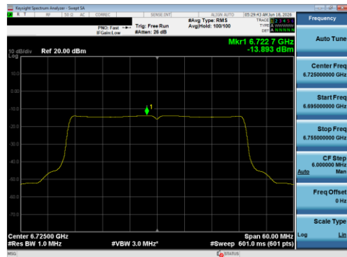
Plot 7-150 PSD CDD Diversity Antenna 1B (40 MHz BW 802.11be(SU) - Ch.155)
