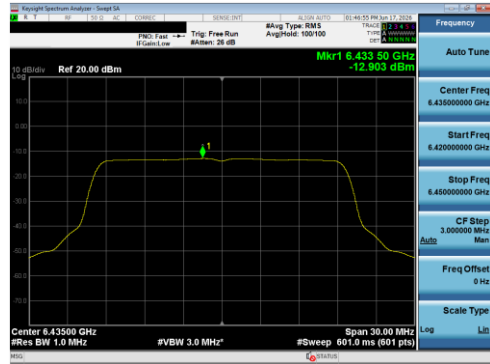
Plot 7-109 PSD SDM Primary Antenna 5B (20 MHz BW 802.11be(SU) - Ch.97)
