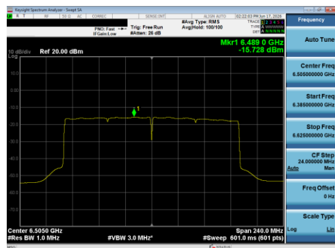
Plot 7-112 PSD SDM Primary Antenna 5B (160 MHz BW 802.11be(SU) - Ch.111)
