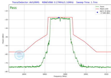
Plot 7-225 In-Band Emission Plot SDM Primary Antenna 5T (20 MHz BW 802.11be(SU) (UNII Band 7) - Ch.185)
