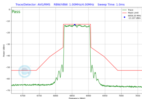
Plot 7-227 In-Band Emission Plot SDM Primary Antenna 5T (80 MHz BW 802.11be(SU) (UNII Band 7) - Ch.183)
