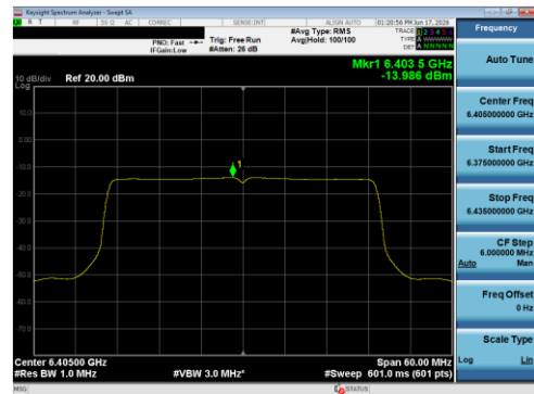
Plot 7-102 PSD SDM Primary Antenna 5B (40 MHz BW 802.11be(SU) - Ch.91)
