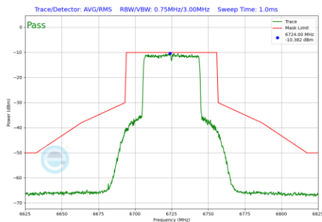
Plot 7-186 In-Band Emission Plot Antenna 5B (40 MHz BW 802.11be(SU) (UNII Band 7) - Ch.155)
