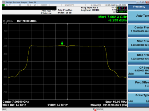
Plot 7-94 PSD Antenna 1B (40 MHz BW 802.11be(SU) - Ch.211)
