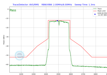
Plot 7-224 In-Band Emission Plot SDM Primary Antenna 5B (160 MHz BW 802.11be(SU) (UNII Band 6) - Ch.111)
