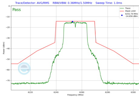
Plot 7-193 In-Band Emission Plot Antenna 1B (20 MHz BW 802.11a (UNII Band 5) - Ch.61)
