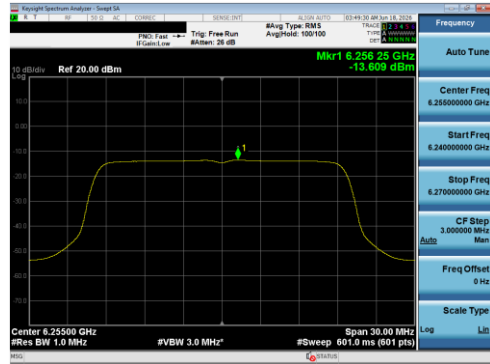
Plot 7-133 PSD CDD Diversity Antenna 1B (20 MHz BW 802.11be(SU) - Ch.61)
