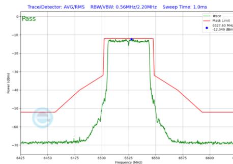
Plot 7-182 In-Band Emission Plot Antenna 5B (40 MHz BW 802.11be(SU) (UNII Band 6) - Ch.115)
