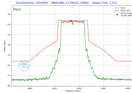
Plot 7-181 In-Band Emission Plot Antenna 5B (20 MHz BW 802.11be(SU) (UNII Band 6) - Ch.97)
