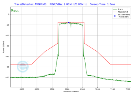
Plot 7-188 In-Band Emission Plot Antenna 5B (160 MHz BW 802.11be(SU) (UNII Band 7) - Ch.175)
