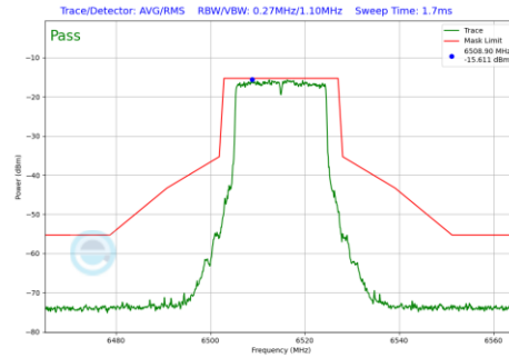
Plot 7-165 In-Band Emission Plot Antenna 5T (20 MHz BW 802.11be(SU) (UNII Band 6) - Ch.113)
