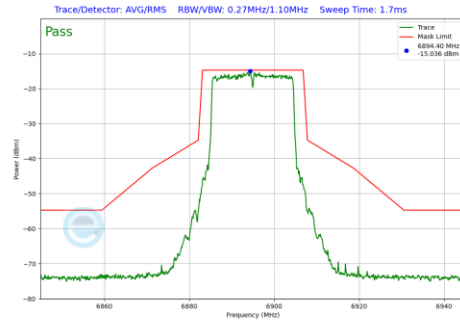
Plot 7-173 In-Band Emission Plot Antenna 5T (20 MHz BW 802.11be(SU) (UNII Band 8) - Ch.189)
