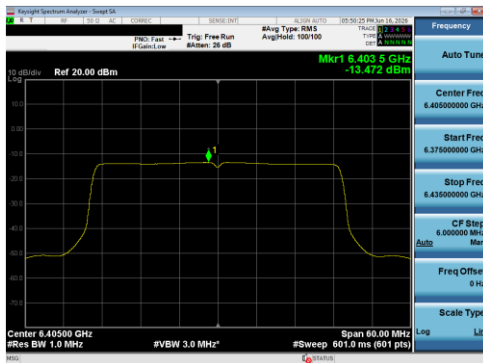
Plot 7-98 PSD SDM Primary Antenna 5T (40 MHz BW 802.11be(SU) - Ch.91)
