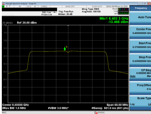
Plot 7-130 PSD CDD Diversity Antenna 5T (40 MHz BW 802.11be(SU) - Ch.91)
