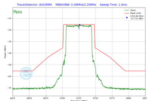
Plot 7-230 In-Band Emission Plot SDM Primary Antenna 5B (40 MHz BW 802.11be(SU) (UNII Band 7) - Ch.155)
