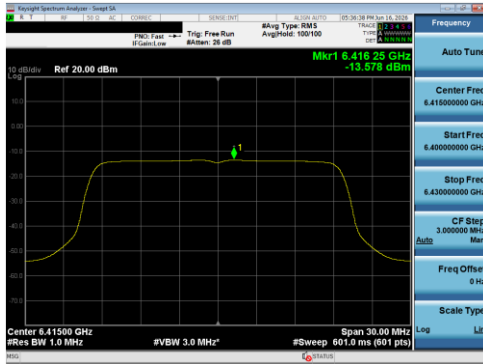
Plot 7-97 PSD SDM Primary Antenna 5T (20 MHz BW 802.11be(SU) - Ch.93)
