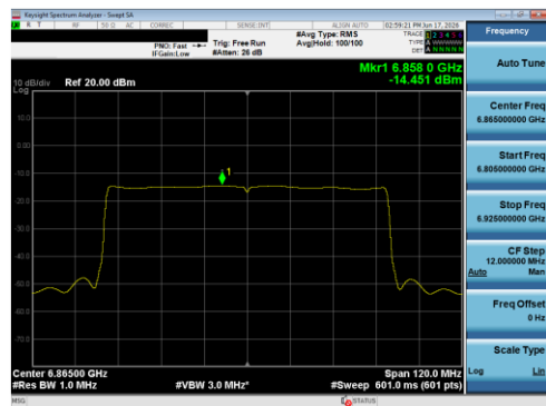
Plot 7-119 PSD SDM Primary Antenna 5B (80 MHz BW 802.11be(SU) - Ch.183)
