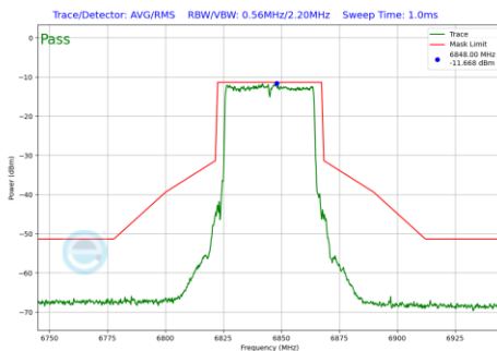
Plot 7-202 In-Band Emission Plot Antenna 1B (40 MHz BW 802.11be(SU) (UNII Band 7) - Ch.179)
