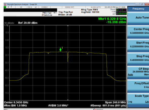
Plot 7-104 PSD SDM Primary Antenna 5B (160 MHz BW 802.11be(SU) - Ch.79)
