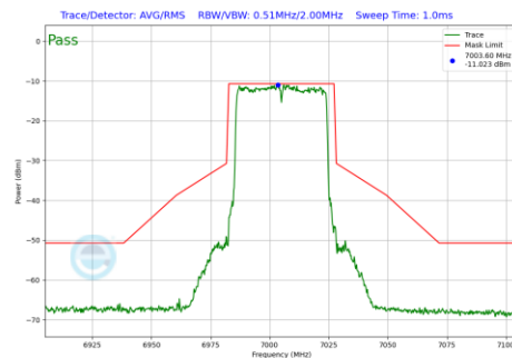
Plot 7-190 In-Band Emission Plot Antenna 5B (40 MHz BW 802.11be(SU) (UNII Band 8) - Ch.211)
