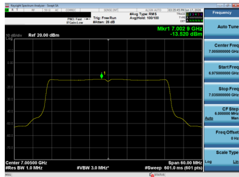
Plot 7-126 PSD SDM Primary Antenna 5B (40 MHz BW 802.11be(SU) - Ch.211)
