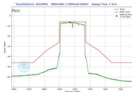
Plot 7-192 In-Band Emission Plot Antenna 5B (160 MHz BW 802.11be(SU) (UNII Band 8) - Ch.207)
