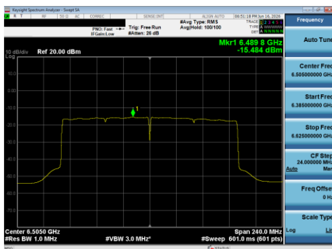
Plot 7-140 PSD CDD Diversity Antenna 5T (160 MHz BW 802.11be(SU) - Ch.111)
