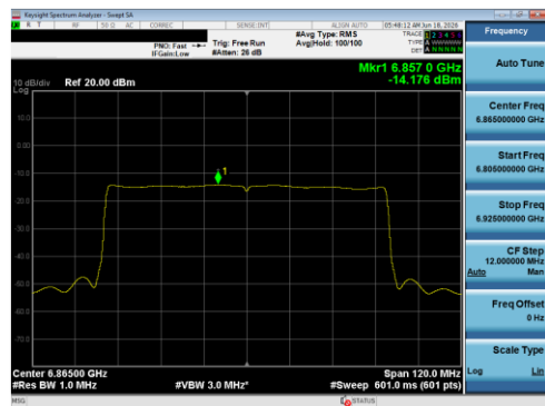
Plot 7-151 PSD CDD Diversity Antenna 1B (80 MHz BW 802.11be(SU) - Ch.183)
