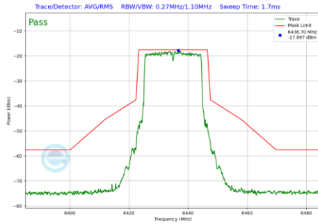
Plot 7-217 In-Band Emission Plot SDM Primary Antenna 5T (20 MHz BW 802.11be(SU) (UNII Band 6) - Ch.97)
