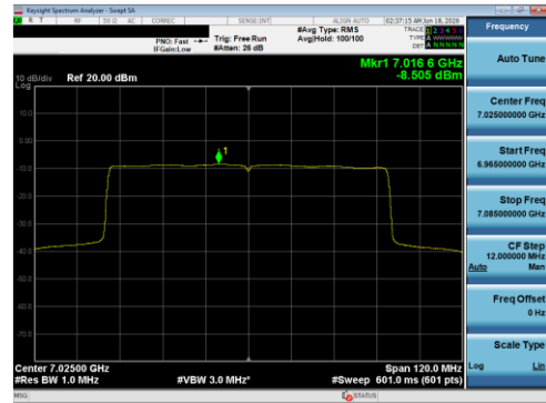
Plot 7-95 PSD Antenna 1B (80 MHz BW 802.11be(SU) - Ch.215)
