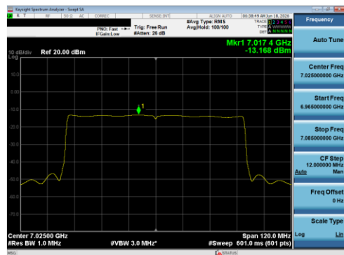
Plot 7-159 PSD CDD Diversity Antenna 1B (80 MHz BW 802.11be(SU) - Ch.215)
