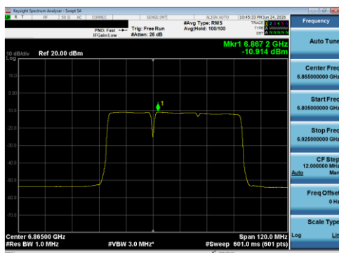
Plot 7-156 PSD Antenna 5T (80 MHz BW 802.11be(RU) RU484+242 Index90 - Ch.183)
