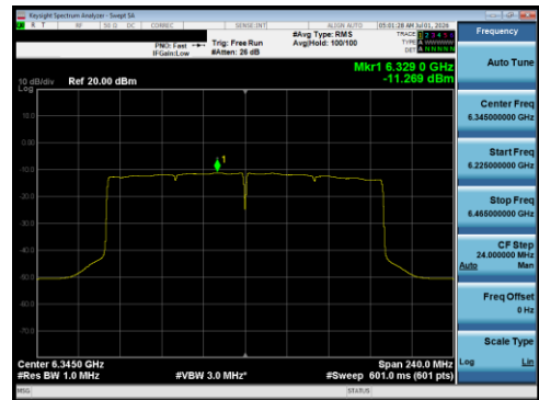
Plot 7-139 PSD Antenna 5T (160 MHz BW 802.11be(RU) RU996X2 Index68 - Ch.79)
