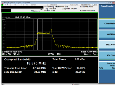
Plot 7-119 26dB BW & 99% OBW Antenna 1B (40MHz BW 802.11be(RU) RU26 Index8 - Ch.123)
