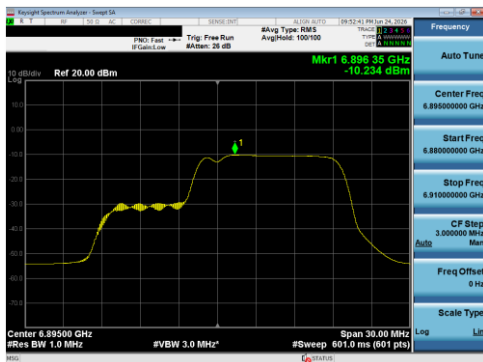
Plot 7-166 PSD Antenna 5T (20 MHz BW 802.11be(RU) RU106+26 Index83 - Ch.189)
