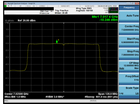
Plot 7-171 PSD Antenna 5T (80 MHz BW 802.11be(RU) RU996 Index67 - Ch.215)
