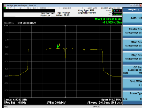
Plot 7-194 PSD Antenna 5B (160 MHz BW 802.11be(RU) RU996X2 Index68 - Ch.111)
