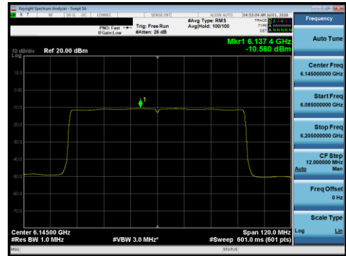
Plot 7-138 PSD Antenna 5T (80 MHz BW 802.11be(RU) RU996 Index67 - Ch.39)
