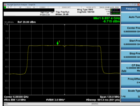
Plot 7-204 PSD Antenna 5B (80 MHz BW 802.11be(RU) RU996 Index67 - Ch.183)
