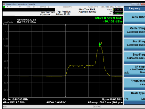
Plot 7-141 PSD Antenna 5T (40 MHz BW 802.11be(RU) RU26 Index17 - Ch.107)
