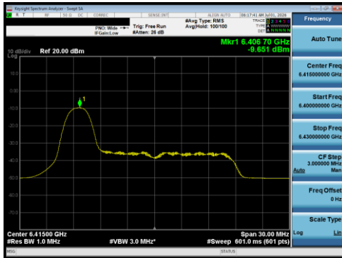
Plot 7-129 PSD Antenna 5T (20 MHz BW 802.11be(RU) RU26 Index0 - Ch.93)
