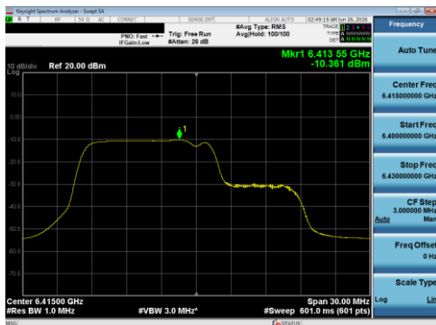
Plot 7-177 PSD Antenna 5B (20 MHz BW 802.11be(RU) RU106+26 Index82 - Ch.93)
