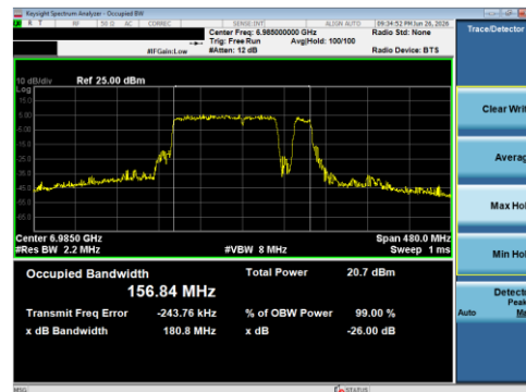
Plot 7-124 26 dB BW & 99% OBW Antenna 1B (160 MHz BW 802.11be(RU) RU996+484+242 Index98 - Ch.207)
