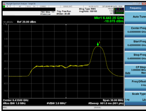
Plot 7-140 PSD Antenna 5T (20 MHz BW 802.11be(RU) RU26 Index8 - Ch.97)
