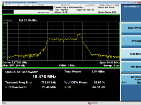
Plot 7-118 26dB BW & 99% OBW Antenna 1B (20MHz BW 802.11be(RU) RU26 Index8 - Ch.185)
