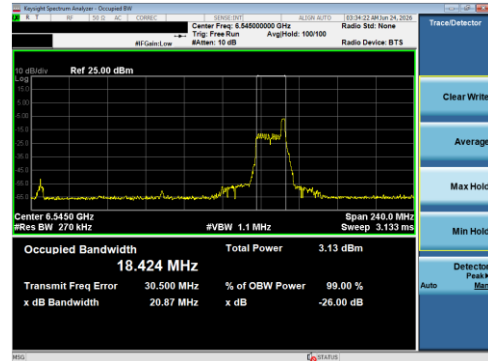
Plot 7-120 26dB BW & 99% OBW Antenna 1B (80MHz BW 802.11be(RU) RU26 Index36 - Ch.119)
