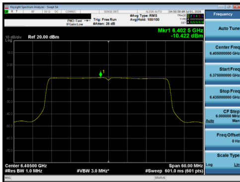
Plot 7-137 PSD Antenna 5T (40 MHz BW 802.11be(RU) RU484 Index65 - Ch.91)
