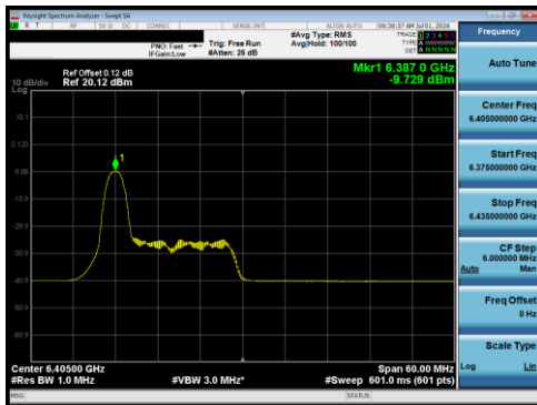
Plot 7-130 PSD Antenna 5T (40 MHz BW 802.11be(RU) RU26 Index0 - Ch.91)
