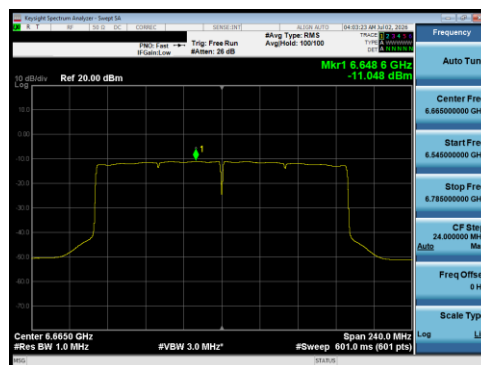
Plot 7-205 PSD Antenna 5B (160 MHz BW 802.11be(RU) RU996X2 Index68 - Ch.143)
