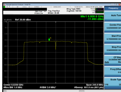
Plot 7-161 PSD Antenna 5T (160 MHz BW 802.11be(RU) RU996X2 Index68 - Ch.175)
