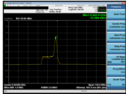
Plot 7-164 PSD Antenna 5T (80 MHz BW 802.11be(RU) RU26 Index17 - Ch.199)
