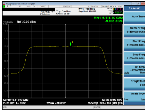
Plot 7-136 PSD Antenna 5T (20 MHz BW 802.11be(RU) RU242 Index61 - Ch.33)
