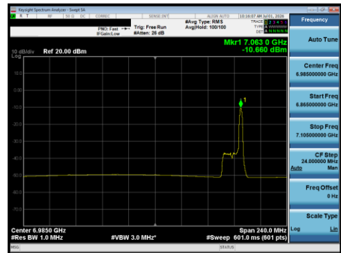
Plot 7-165 PSD Antenna 5T (160 MHz BW 802.11be(RU) RU26 Index36 - Ch.207)
