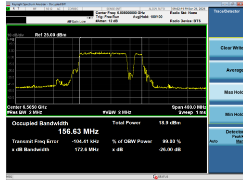
Plot 7-102 26 dB BW & 99% OBW Antenna 1B (160 MHz BW 802.11be(RU) RU996+484+242 Index98 - Ch.111)
