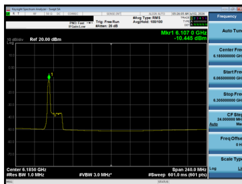
Plot 7-176 PSD Antenna 5B (160 MHz BW 802.11be(RU) RU26 Index0 - Ch.47)
