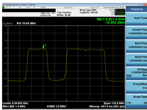
Plot 7-167 PSD Antenna 5T (80 MHz BW 802.11be(RU) RU484+242 Index91 - Ch.199)
