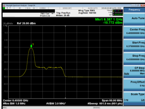
Plot 7-174 PSD Antenna 5B (40 MHz BW 802.11be(RU) RU26 Index0 - Ch.91)
