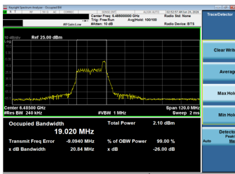
Plot 7-108 26dB BW & 99% OBW Antenna 1B (40MHz BW 802.11be(RU) RU26 Index8 - Ch.107)
