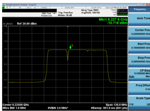
Plot 7-134 PSD Antenna 5T (80 MHz BW 802.11be(RU) RU484+242 Index90 - Ch.55)
