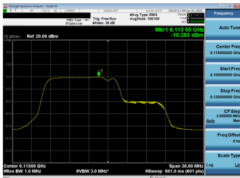
Plot 7-133 PSD Antenna 5T (20 MHz BW 802.11be(RU) RU106+26 Index82 - Ch.33)
