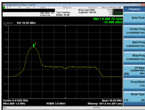
Plot 7-173 PSD Antenna 5B (20 MHz BW 802.11be(RU) RU26 Index0 - Ch.93)
