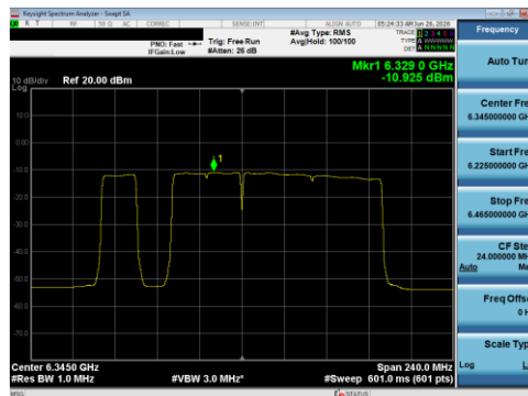
Plot 7-179 PSD Antenna 5B (160 MHz BW 802.11be(RU) RU996+484+242 Index97 - Ch.79)
