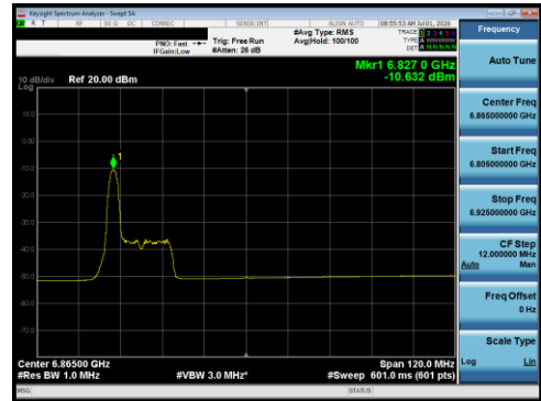
Plot 7-153 PSD Antenna 5T (80 MHz BW 802.11be(RU) RU26 Index0 - Ch.183)
