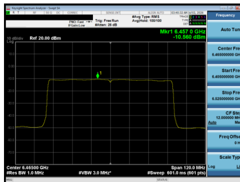
Plot 7-193 PSD Antenna 5B (80MHz BW 802.11be(RU) RU996 Index67 - Ch.103)
