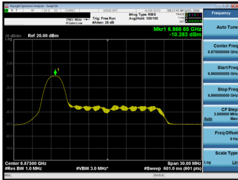
Plot 7-151 PSD Antenna 5T (20 MHz BW 802.11be(RU) RU26 Index0 - Ch.185)
