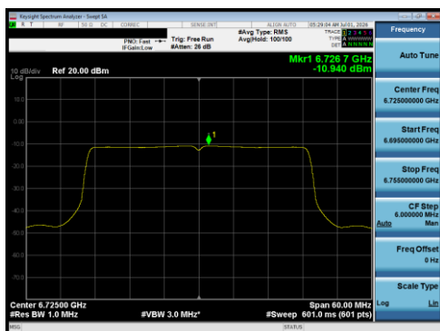
Plot 7-159 PSD Antenna 5T (40 MHz BW 802.11be(RU) RU484 Index65 - Ch.155)
