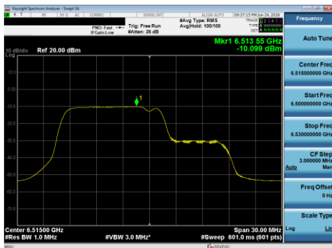
Plot 7-144 PSD Antenna 5T (20 MHz BW 802.11be(RU) RU106+26 Index82 - Ch.113)
