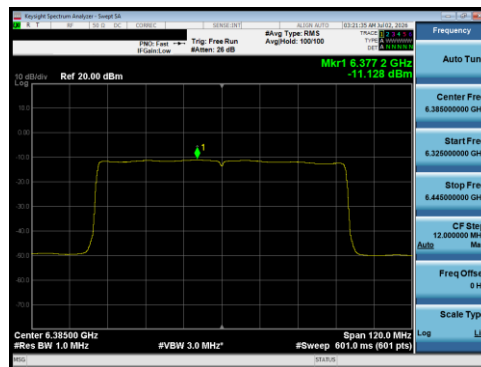
Plot 7-182 PSD Antenna 5B (80 MHz BW 802.11be(RU) RU996 Index67 - Ch.87)
