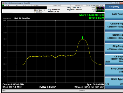
Plot 7-184 PSD Antenna 5B (20 MHz BW 802.11be(RU) RU26 Index8 - Ch.113)
