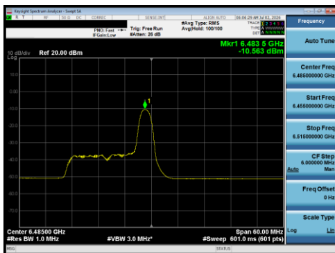
Plot 7-185 PSD Antenna 5B (40 MHz BW 802.11be(RU) RU26 Index8 - Ch.107)
