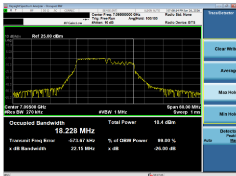
Plot 7-122 26 dB BW & 99% OBW Antenna 1B (20 MHz BW 802.11be(RU) RU106+26 Index82 - Ch.229)
