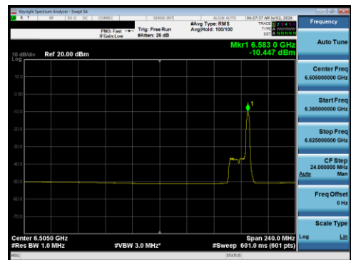
Plot 7-187 PSD Antenna 5B (160 MHz BW 802.11be(RU) RU26 Index36 - Ch.111)
