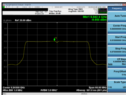
Plot 7-203 PSD Antenna 5B (40 MHz BW 802.11be(RU) RU484 Index65 - Ch.179)
