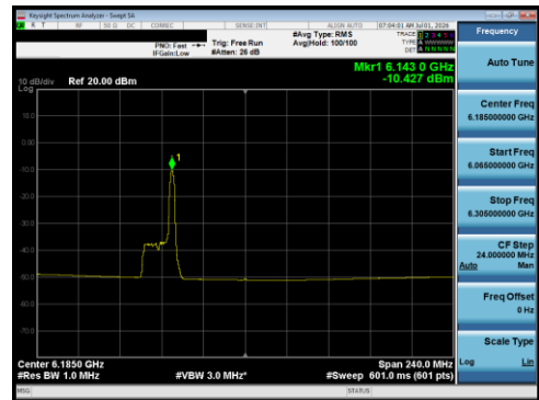
Plot 7-132 PSD Antenna 5T (160 MHz BW 802.11be(RU) RU26 Index17 - Ch.47)
