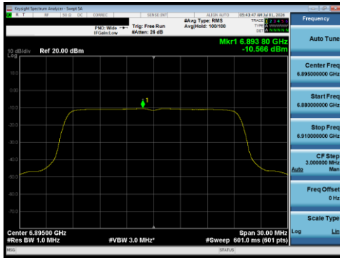
Plot 7-169 PSD Antenna 5T (20 MHz BW 802.11be(RU) RU242 Index61 - Ch.189)
