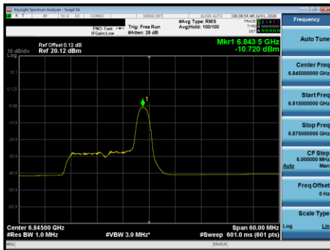
Plot 7-152 PSD Antenna 5T (40 MHz BW 802.11be(RU) RU26 Index8 - Ch.179)
