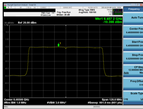
Plot 7-149 PSD Antenna 5T (80MHz BW 802.11be(RU) RU996 Index67 - Ch.103)
