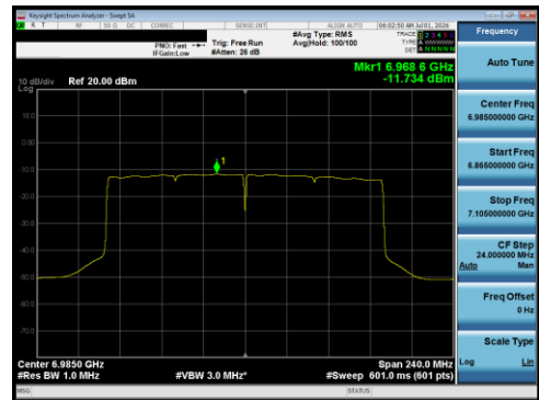
Plot 7-172 PSD Antenna 5T (160 MHz BW 802.11be(RU) RU996X2 Index68 - Ch.207)
