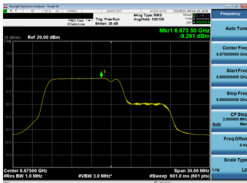
Plot 7-199 PSD Antenna 5B (20 MHz BW 802.11be(RU) RU106+26 Index82 - Ch.185)
