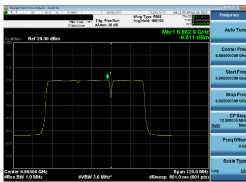
Plot 7-200 PSD Antenna 5B (80 MHz BW 802.11be(RU) RU484+242 Index93 - Ch.183)
