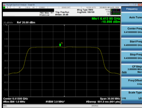
Plot 7-180 PSD Antenna 5B (20 MHz BW 802.11be(RU) RU242 Index61 - Ch.93)
