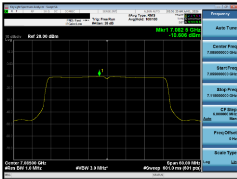
Plot 7-170 PSD Antenna 5T (40 MHz BW 802.11be(RU) RU484 Index65 - Ch.227)
