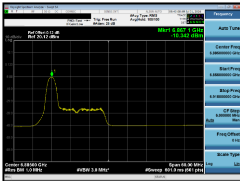
Plot 7-163 PSD Antenna 5T (40 MHz BW 802.11be(RU) RU26 Index0 - Ch.187)
