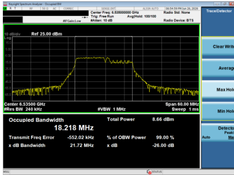
Plot 7-111 26 dB BW & 99% OBW Antenna 1B (20 MHz BW 802.11be(RU) RU106+26 Index82 - Ch.117)
