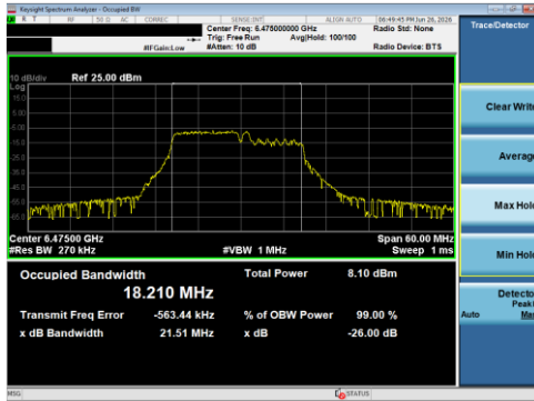
Plot 7-100 26 dB BW & 99% OBW Antenna 1B (20 MHz BW 802.11be(RU) RU106+26 Index82 - Ch.105)
