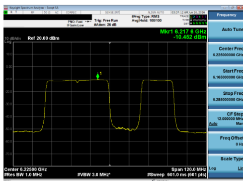
Plot 7-178 PSD Antenna 5B (80 MHz BW 802.11be(RU) RU484+242 Index92 - Ch.55)
