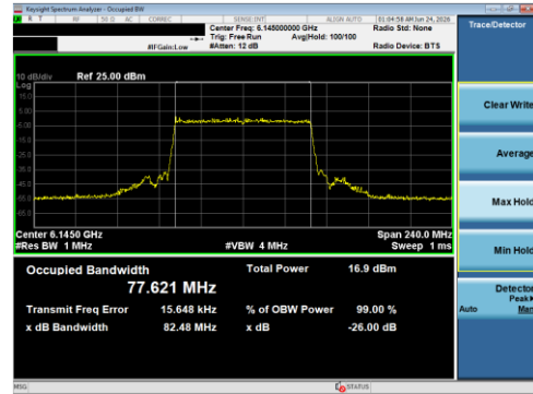
Plot 7-98 26 dB BW & 99% OBW Antenna 1B (80 MHz BW 802.11be(RU) RU996 Index67 - Ch.39)
