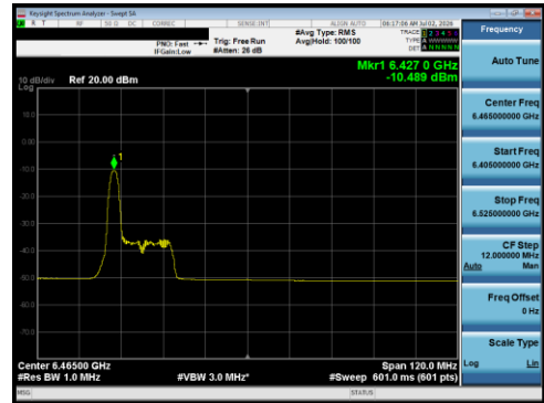
Plot 7-186 PSD Antenna 5B (80MHz BW 802.11be(RU) RU26 Index0 - Ch.103)
