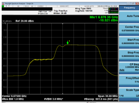
Plot 7-155 PSD Antenna 5T (20 MHz BW 802.11be(RU) RU106+26 Index83 - Ch.185)
