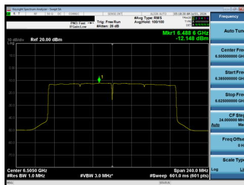
Plot 7-150 PSD Antenna 5T (160 MHz BW 802.11be(RU) RU996X2 Index68 - Ch.111)
