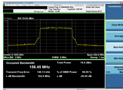
Plot 7-99 26 dB BW & 99% OBW Antenna 1B (160 MHz BW 802.11be(RU) RU996X2 Index68 - Ch.47)
