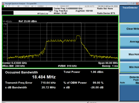
Plot 7-107 26dB BW & 99% OBW Antenna 1B (20MHz BW 802.11be(RU) RU26 Index8 - Ch.97)
