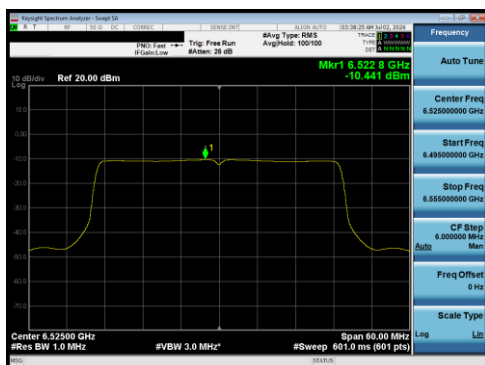
Plot 7-192 PSD Antenna 5B (40 MHz BW 802.11be(RU) RU484 Index65 - Ch.115)
