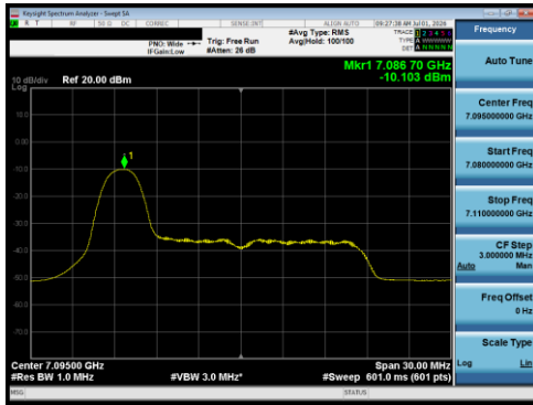
Plot 7-162 PSD Antenna 5T (20 MHz BW 802.11be(RU) RU26 Index0 - Ch.229)
