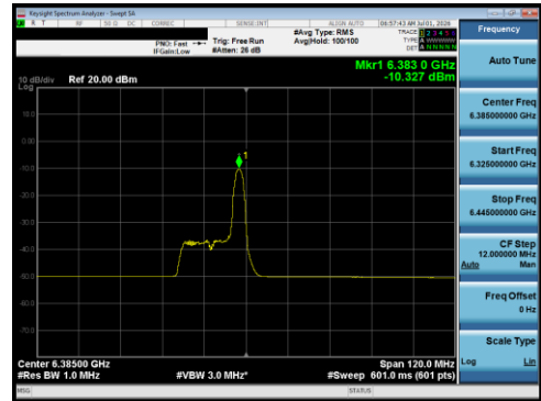
Plot 7-131 PSD Antenna 5T (80 MHz BW 802.11be(RU) RU26 Index17 - Ch.87)
