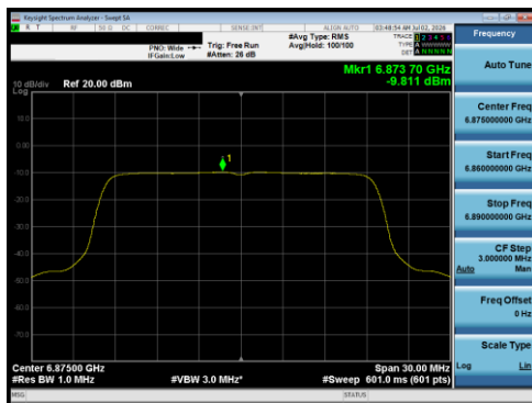
Plot 7-202 PSD Antenna 5B (20 MHz BW 802.11be(RU) RU242 Index61 - Ch.185)
