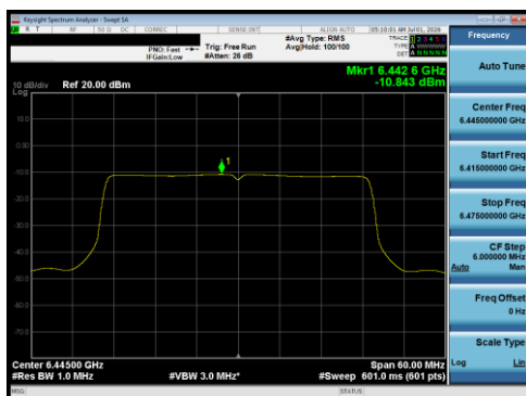
Plot 7-148 PSD Antenna 5T (40 MHz BW 802.11be(RU) RU484 Index65 - Ch.99)
