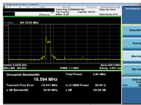
Plot 7-110 26dB BW & 99% OBW Antenna 1B (160MHz BW 802.11be(RU) RU26 Index0 - Ch.111)
