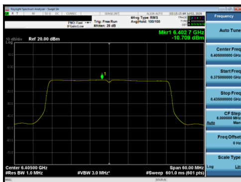
Plot 7-181 PSD Antenna 5B (40 MHz BW 802.11be(RU) RU484 Index65 - Ch.91)
