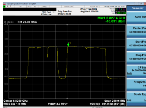
Plot 7-201 PSD Antenna 5B (160 MHz BW 802.11be(RU) RU996+484+242 Index99 - Ch.175)
