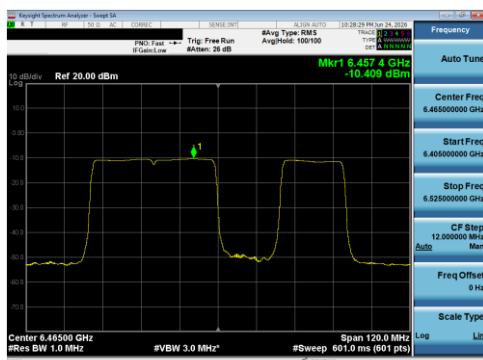
Plot 7-145 PSD Antenna 5T (80 MHz BW 802.11be(RU) RU484+242 Index92 - Ch.103)
