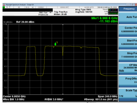
Plot 7-168 PSD Antenna 5T (160 MHz BW 802.11be(RU) RU996+484+242 Index97 - Ch.207)
