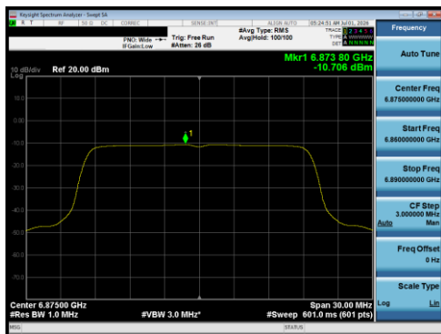
Plot 7-158 PSD Antenna 5T (20 MHz BW 802.11be(RU) RU242 Index61 - Ch.185)
