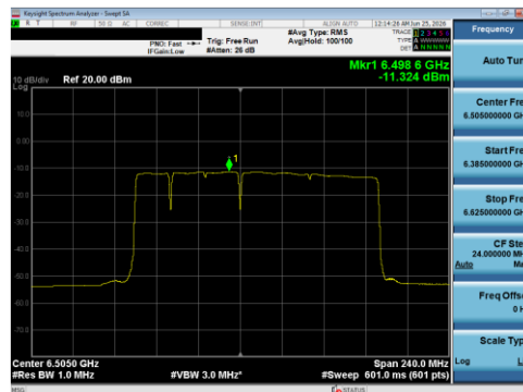
Plot 7-146 PSD Antenna 5T (160 MHz BW 802.11be(RU) RU996+484+242 Index96 - Ch.111)
