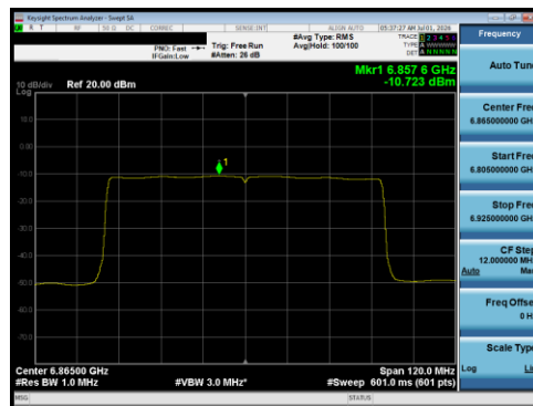
Plot 7-160 PSD Antenna 5T (80 MHz BW 802.11be(RU) RU996 Index67 - Ch.183)
