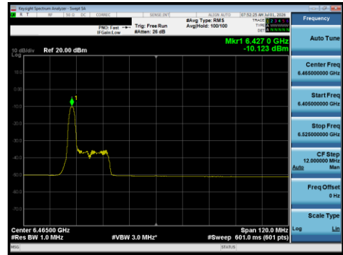
Plot 7-142 PSD Antenna 5T (80MHz BW 802.11be(RU) RU26 Index0 - Ch.103)
