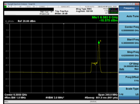
Plot 7-143 PSD Antenna 5T (160 MHz BW 802.11be(RU) RU26 Index36 - Ch.111)
