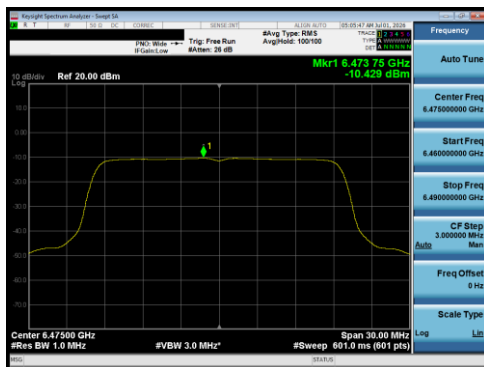
Plot 7-147 PSD Antenna 5T (20 MHz BW 802.11be(RU) RU242 Index61 - Ch.105)
