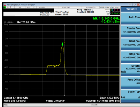
Plot 7-175 PSD Antenna 5B (80 MHz BW 802.11be(RU) RU26 Index17 - Ch.39)
