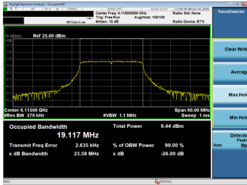
Plot 7-96 26 dB BW & 99% OBW Antenna 1B (20 MHz BW 802.11be(RU) RU242 Index61 - Ch.33)
