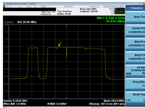
Plot 7-135 PSD Antenna 5T (160 MHz BW 802.11be(RU) RU996+484+242 Index97 - Ch.79)
