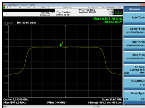
Plot 7-191 PSD Antenna 5B (20 MHz BW 802.11be(RU) RU242 Index61 - Ch.113)
