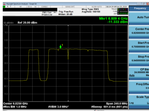
Plot 7-157 PSD Antenna 5T (160 MHz BW 802.11be(RU) RU996+484+242 Index97 - Ch.175)
