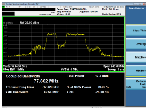
Plot 7-123 26 dB BW & 99% OBW Antenna 1B (80 MHz BW 802.11be(RU) RU484+242 Index91 - Ch.199)
