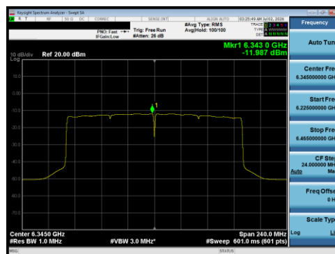
Plot 7-183 PSD Antenna 5B (160 MHz BW 802.11be(RU) RU996X2 Index68 - Ch.79)
