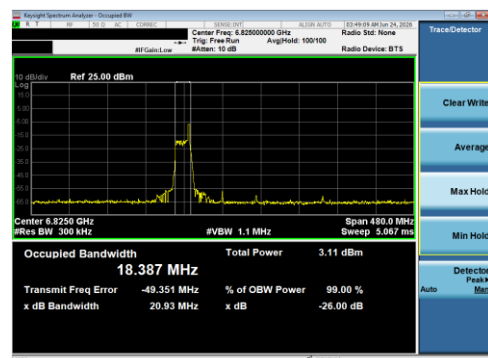
Plot 7-121 26dB BW & 99% OBW Antenna 1B (160MHz BW 802.11be(RU) RU26 Index17 - Ch.175)
