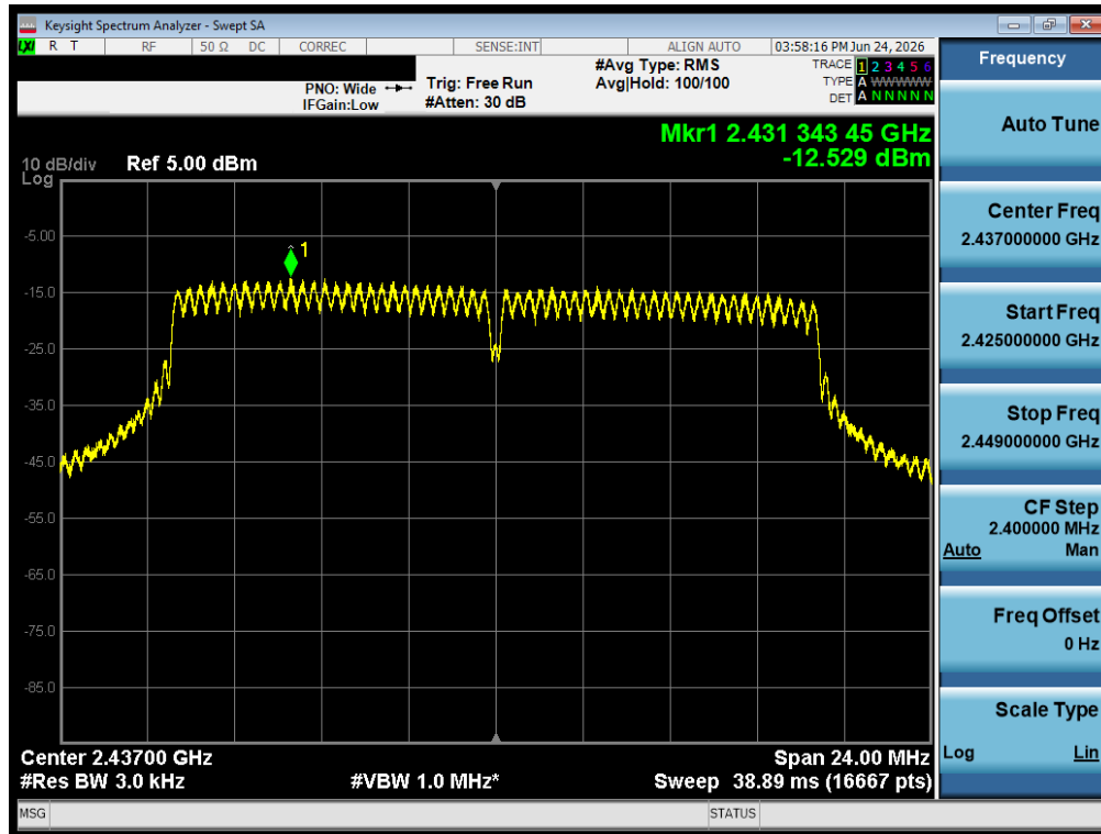
Plot 7-19 PSD Antenna 3A (20 MHz BW 802.11n - Ch.6)
