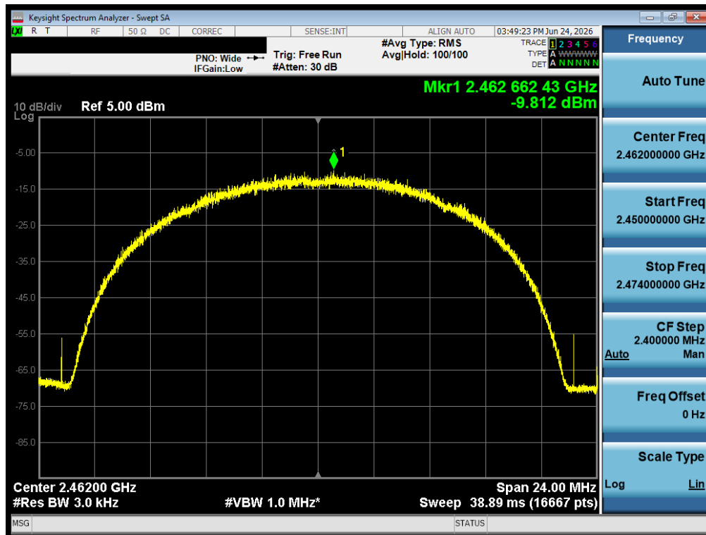
Plot 7-17 PSD Antenna 3A (20 MHz BW 802.11b - Ch.11)
