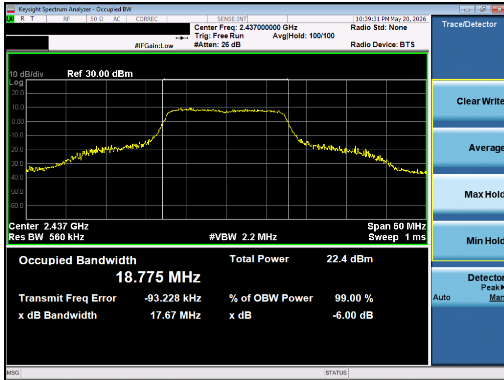
Plot 7-7 99% OBW Antenna 1A (20 MHz BW 802.11n - Ch.6)
