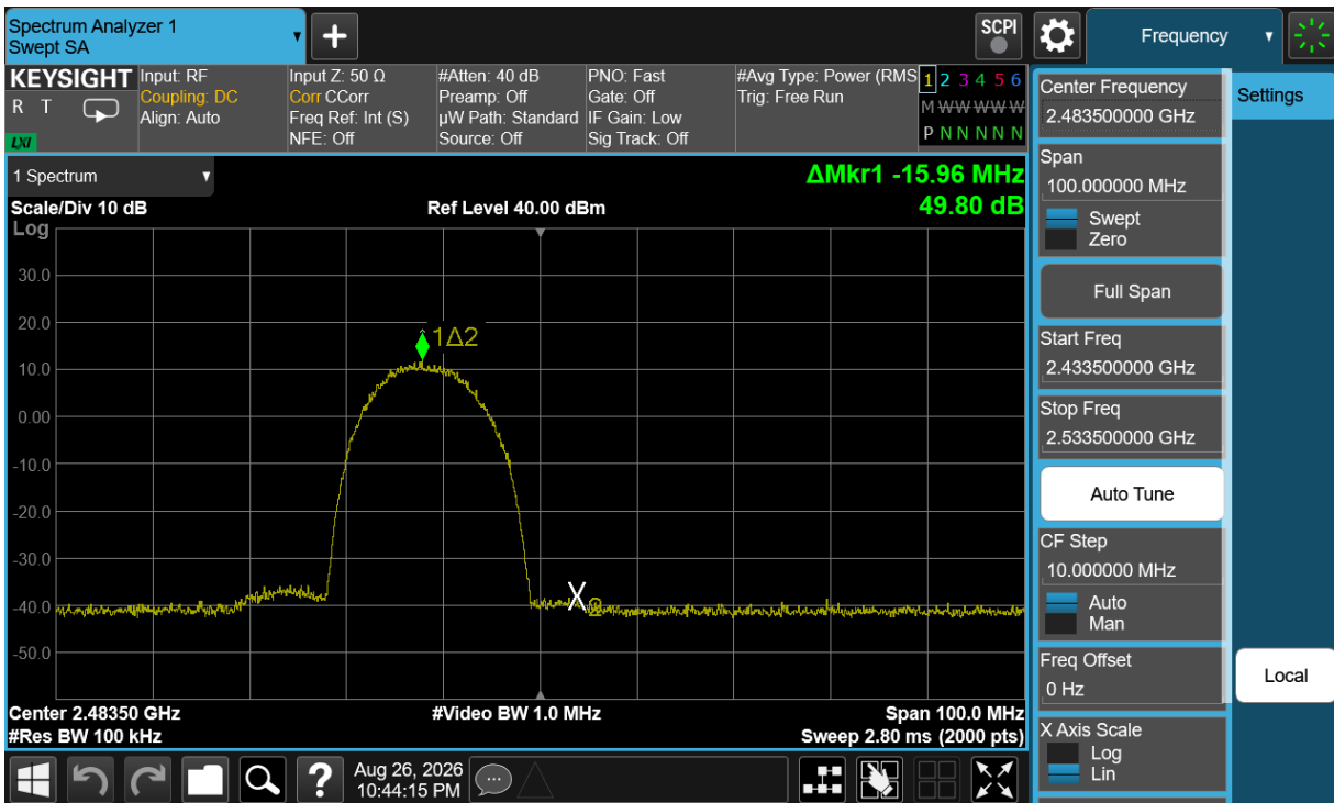
Plot 7-36. Band Edge Plot Antenna 3A (802.11b – Ch. 13)
