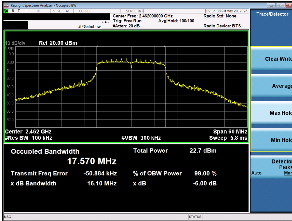
Plot 7-15 6 dB BW Antenna 1A (20 MHz BW 802.11n - Ch.11)
