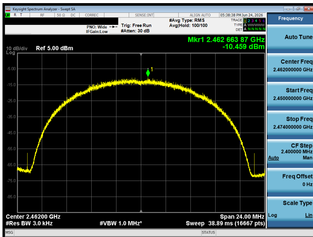
Plot 7-21 PSD Antenna 1A (20 MHz BW 802.11b - Ch.11)
