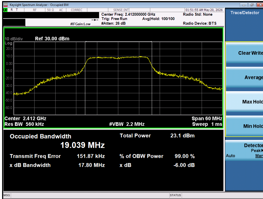
Plot 7-3 99% OBW Antenna 3A (20 MHz BW 802.11n - Ch.1)
