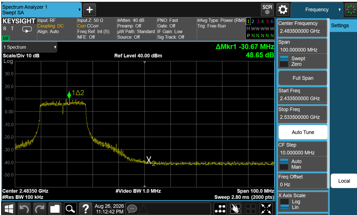
Plot 7-46. Band Edge Plot Antenna 3A (802.11g – Ch. 9)
