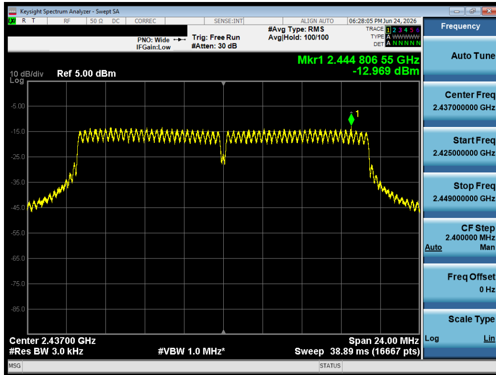
Plot 7-31 PSD CDD Antenna 1A (20 MHz BW 802.11n - Ch.6)
