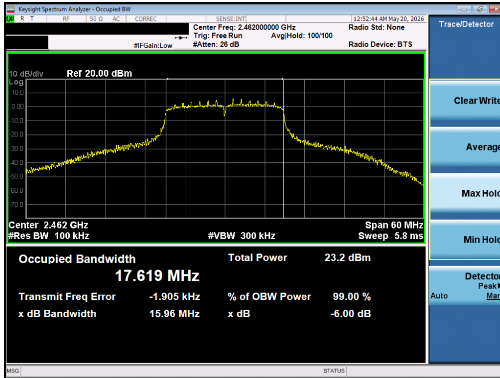
Plot 7-11 6 dB BW Antenna 3A (20 MHz BW 802.11n - Ch.11)
