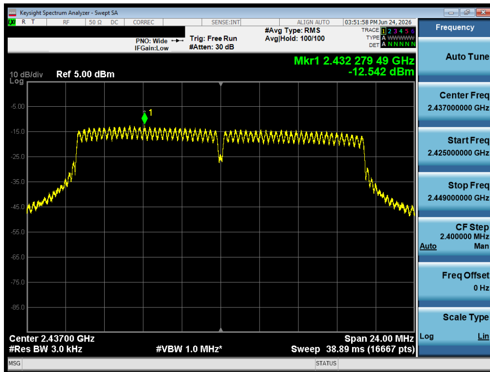
Plot 7-18 PSD Antenna 3A (20 MHz BW 802.11g - Ch.6)
