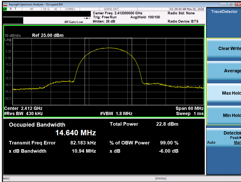
Plot 7-1 99% OBW Antenna 3A (20 MHz BW 802.11b - Ch.1)
