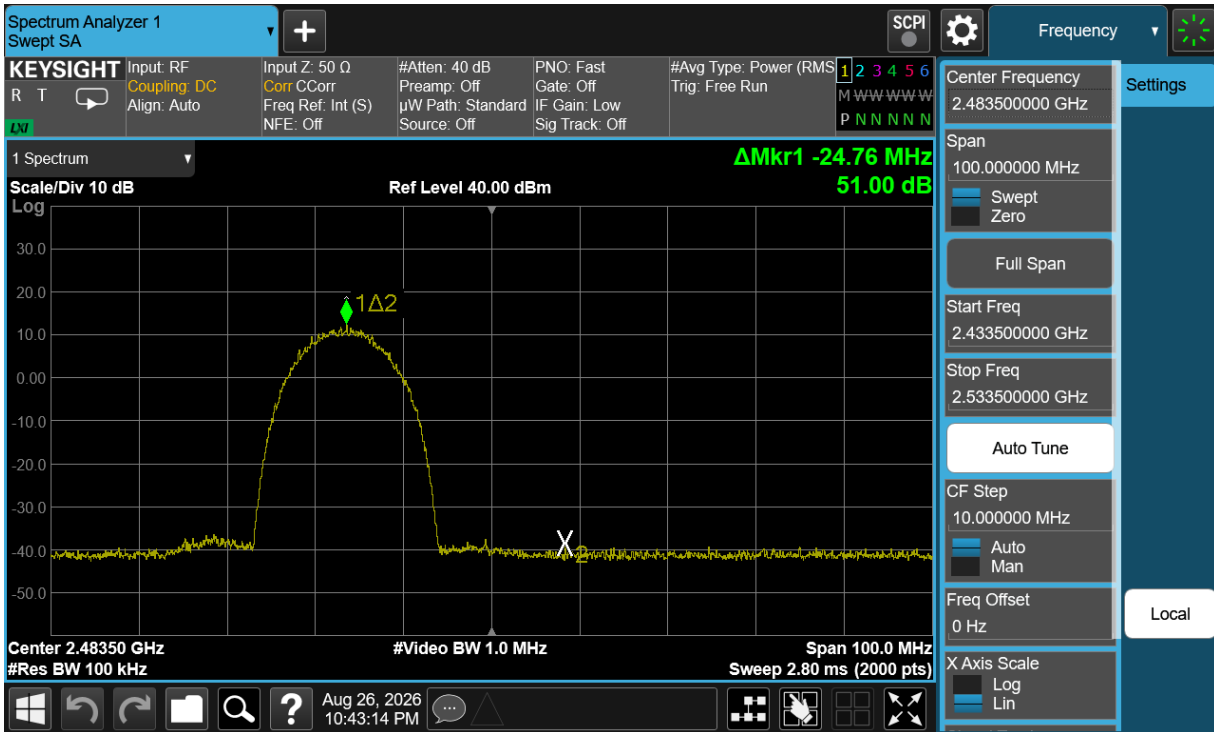
Plot 7-35. Band Edge Plot Antenna 3A (802.11b – Ch. 12)
