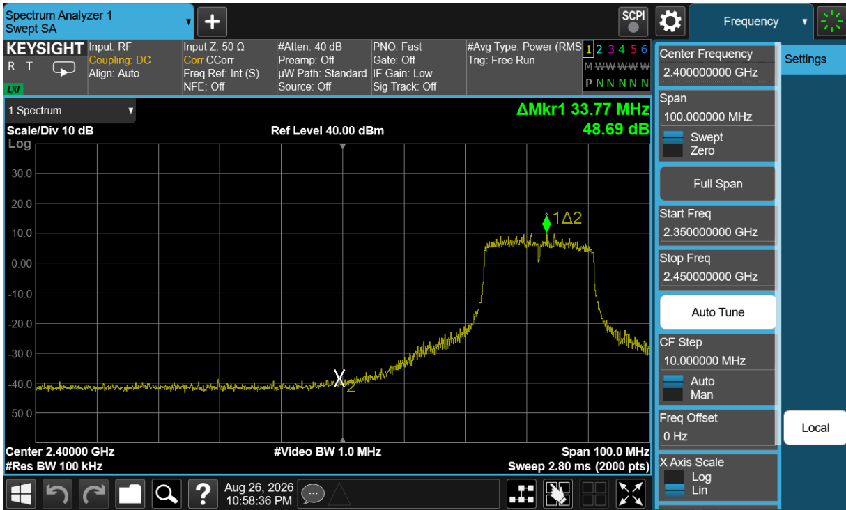
Plot 7-41. Band Edge Plot Antenna 3A (802.11g – Ch. 5)
