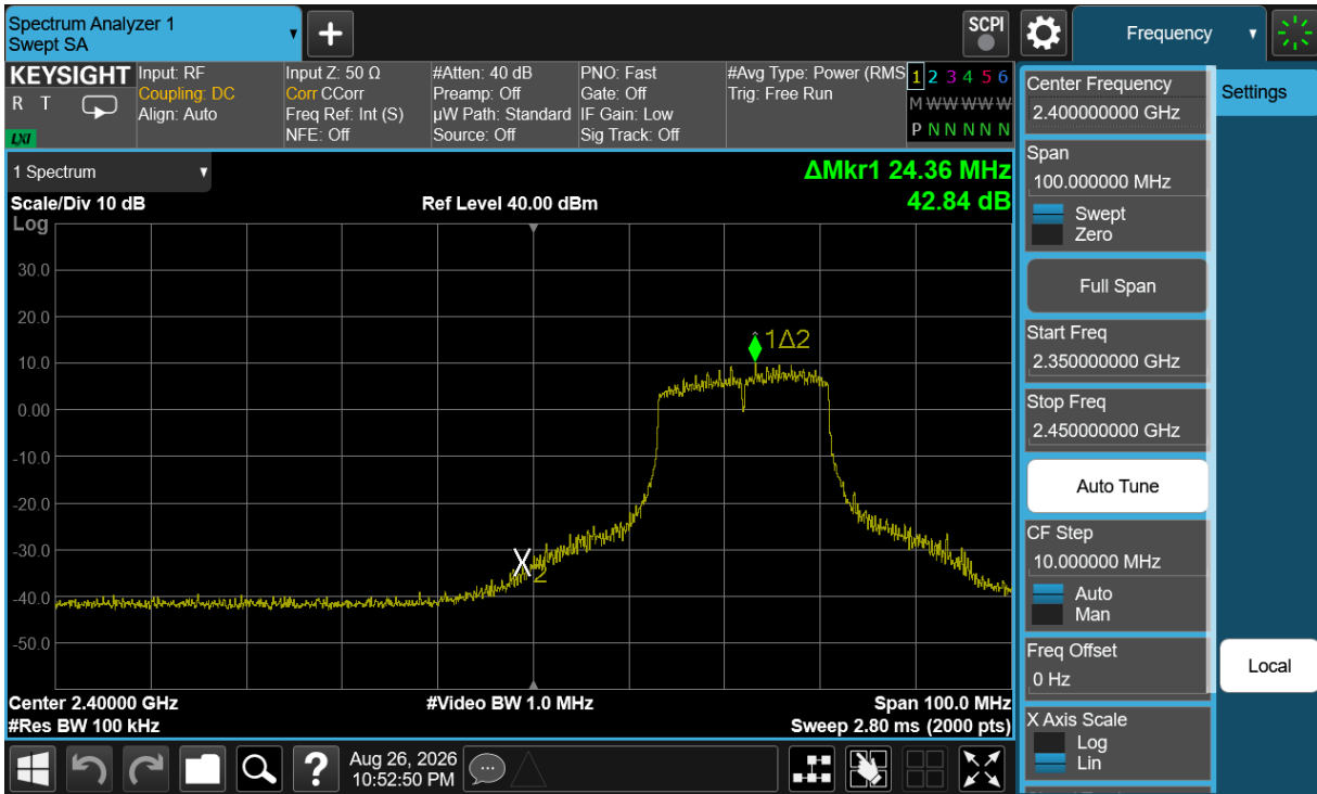
Plot 7-39. Band Edge Plot Antenna 3A (802.11g – Ch. 3)
