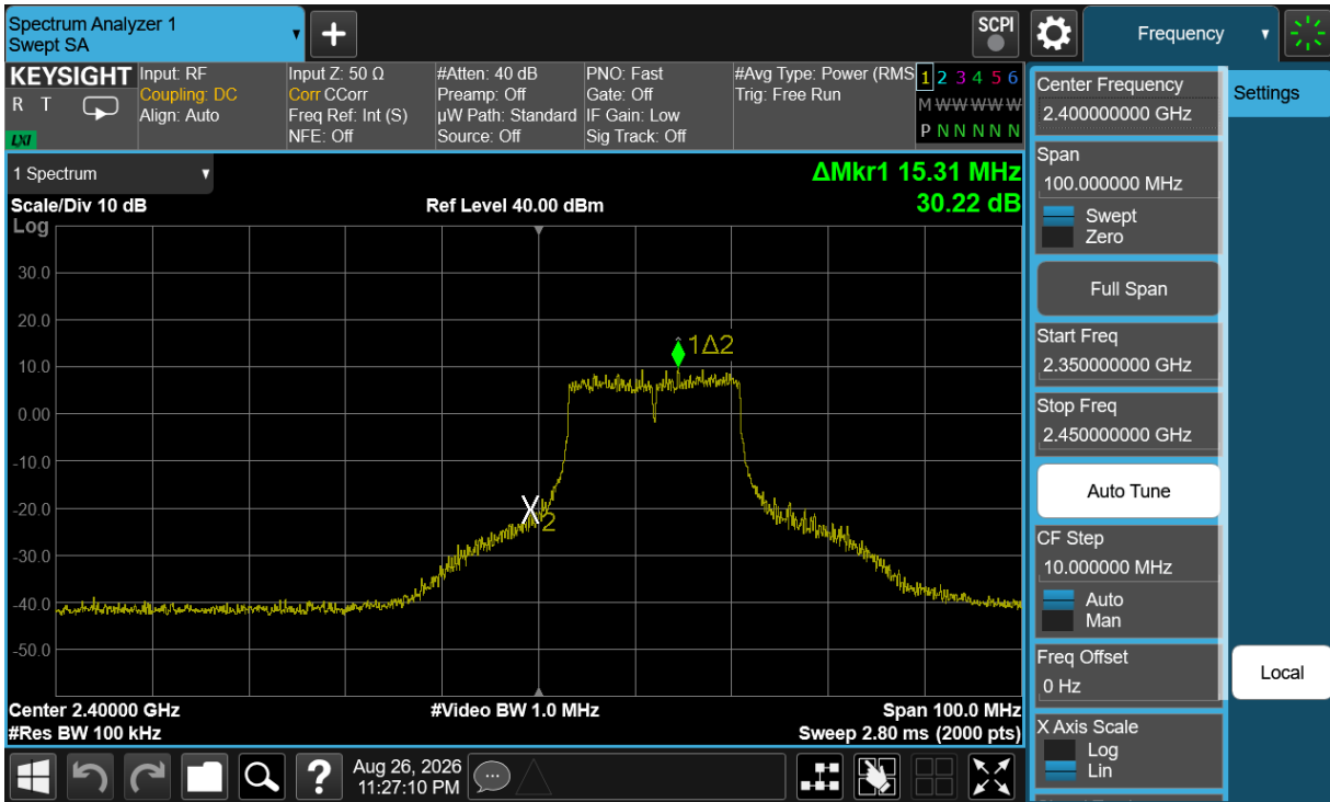
Plot 7-51. Band Edge Plot Antenna 3A (802.11n (2.4 GHz) – Ch. 1)
