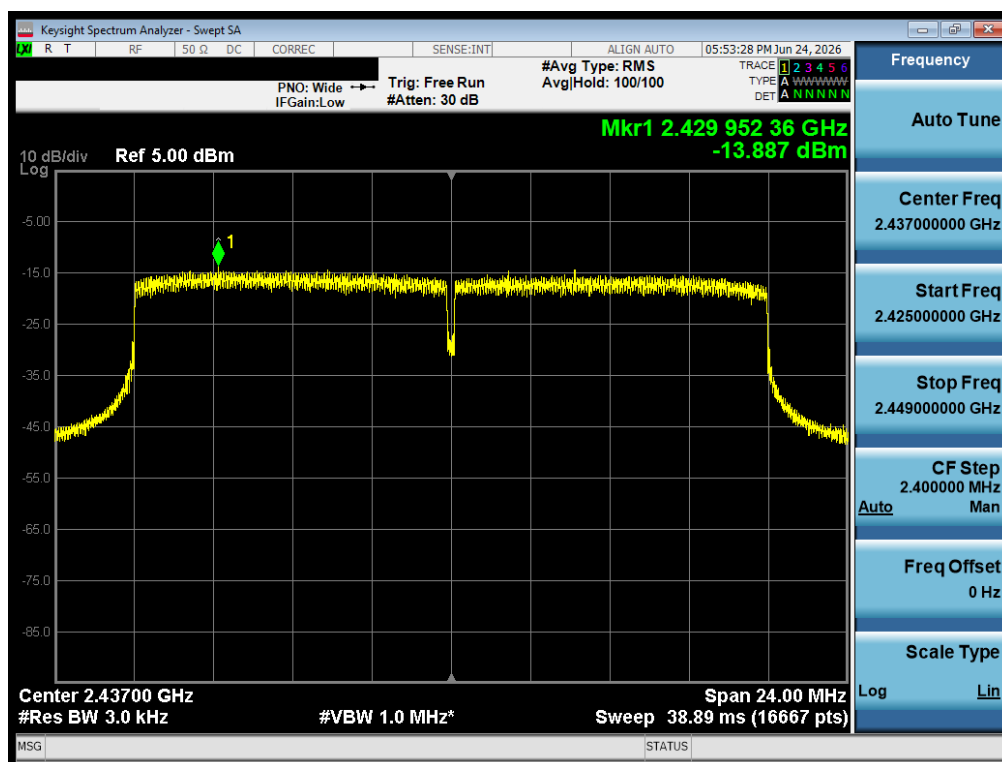
Plot 7-24 PSD Antenna 1A (20 MHz BW 802.11be(SU) - Ch.6)
