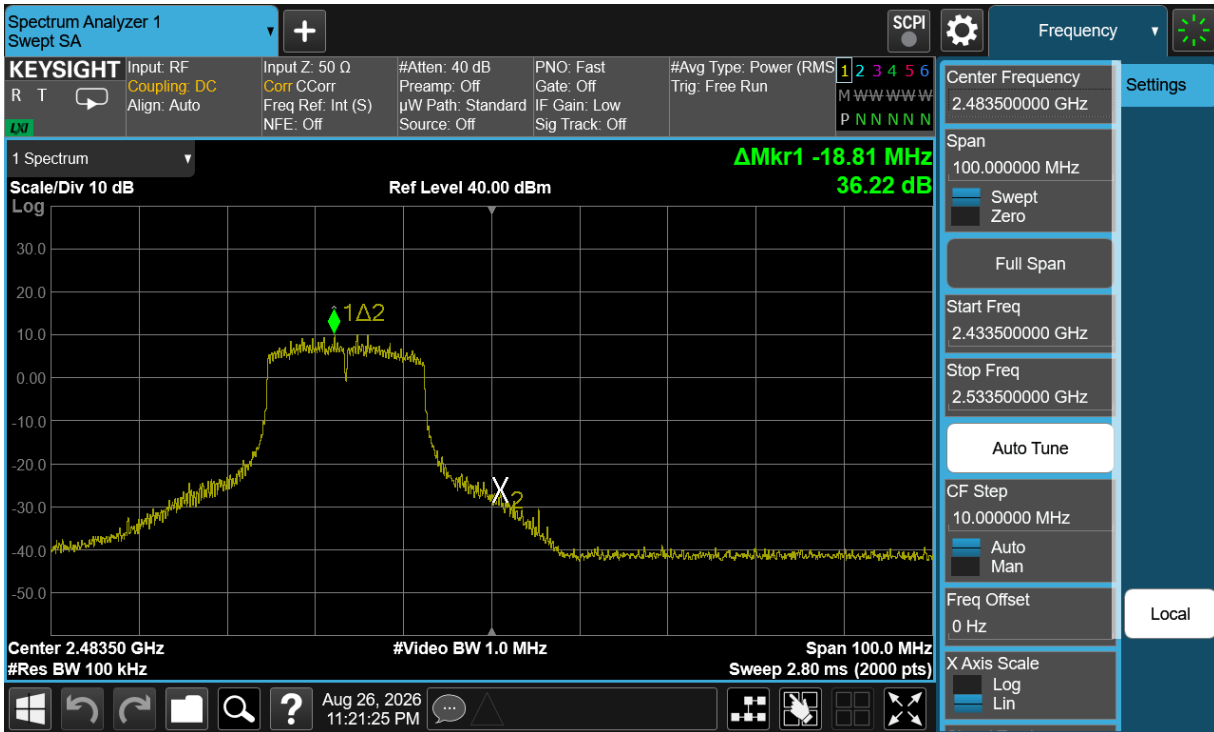
Plot 7-49. Band Edge Plot Antenna 3A (802.11g - Ch. 12)
