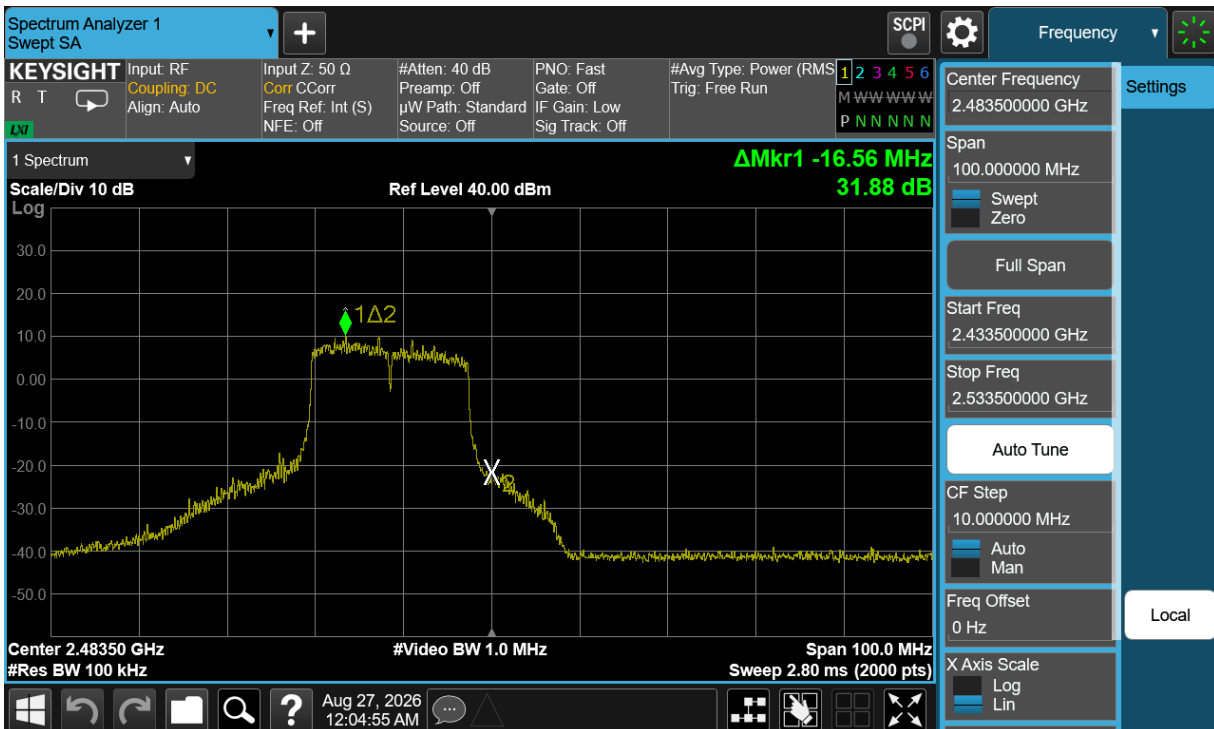
Plot 7-64. Band Edge Plot Antenna 3A (802.11n (2.4 GHz) – Ch. 13)
