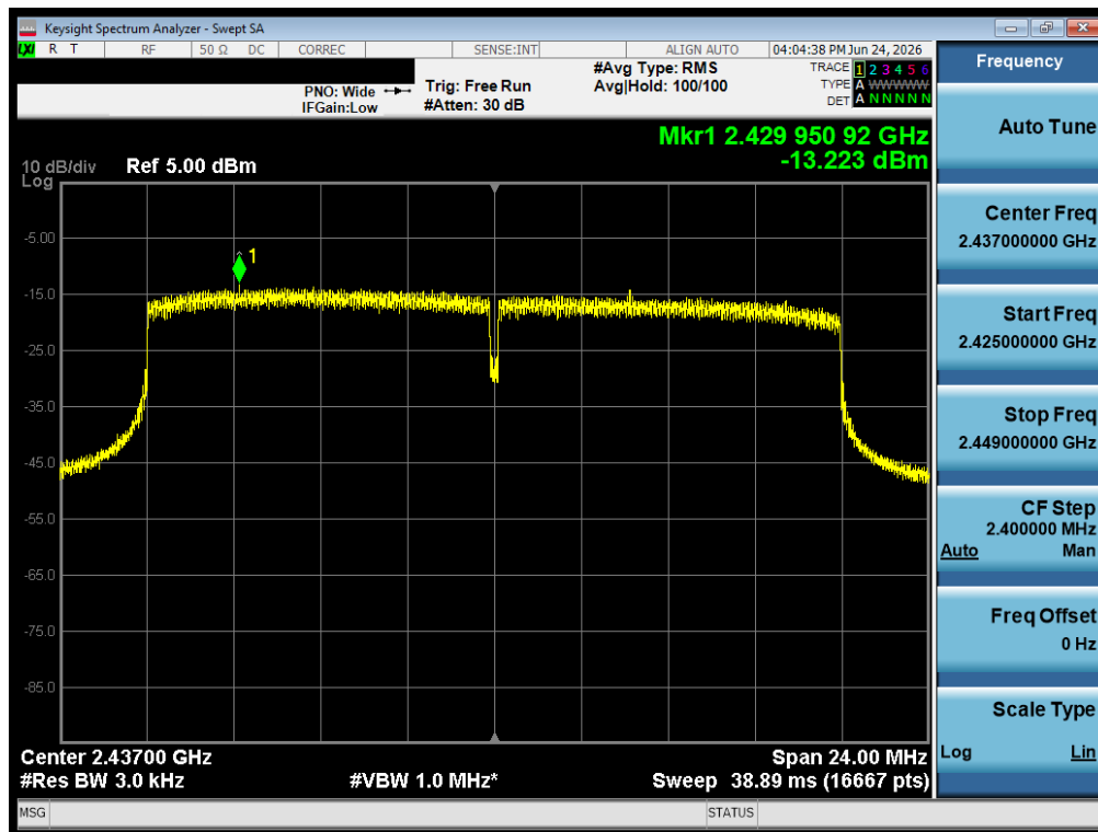
Plot 7-20 PSD Antenna 3A (20 MHz BW 802.11be(SU) - Ch.6)
