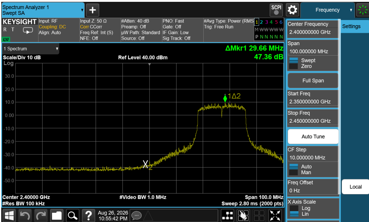
Plot 7-40. Band Edge Plot Antenna 3A (802.11g – Ch. 4)
