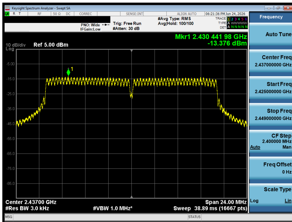
Plot 7-30 PSD CDD Antenna 1A (20 MHz BW 802.11g - Ch.6)
