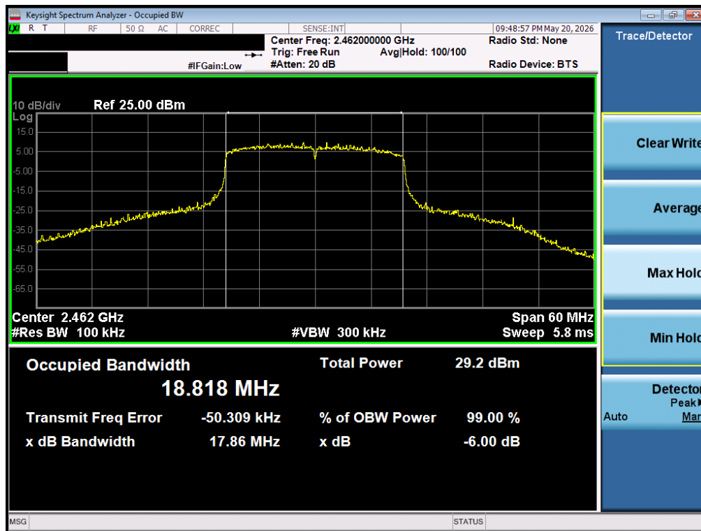
Plot 7-16 6 dB BW Antenna 1A (20 MHz BW 802.11be(SU) - Ch.11)
