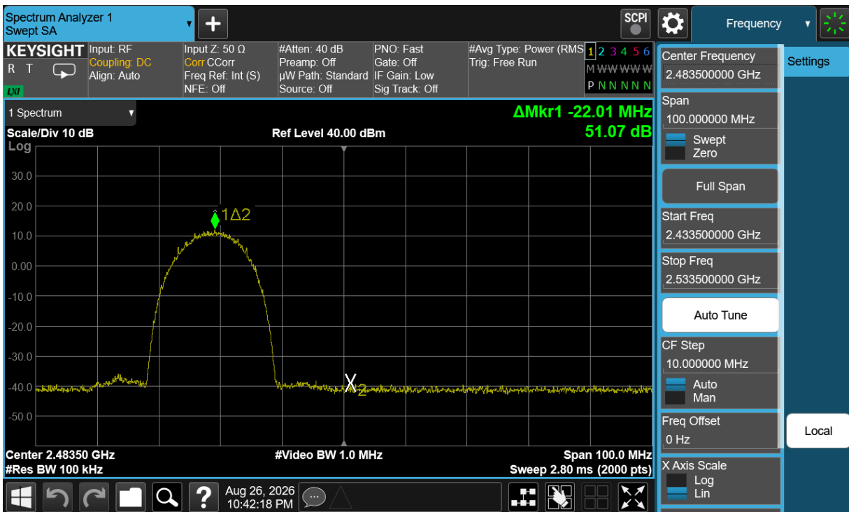
Plot 7-34. Band Edge Plot Antenna 3A (802.11b – Ch. 11)
