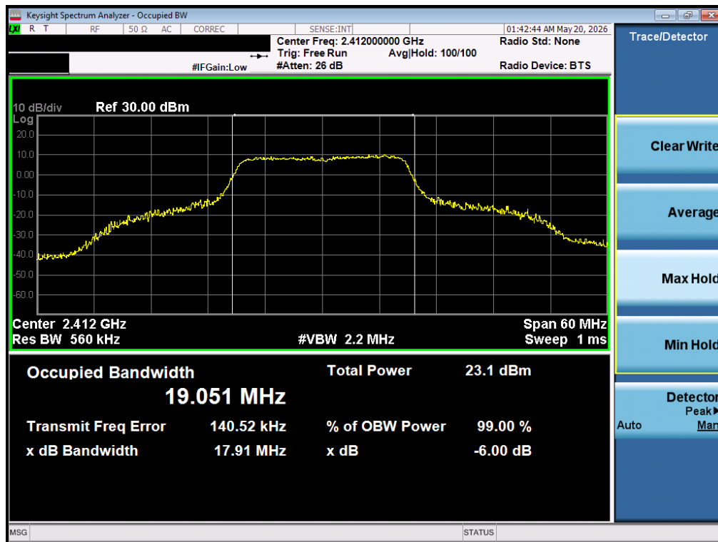
Plot 7-2 99% OBW Antenna 3A (20 MHz BW 802.11g - Ch.1)
