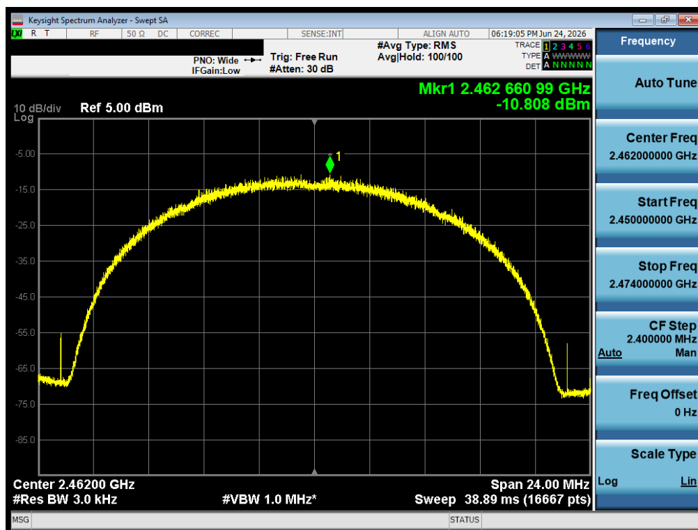
Plot 7-29 PSD CDD Antenna 1A (20 MHz BW 802.11b - Ch.11)
