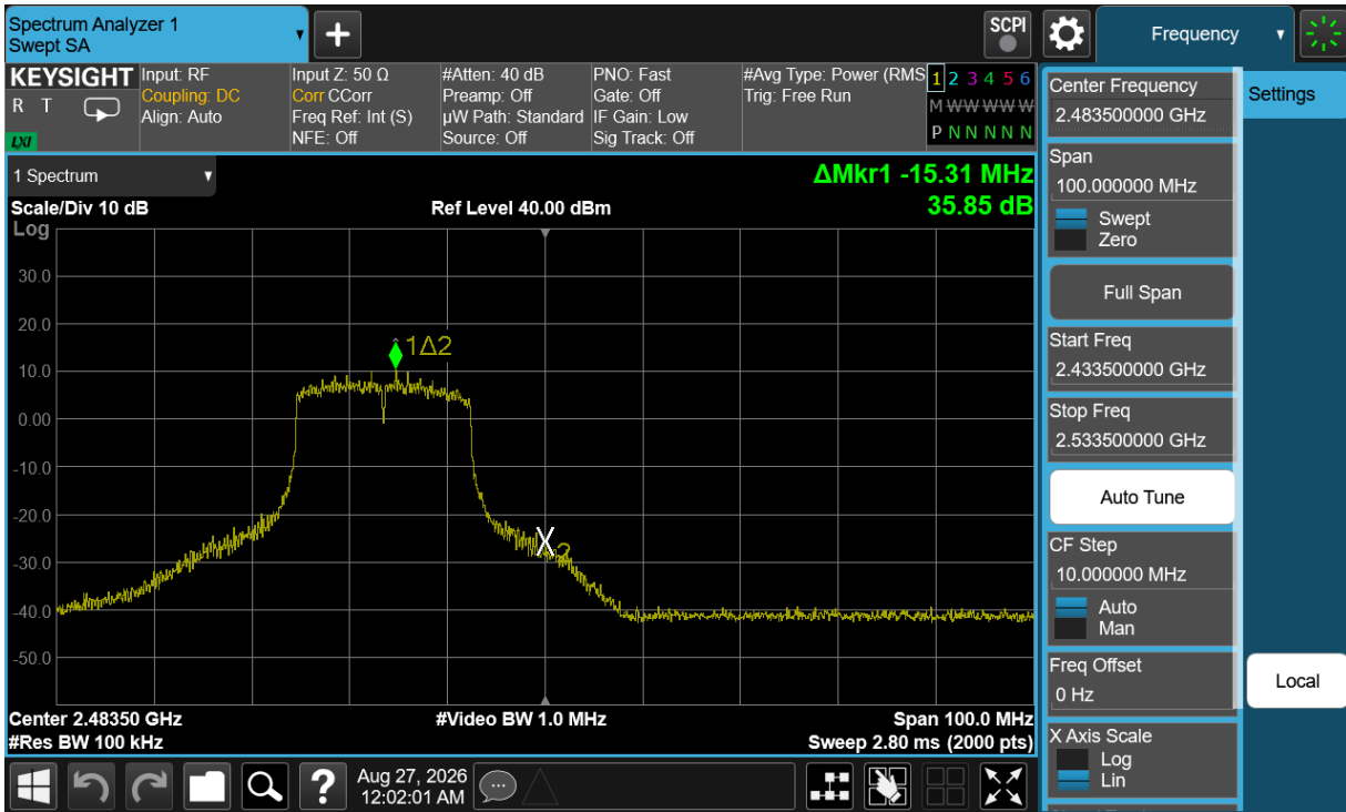
Plot 7-63. Band Edge Plot Antenna 3A (802.11n (2.4 GHz) – Ch. 12)
