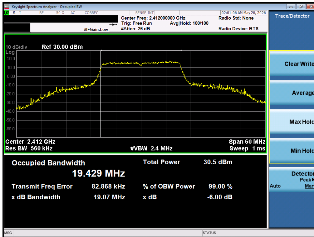
Plot 7-4 99% OBW Antenna 3A (20 MHz BW 7802.11be(SU) - Ch.1)
