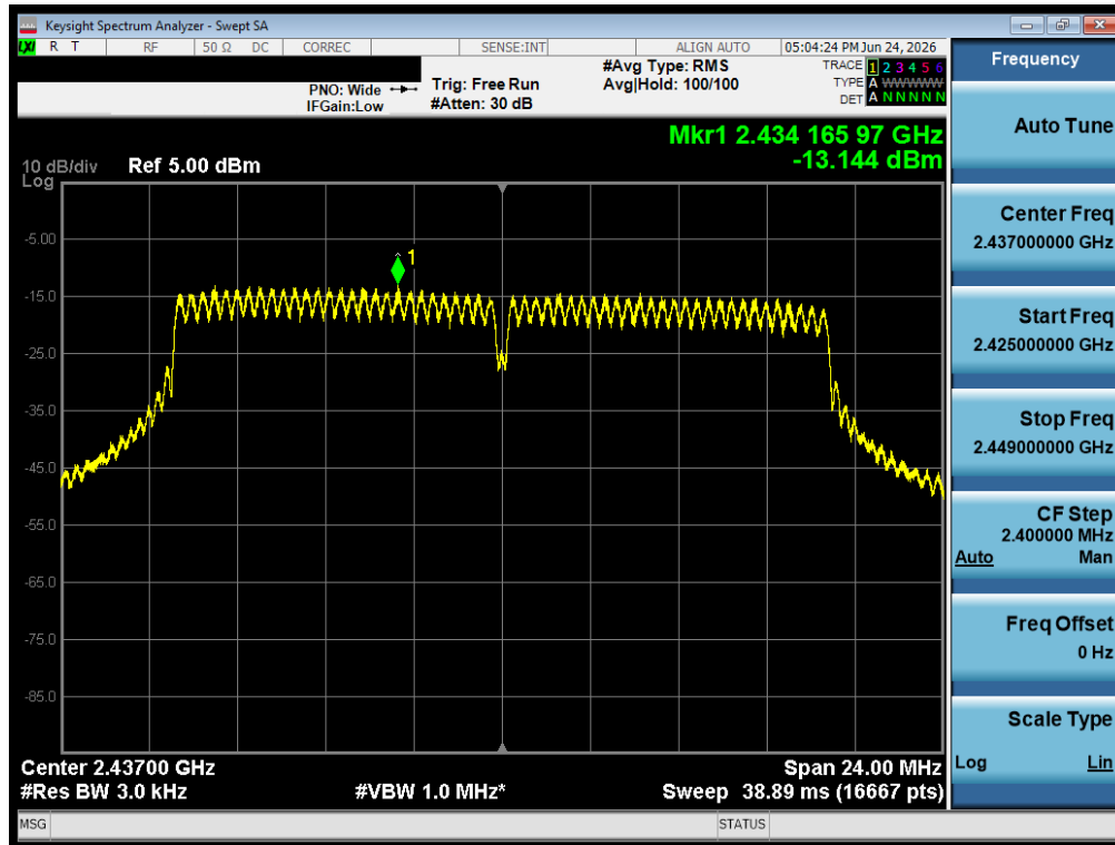
Plot 7-27 PSD CDD Antenna 3A (20 MHz BW 802.11n - Ch.6)
