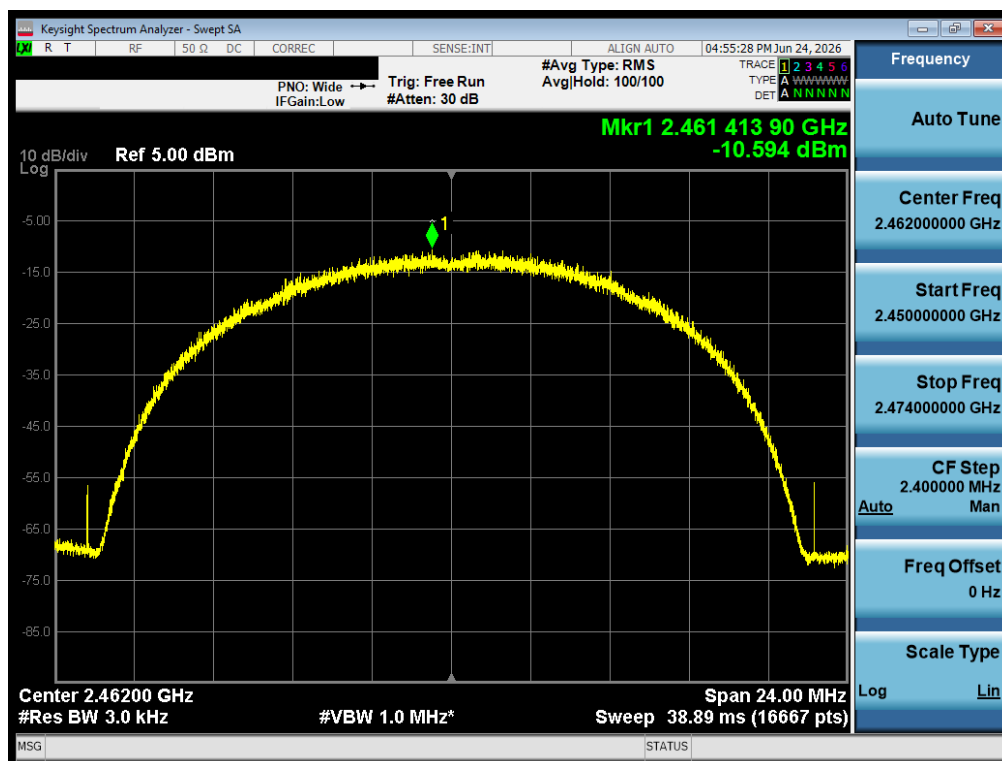
Plot 7-25 PSD CDD Antenna 3A (20 MHz BW 802.11b - Ch.11)
