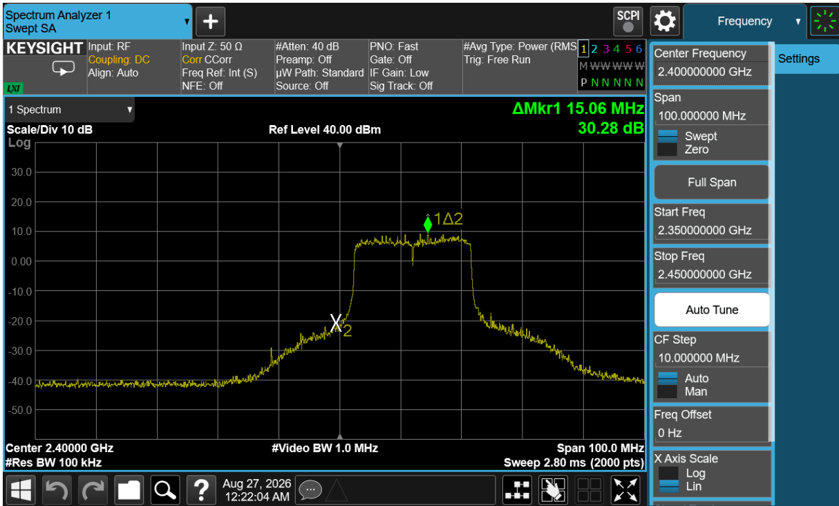
Plot 7-65. Band Edge Plot Antenna 3A (802.11be (SU - 2.4 GHz) – Ch. 1)
