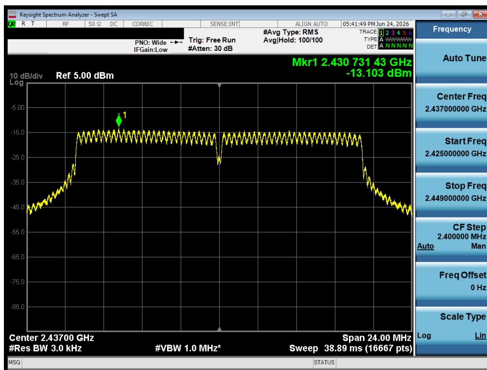
Plot 7-22 PSD Antenna 1A (20 MHz BW 802.11g - Ch.6)
