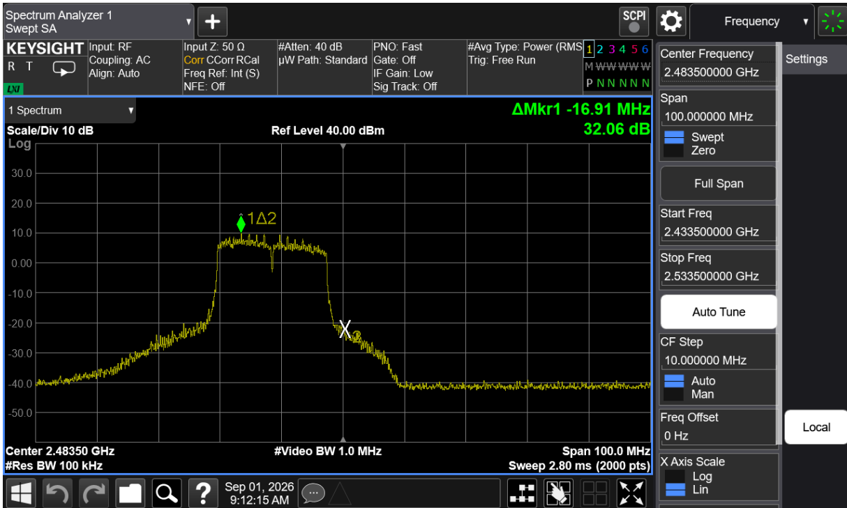
Plot 7-50. Band Edge Plot Antenna 3A (802.11g - Ch. 13)
