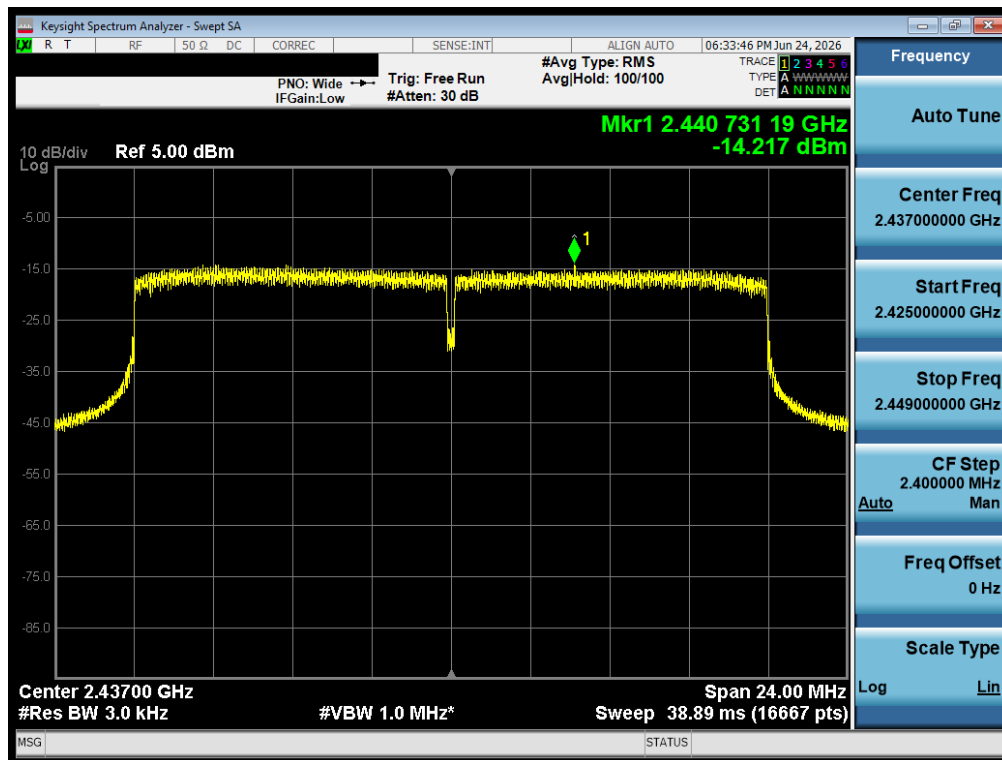
Plot 7-32 PSD CDD Antenna 1A (20 MHz BW 802.11be(SU) - Ch.6)
