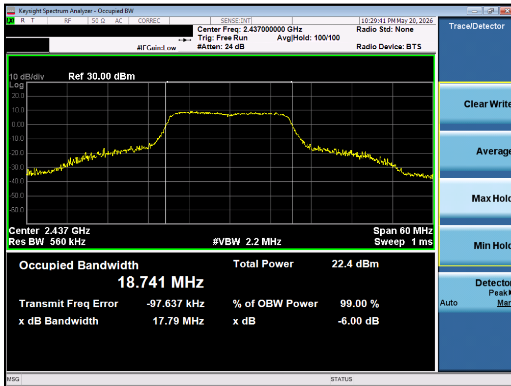
Plot 7-6 99% OBW Antenna 1A (20 MHz BW 802.11g - Ch.6)
