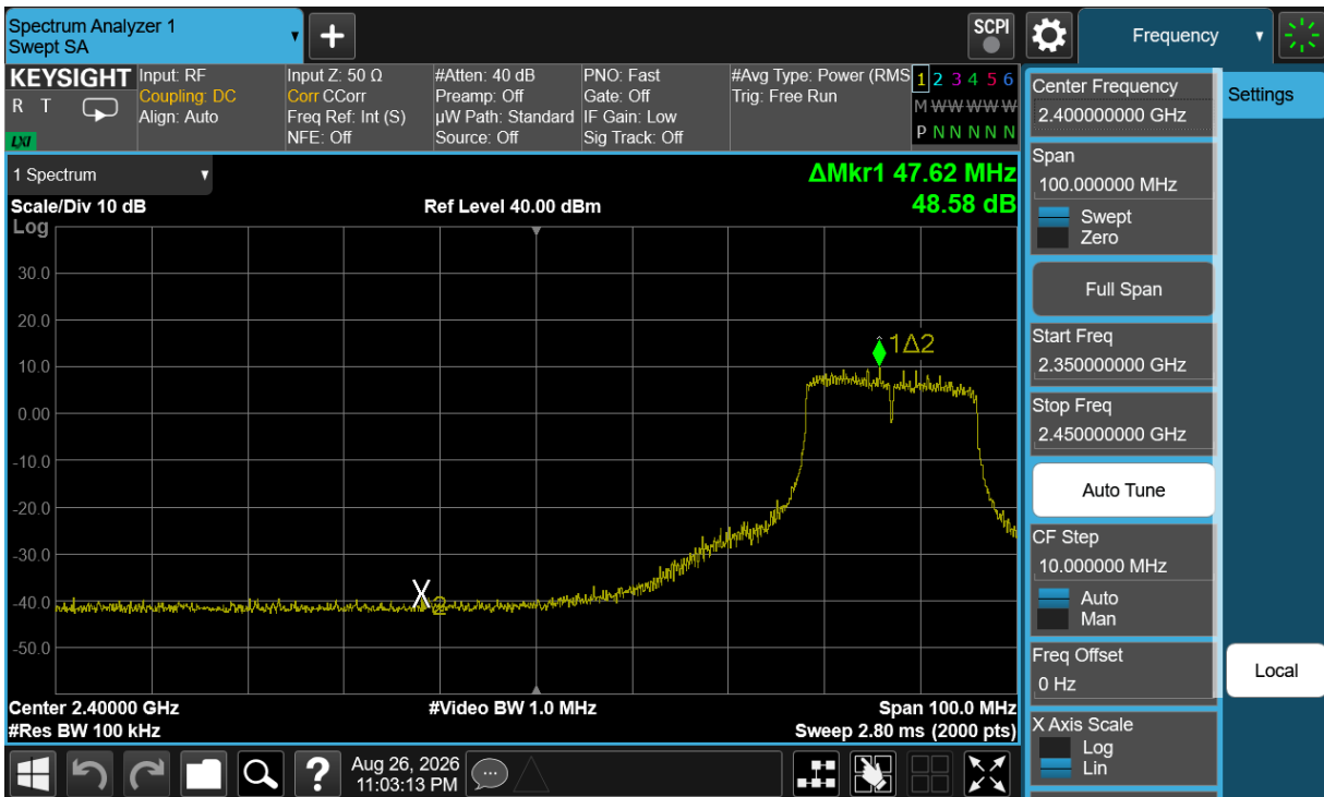
Plot 7-42. Band Edge Plot Antenna 3A (802.11g – Ch. 6)
