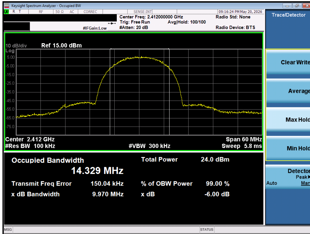
Plot 7-13 6 dB BW Antenna 1A (20 MHz BW 802.11b - Ch.1)
