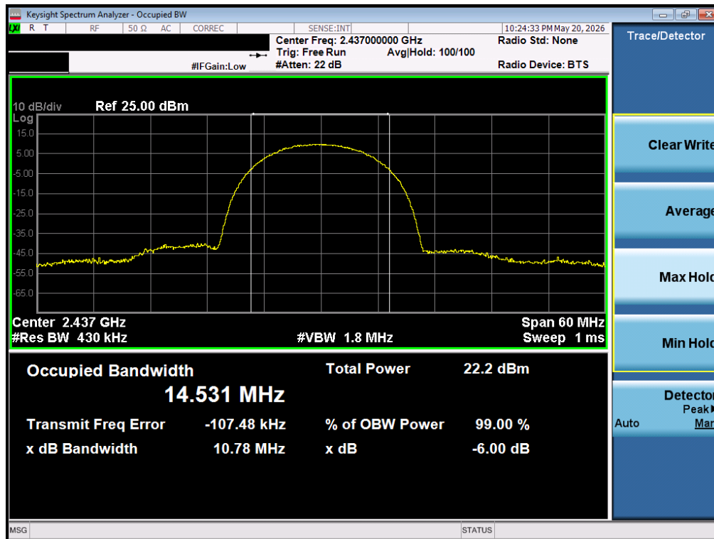
Plot 7-5 99% OBW Antenna 1A (20 MHz BW 802.11b - Ch.6)
