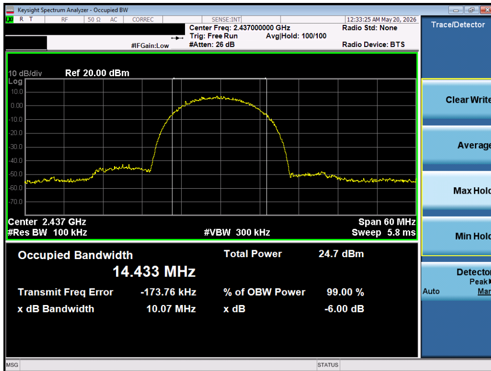
Plot 7-9 6 dB BW Antenna 3A (20 MHz BW 802.11b - Ch.6)
