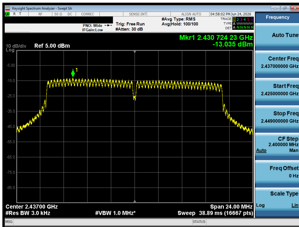
Plot 7-26 PSD CDD Antenna 3A (20 MHz BW 802.11g - Ch.6)
