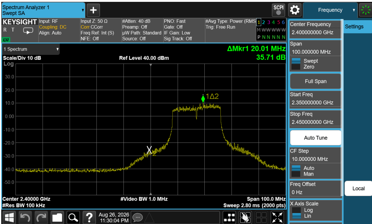
Plot 7-52. Band Edge Plot Antenna 3A (802.11n (2.4 GHz) – Ch. 2)
