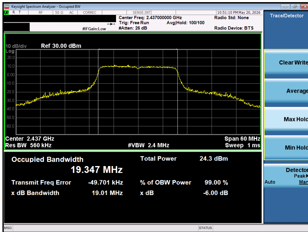
Plot 7-8 99% OBW Antenna 1A (20 MHz BW 802.11be(SU) - Ch.6)
