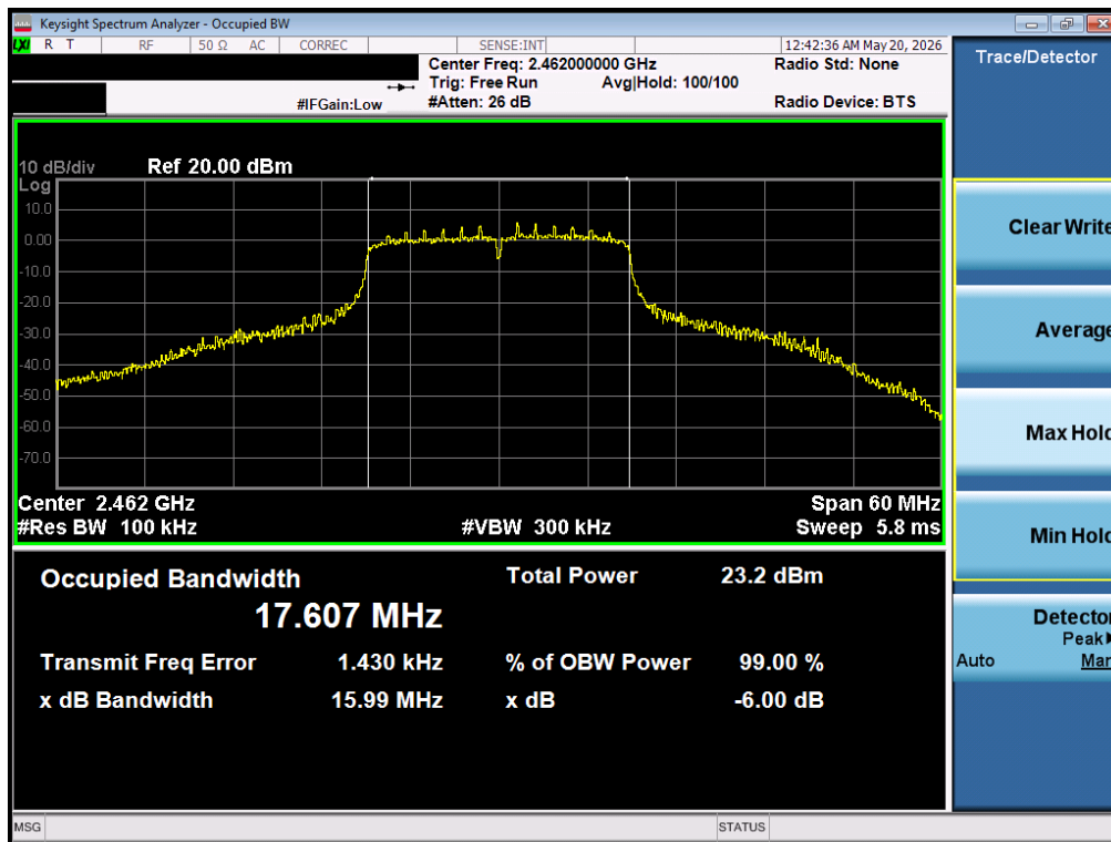
Plot 7-10 6 dB BW Antenna 3A (20 MHz BW 802.11g - Ch.11)
