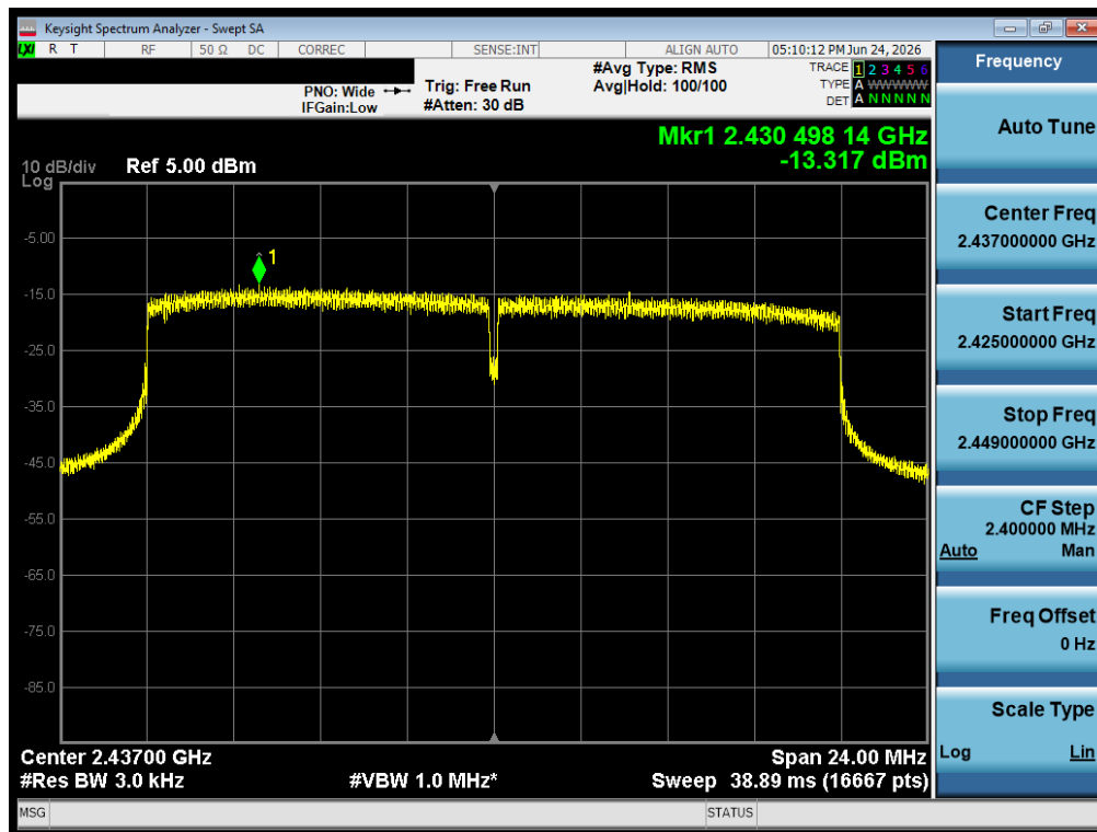
Plot 7-28 PSD CDD Antenna 3A (20 MHz BW 802.11be(SU) - Ch.6)
