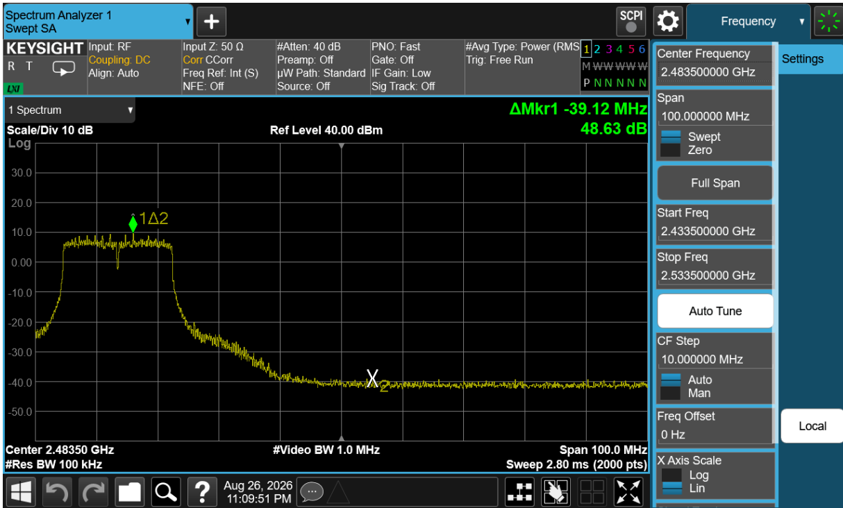
Plot 7-45. Band Edge Plot Antenna 3A (802.11g – Ch. 8)
