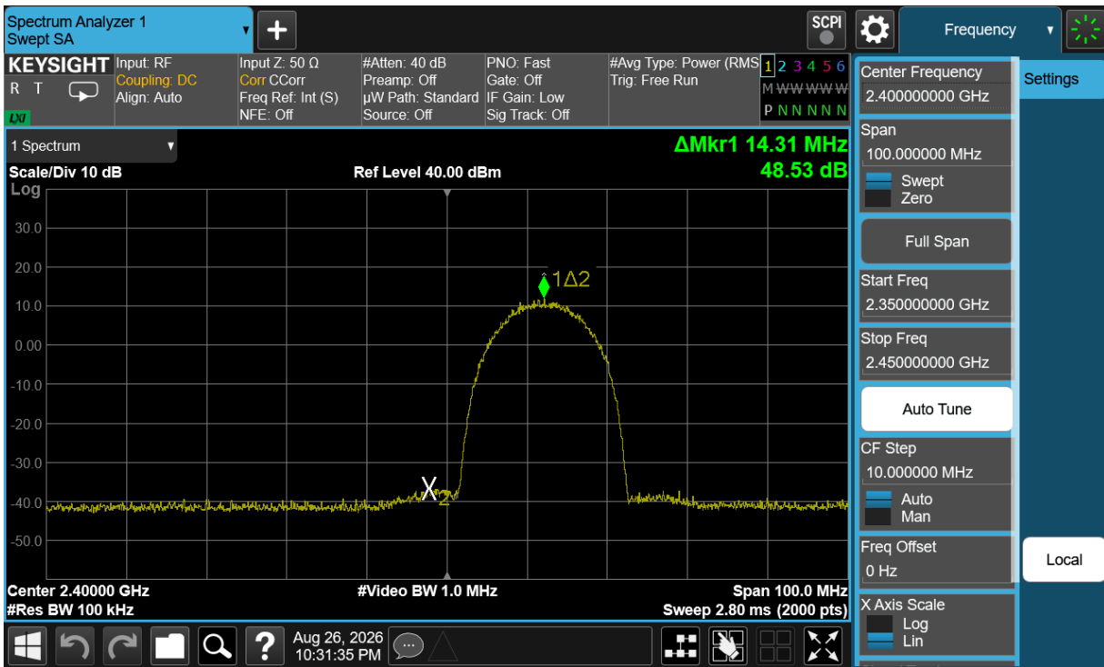
Plot 7-33. Band Edge Plot Antenna 3A (802.11b – Ch. 1)
