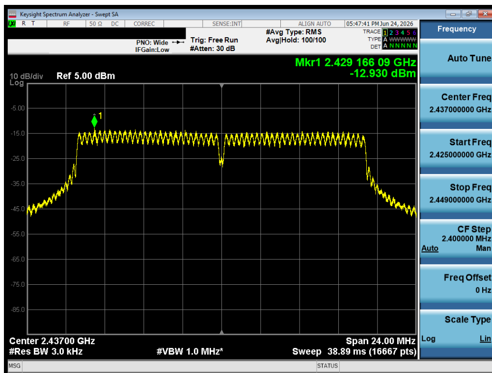
Plot 7-23 PSD Antenna 1A (20 MHz BW 802.11n - Ch.6)
