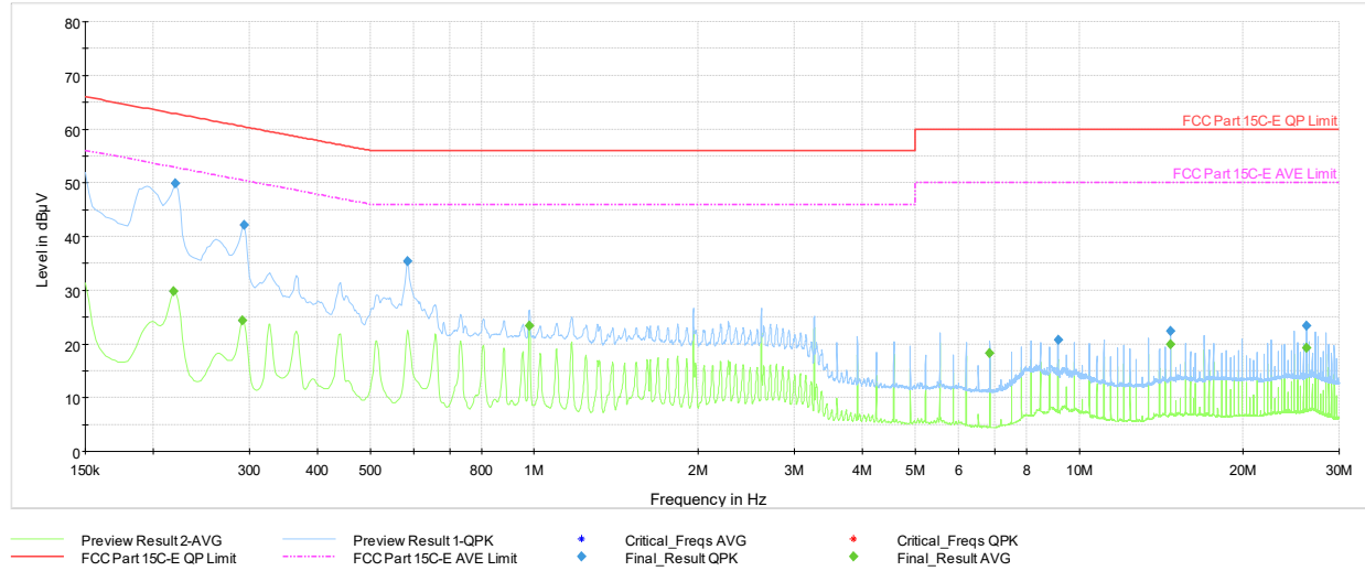
Plot 6-11. AC Line Conducted Plot (L1 - Mode 1, with Host Laptop via USB-C Cable)
