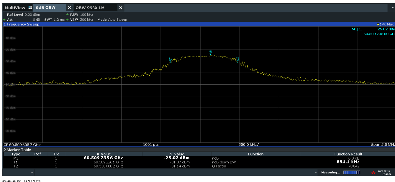
Plot 6-1. 6dB Bandwidth Measurement (Mode 1)
