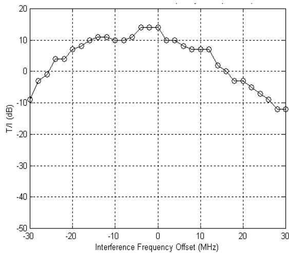
Figure E-10 T/I versus wideband interference frequency offset (Direction A: 05B8, Direction B: 0247)
