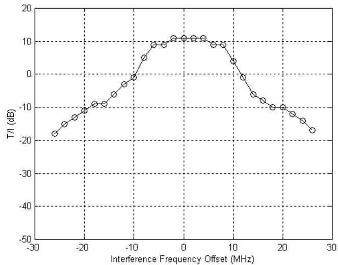
Figure B-10 T/I versus wideband interference frequency offset (Direction A: 1F35, Direction B: 3F0C)
