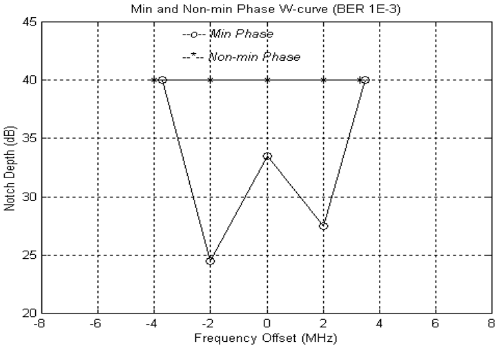
Figure B-4 W Curve at BER = 1E-3, Direction A
