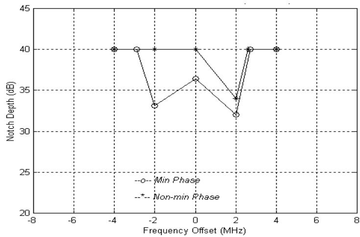
Figure C-4 W Curve at BER = 1E-3, Direction A
