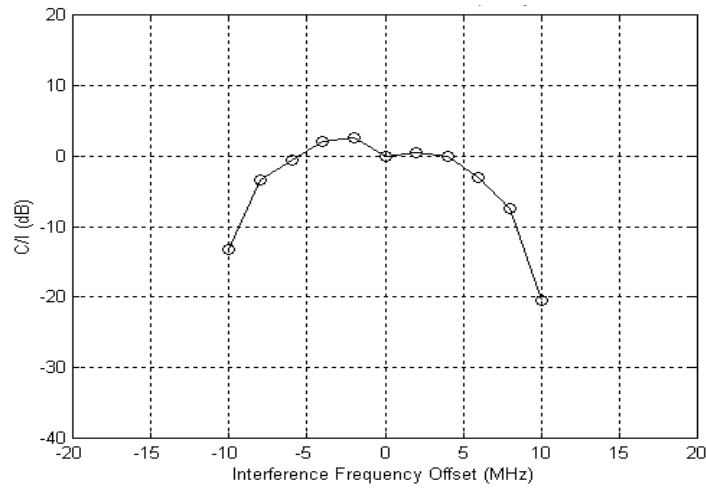
Figure C-8 C/I versus narrowband interference frequency offset
