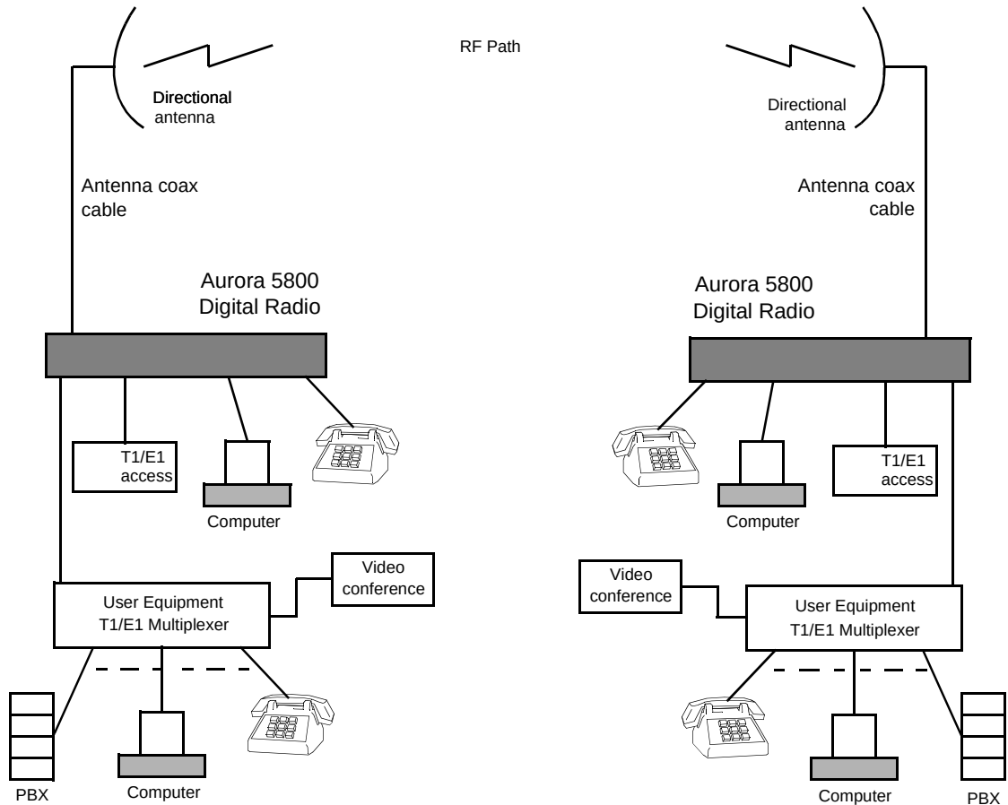
Figure 3-3 Point-to-point configuration
