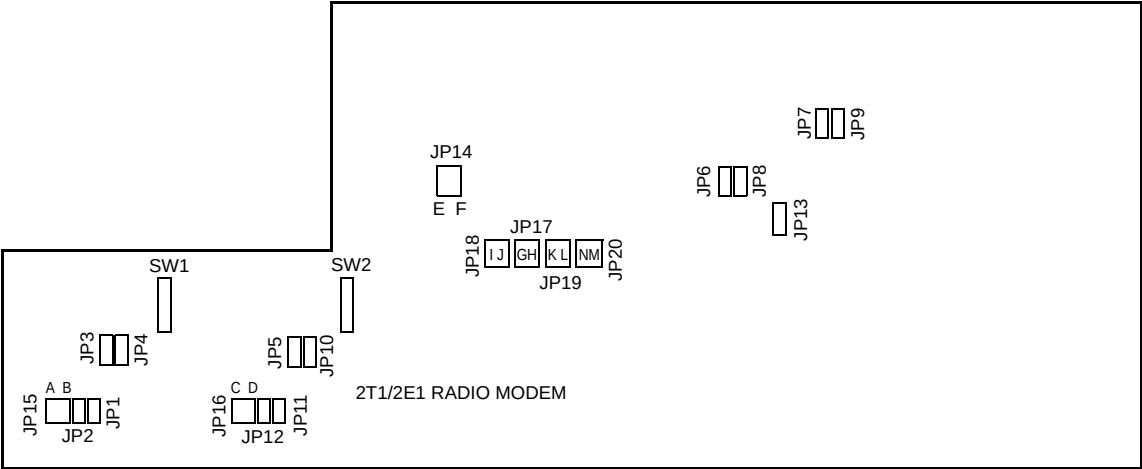
Figure 2-10 Modem, component side
