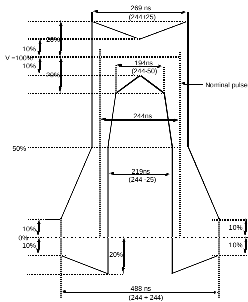
Figure 4-4 Pulse shape
