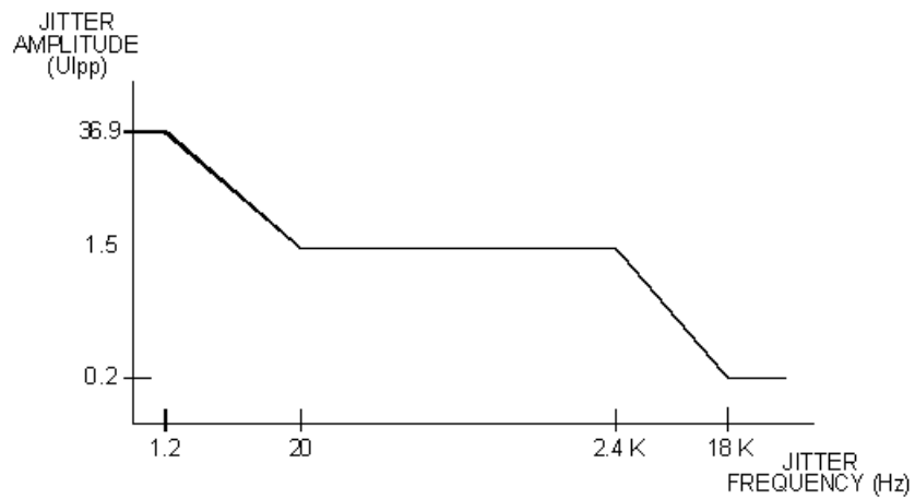
Figure 4-5 Input jitter tolerance
