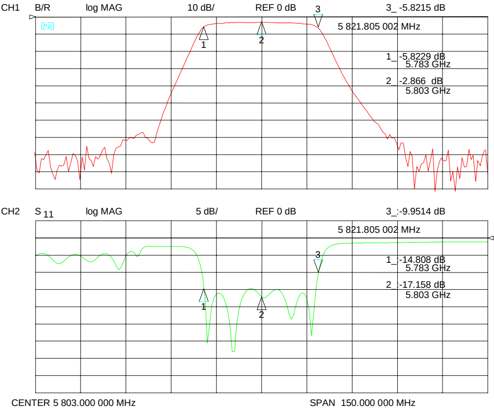
Figure A-9 Filter with center frequency of 5.803 GHz
