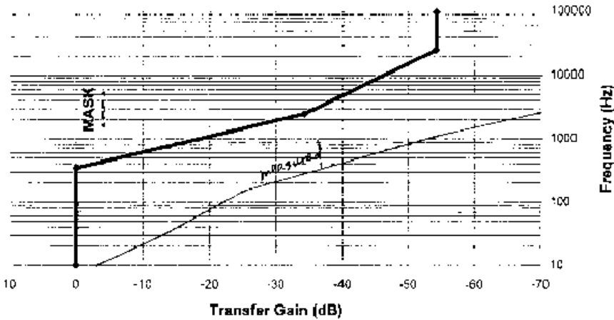
Figure D-13 Jitter transfer (DS1)
