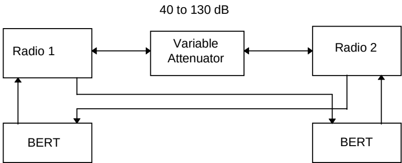
Figure E-2 Receiver test setup
