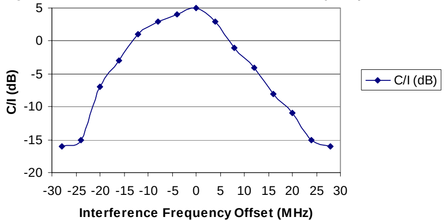
Figure D-11 C/I versus wideband interference frequency offset
