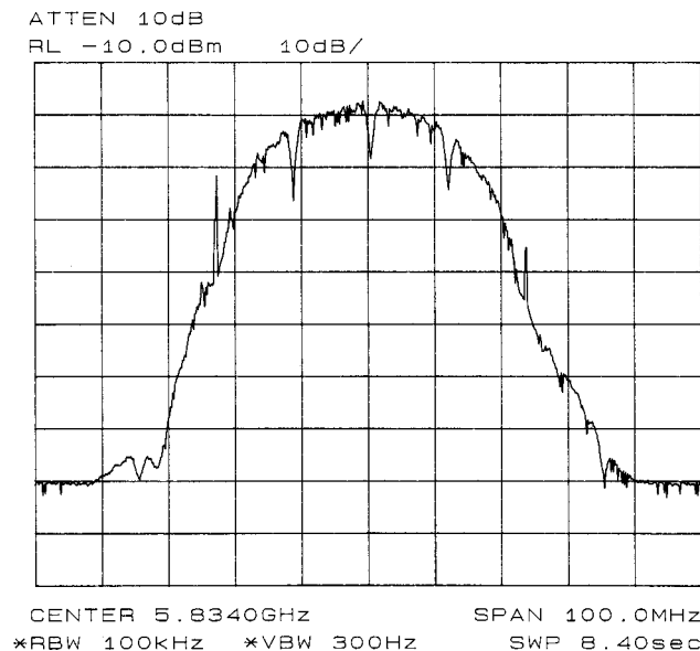
Figure E-1 Transmit RF spectrum
