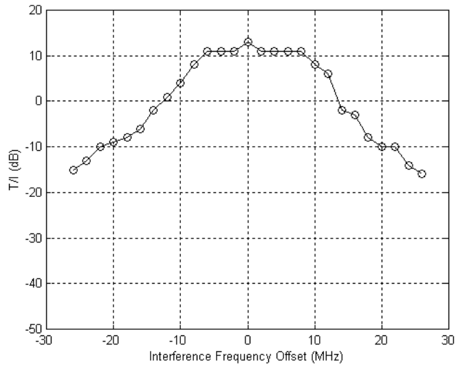
Figure B-9 T/I versus wideband interference frequency offset (Directions A and B, same code, 1F35)
