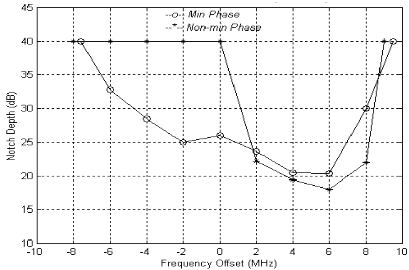
Figure E-3 W Curve at BER=1E-6, Direction A
