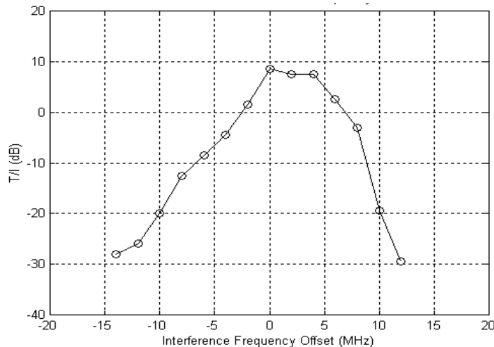
Figure C-7 T/I versus narrowband interference frequency offset
