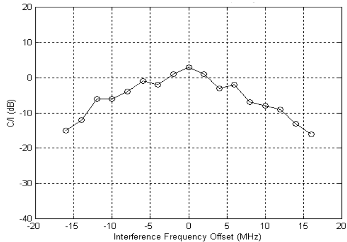
Figure C-11 C/I versus wideband interference frequency offset
