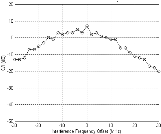
Figure E-11 C/I versus wideband interference frequency offset
