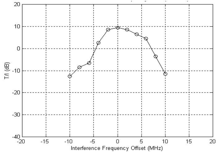
Figure C-10 T/I versus wideband interference frequency offset (Direction A: 05B8, Direction B: 0247)
