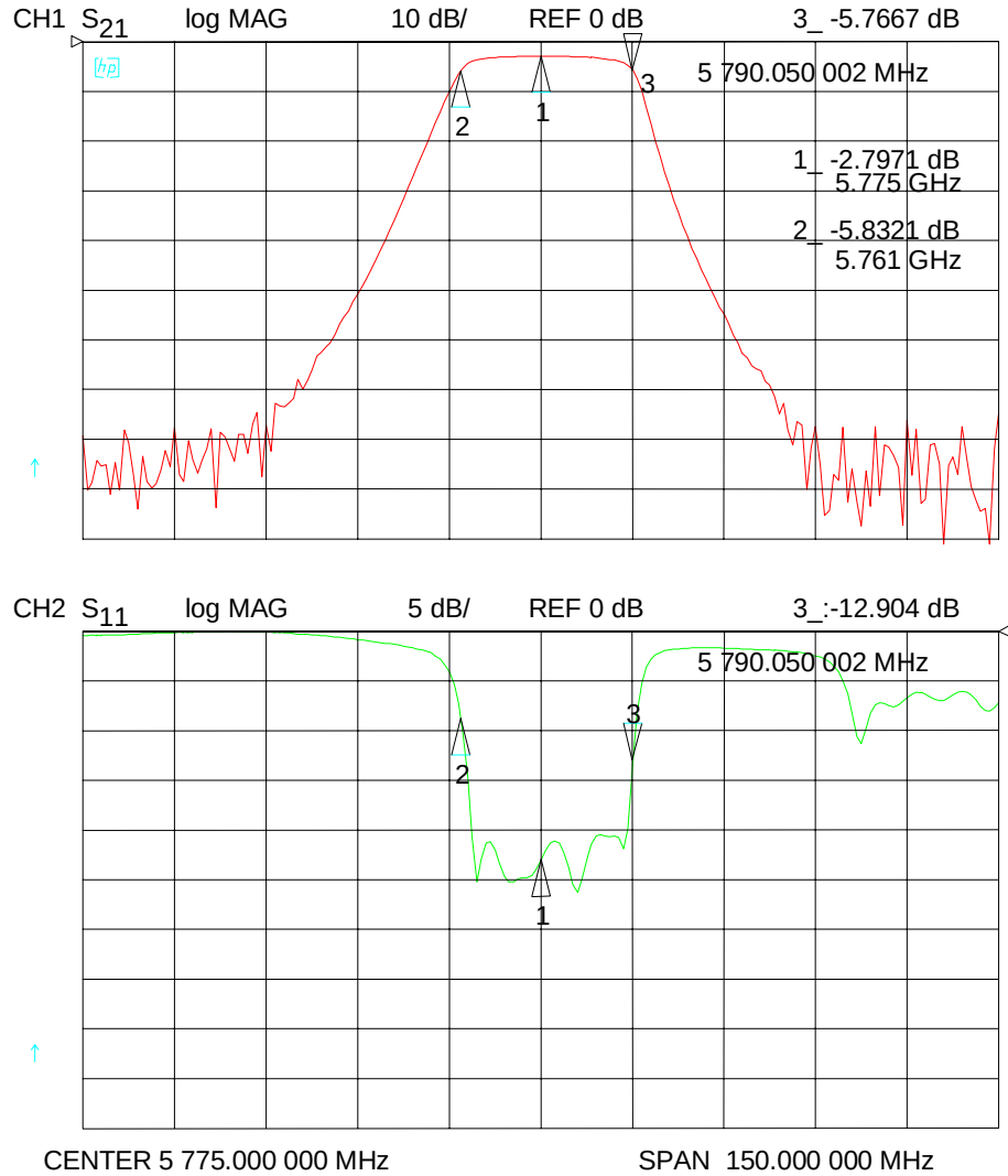
Figure A-3 Filter with center frequency of 5.775 GHz
