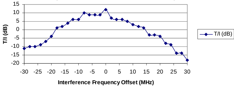
Figure D-9 T/I versus wideband interference frequency offset (Directions A and B, same code, 05B8)
