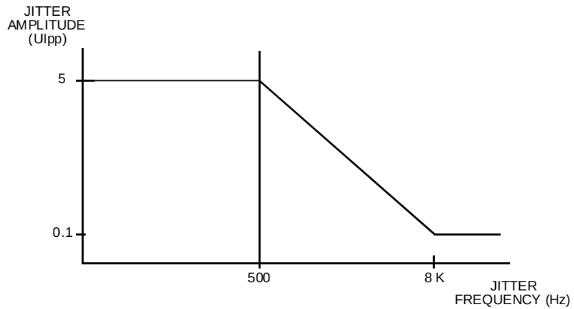
Figure 4-2 Input jitter tolerance
