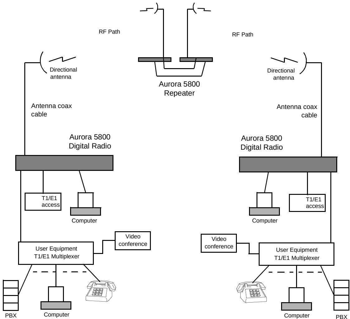
Figure 3-4 Repeater configuration
