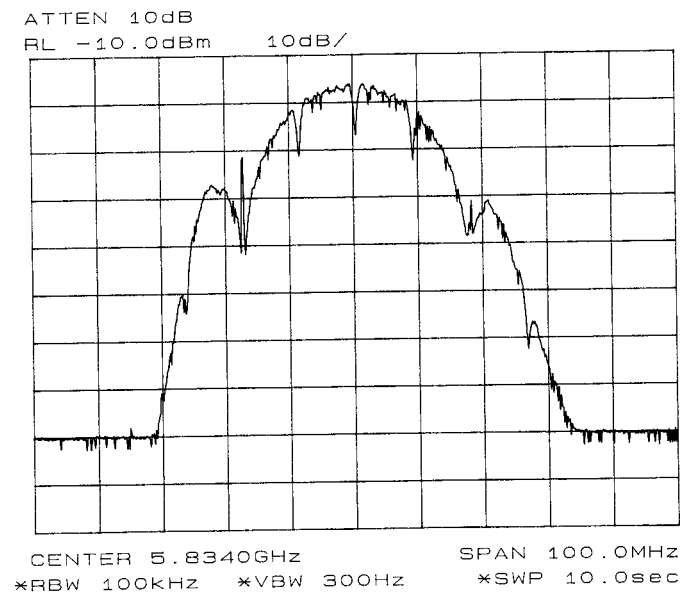
Figure D-1 Transmit RF spectrum
