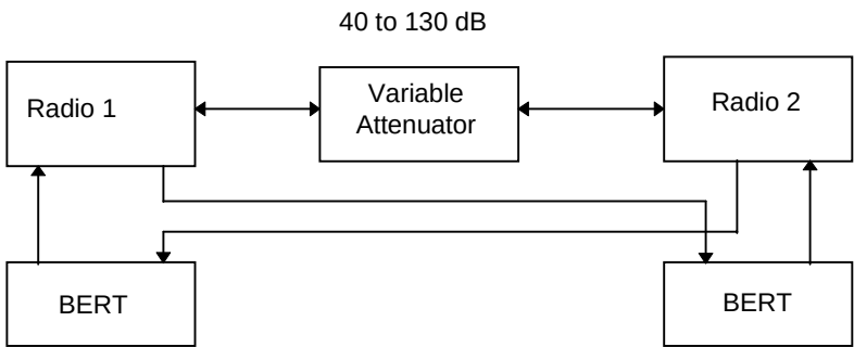
Figure B-2 Receiver test setup
