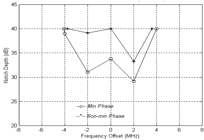
Figure C-5 W Curve at BER = 1E-6, Direction B
