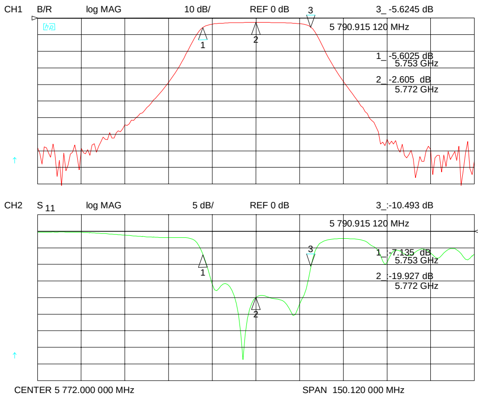
Figure A-8 Filter with center frequency of 5.772 GHz
