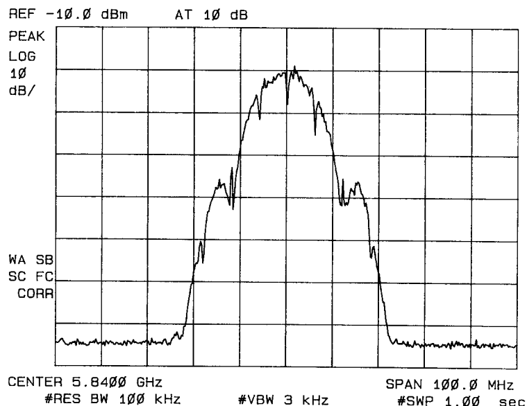
Figure C-1 Transmit RF spectrum
