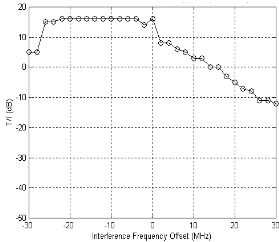
Figure E-9 T/I versus wideband interference frequency offset (Directions A and B, same code, 05B8)
