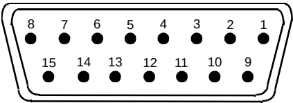
Figure 2-7 DA-15, female
