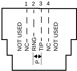
Figure 2-8 RJ-11
