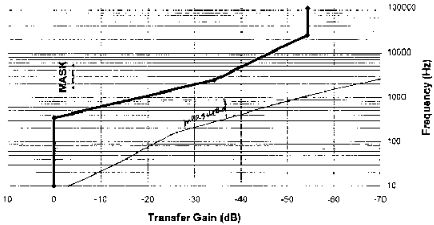
Figure 0-1 Jitter transfer (DS1)
