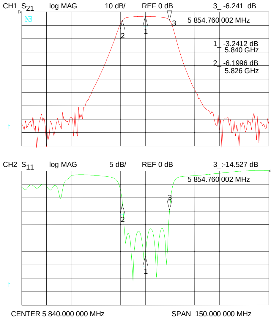
Figure A-6 Filter with center frequency of 5.84 GHz
