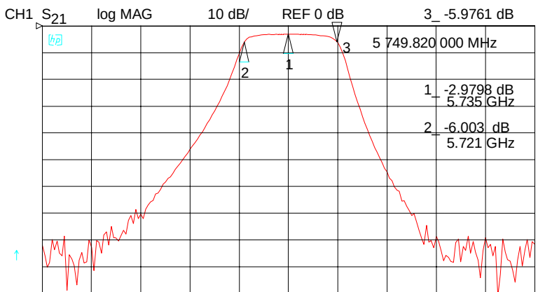
Figure A-1 Filter with center frequency of 5.735 GHz
