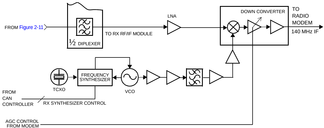
Figure 2-12 Down Converter block diagram
