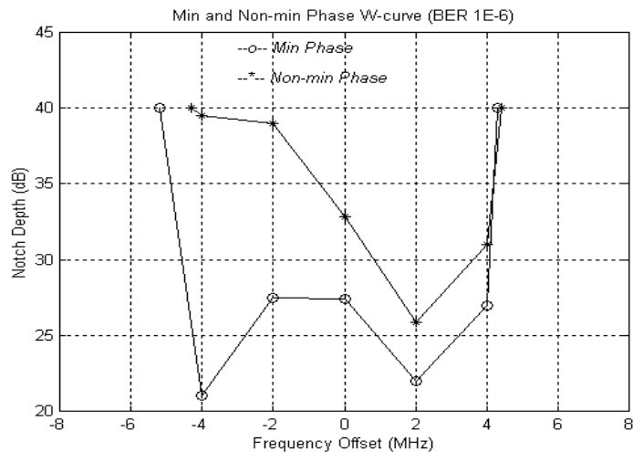
Figure B-5 W Curve at BER = 1E-6, Direction B
