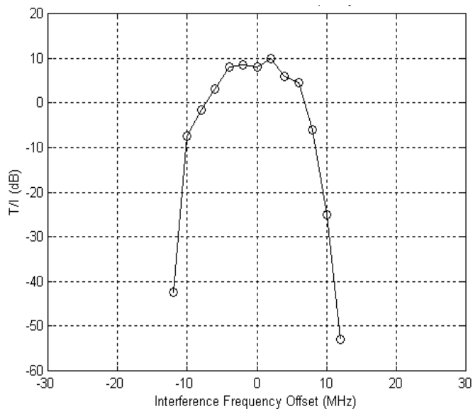
Figure B-7 T/I versus narrowband interference frequency offset
