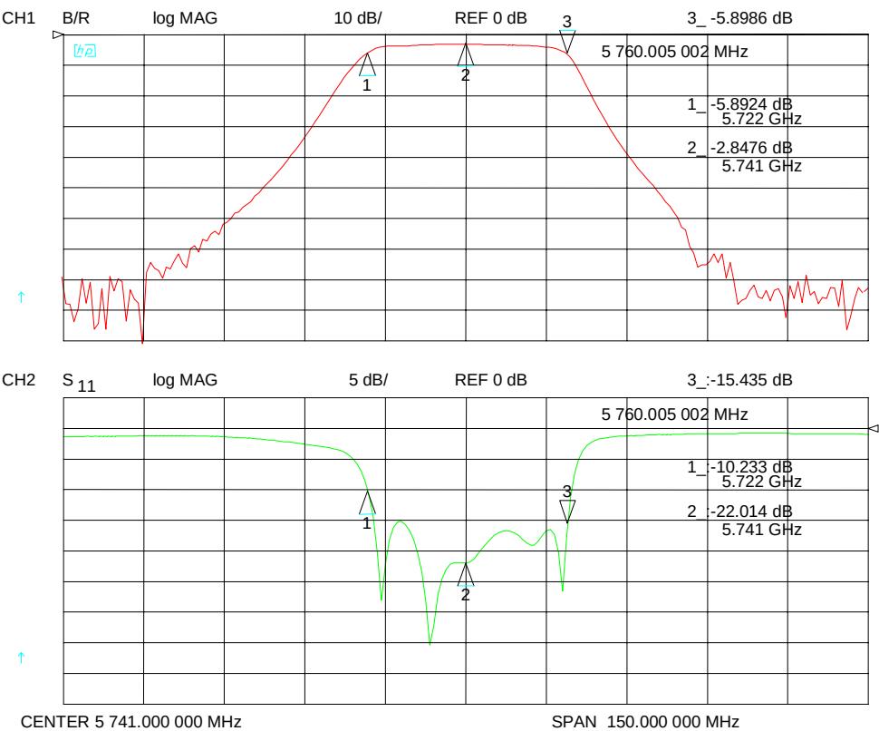
Figure A-7 Filter with center frequency of 5.741 GHz
