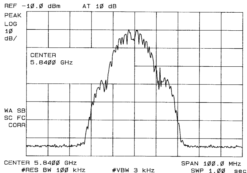
Figure B-1 Transmit RF spectrum
