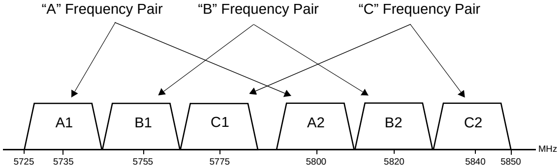
Figure 3-2 Aurora 5800 2T1/2E1 frequency plan
