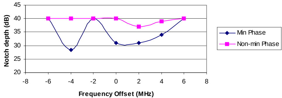
Figure D-5 W Curve at BER=1E-6, Direction B
