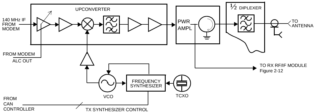
Figure 2-11 Upconverter and Power Amplifier block diagram
