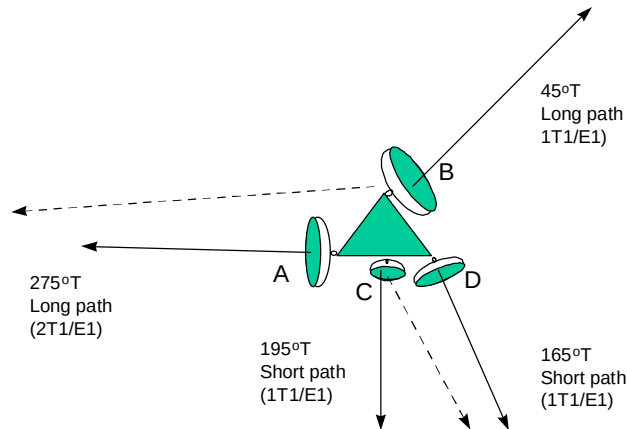
Figure 3-6 Tower mounting with no blockage
