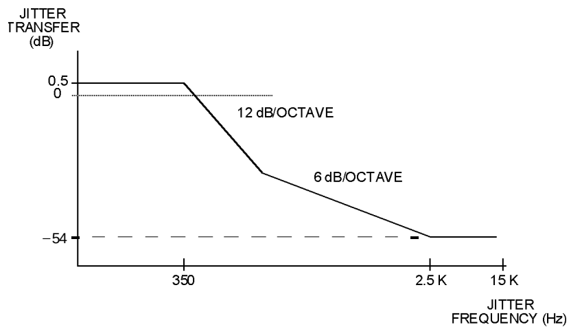
Figure 4-3 Jitter transfer function tolerance
