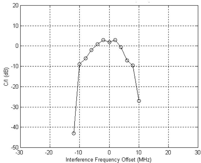
Figure B-8 C/I versus narrowband interference frequency offset
