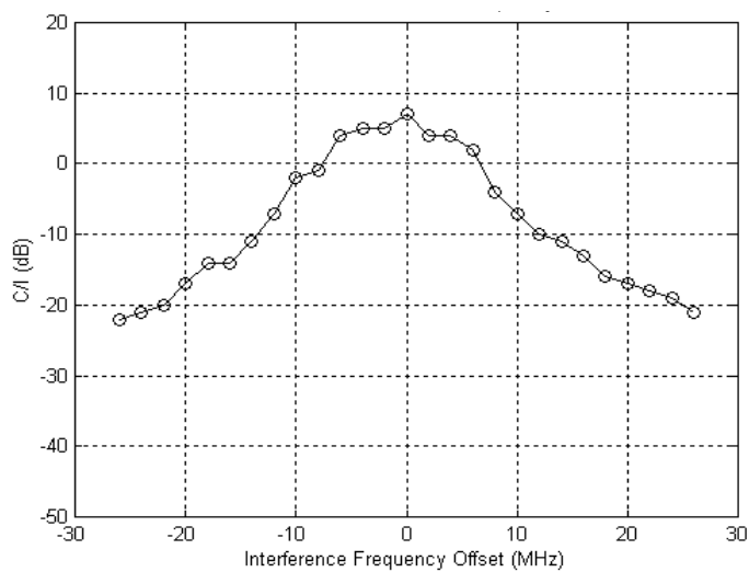
Figure B-11 C/I versus wideband interference frequency offset
