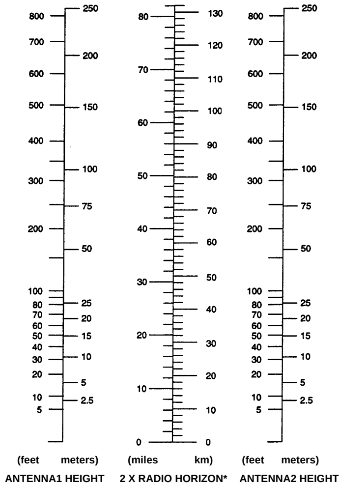
Figure 5-1 Antenna height chart
