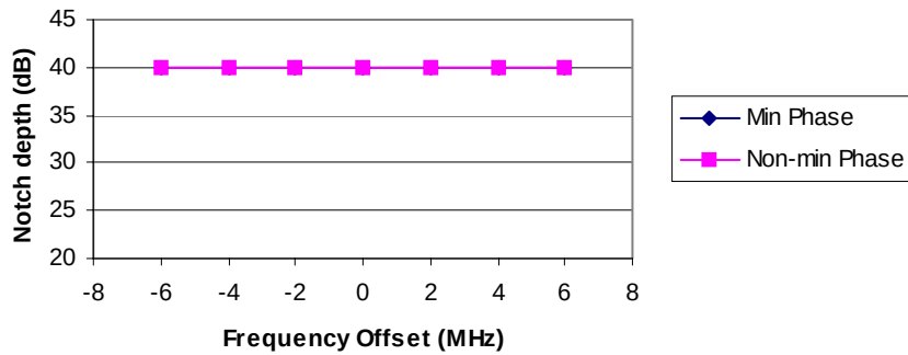
Figure D-4 W Curve at BER=1E-3, Direction A
