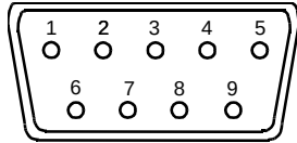
Figure 2-5 Alarm port, RS-232, male
