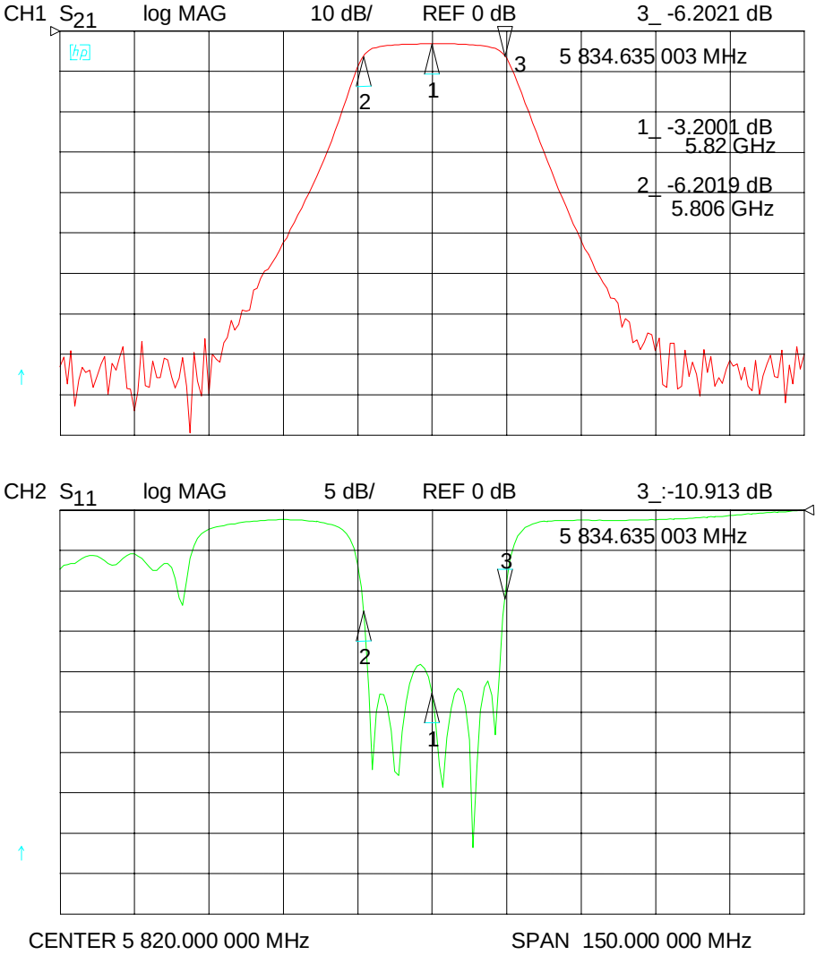
Figure A-5 Filter with center frequency of 5.82 GHz
