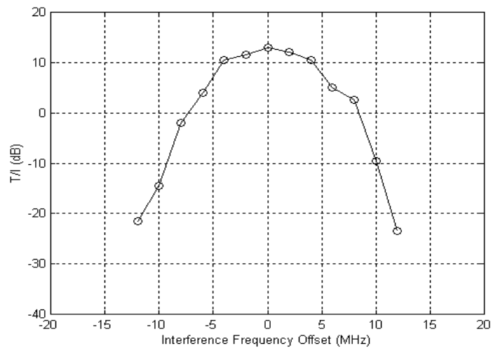
Figure C-9 T/I versus wideband interference frequency offset (Directions A and B, same code, 05B8)
