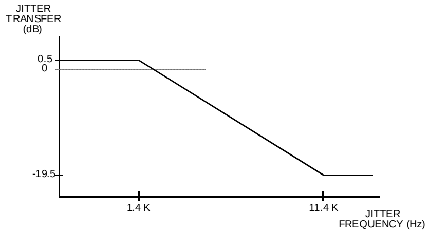
Figure 4-6 Jitter transfer function
