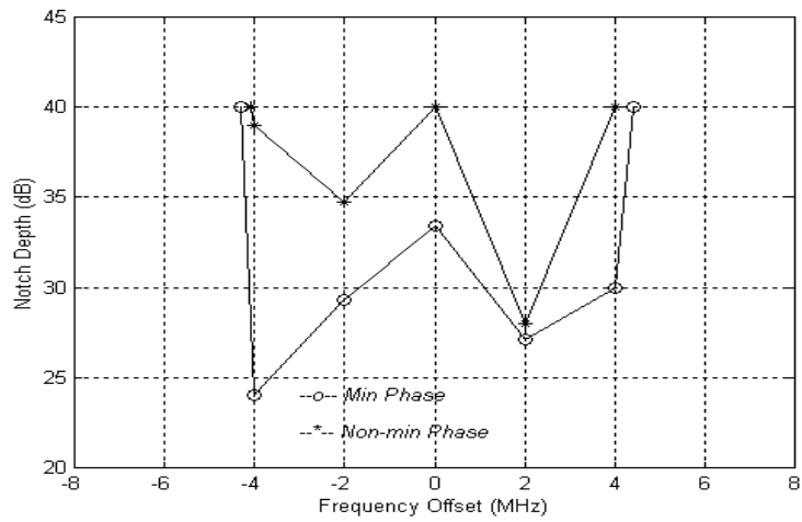
Figure C-3 W Curve at BER=1E-6, Direction A
