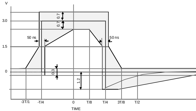
Figure 4-1 Pulse mask for T1
