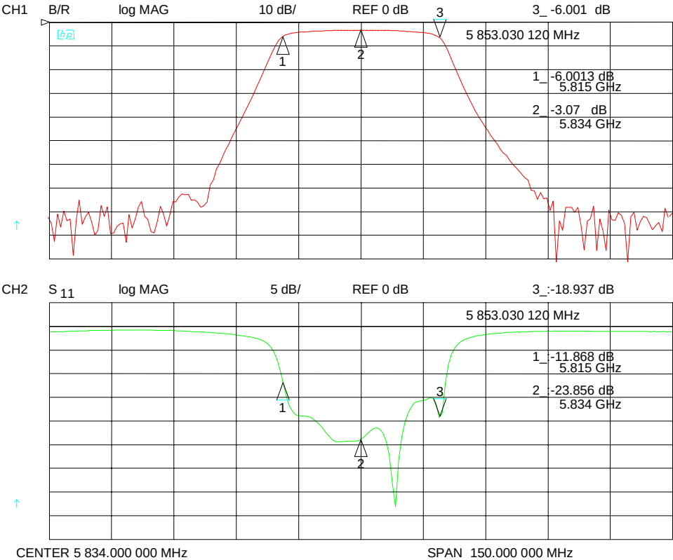
Figure A-10 Filter with center frequency of 5.834 GHz
