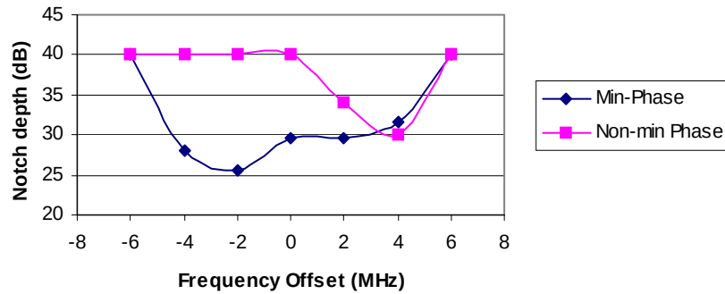
Figure D-3 W Curve at BER=1E-6, Direction A
