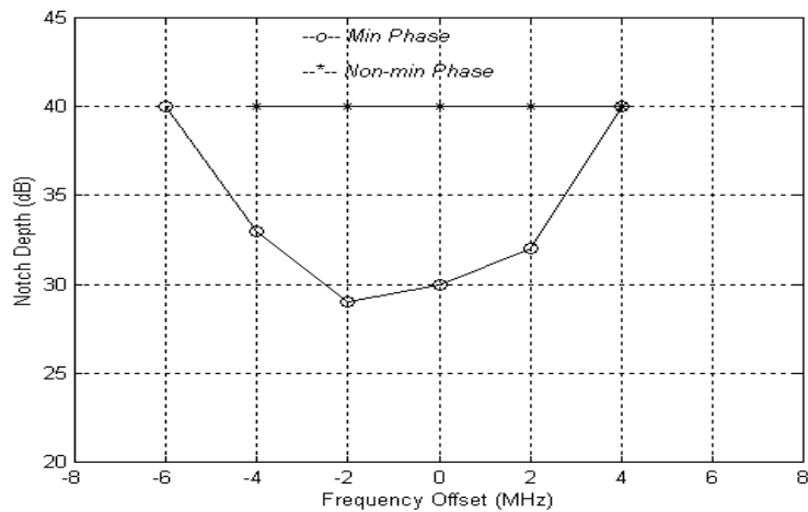
Figure E-4 W Curve at BER=1E-3, Direction A
