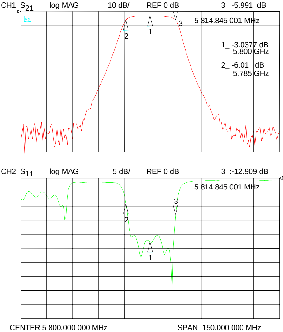
Figure A-4 Filter with center frequency of 5.8 GHz
