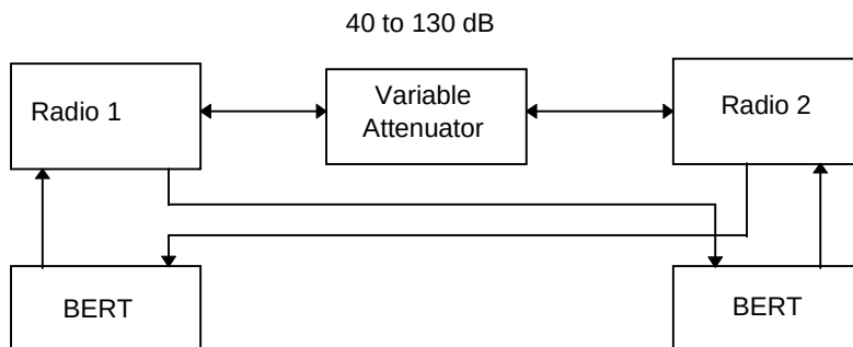
Figure D-2 Receiver test setup
