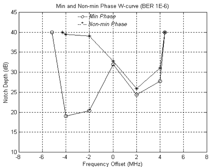
Figure B-3 W Curve at BER=1E-6, Direction A
