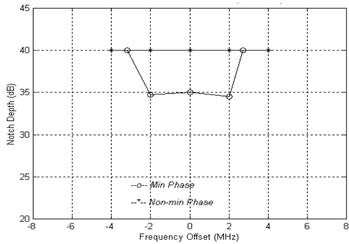
Figure C-6 W Curve at BER = 1E-3, Direction B
