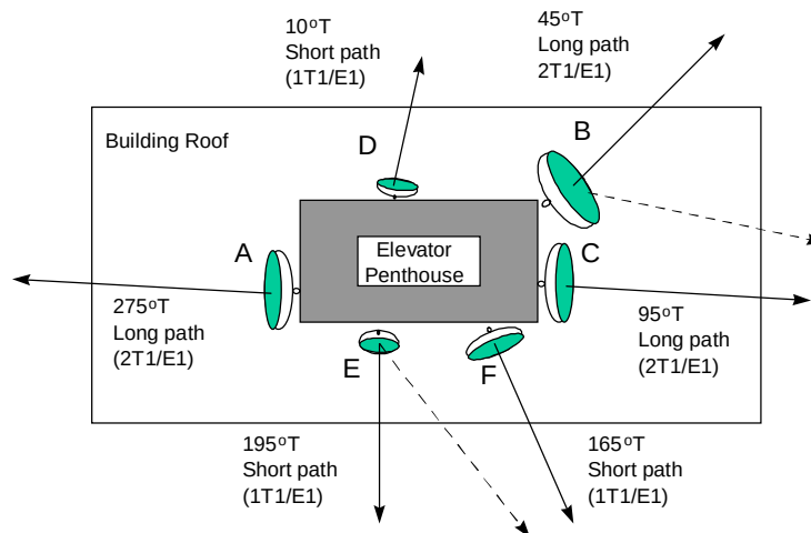
Figure 3-5 Roof mounting with building blockage
