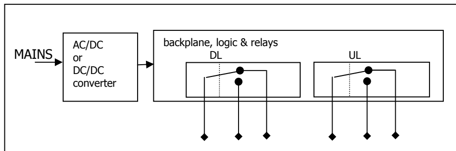
Fig. 24 – TPR block diagram
