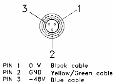
Fig. 39 - VDC connector
