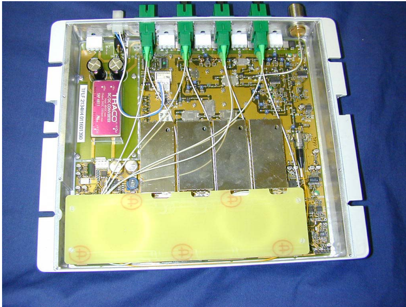
Local Unit Internal
