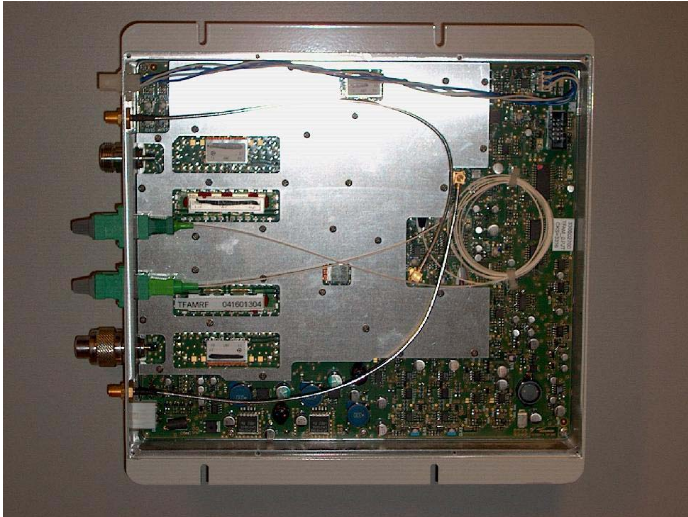
Figure 1 - TFAM23 Top With Shield
