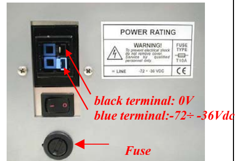
Fig. 13: -72÷-36Vdc connector
