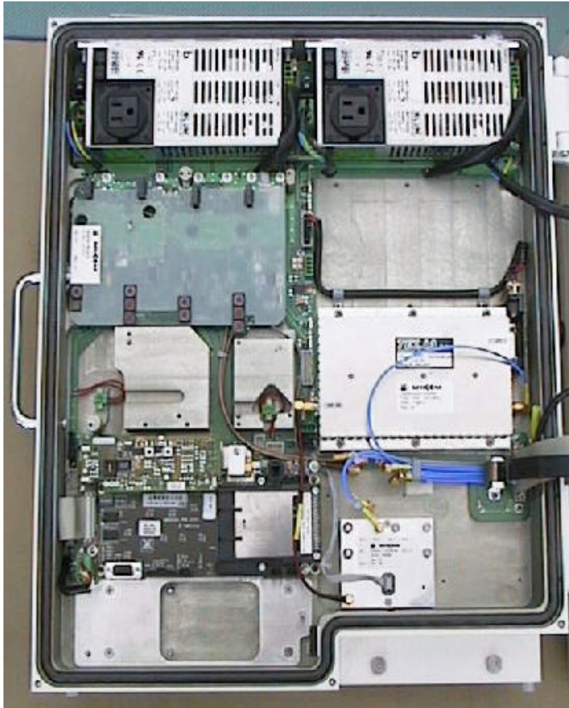
Figure 2 - Left Side of EUT cabinet
