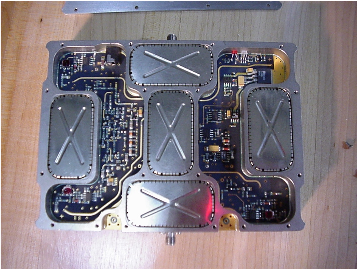
Exhibit E: Top Metal Cover Removed
