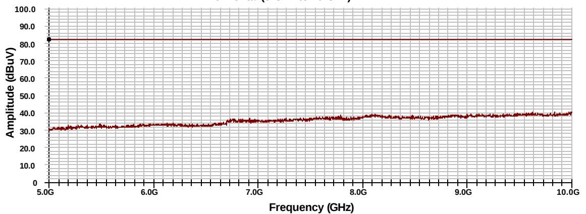
Radiated Emissions Profile (Chamber) Electric Field (3-Meters, Peak Detector) Horizontal (5 GHz to 10 GHz)
