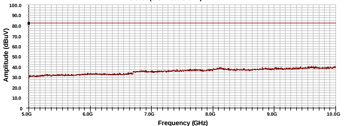
Radiated Emission Profile (Chamber) Electric Field (3-Meters, Peak Detector) Vertical (5 GHz to 10 GHz)
