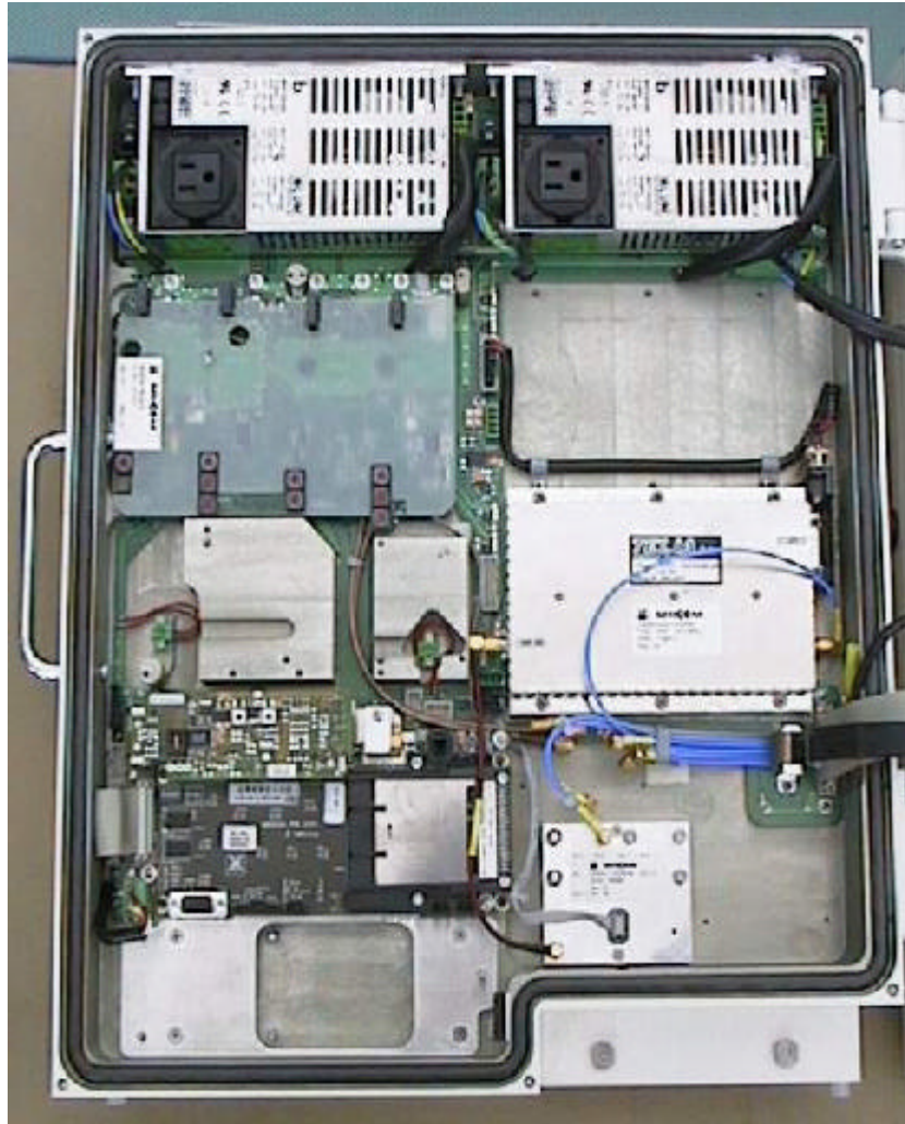
Figure 1 - Left Side of EUT cabinet
