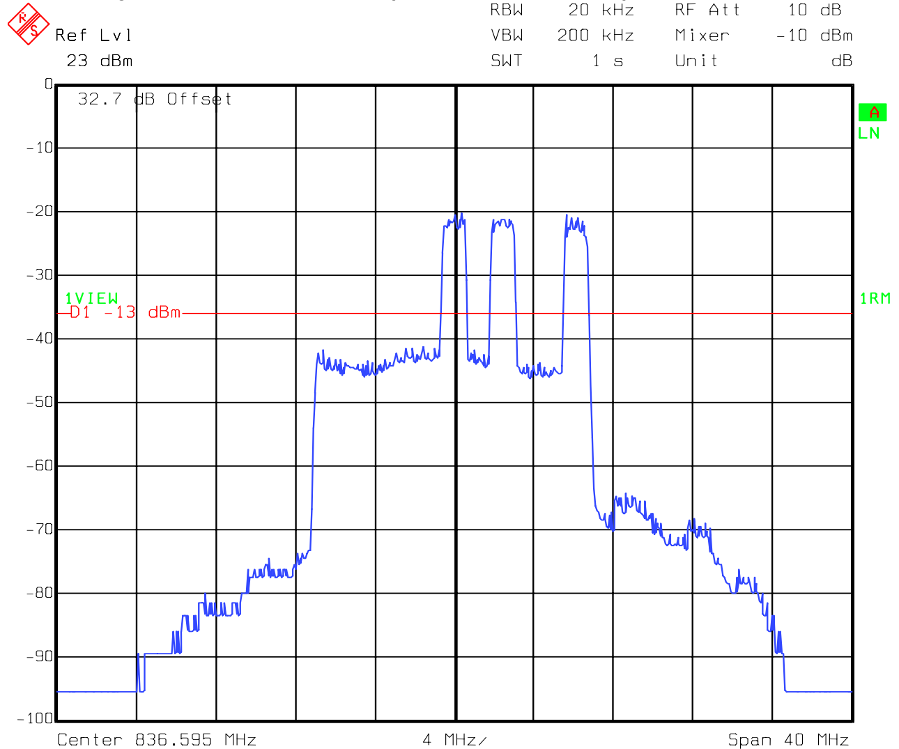
Figure 27 Intermodulation Spurious - IS-95 CDMA - Uplink
