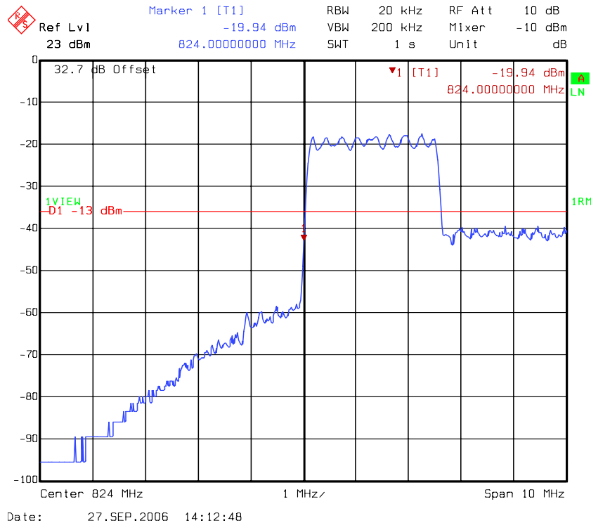
Figure 28 Intermodulation Spurious - IS-95 CDMA - Uplink
