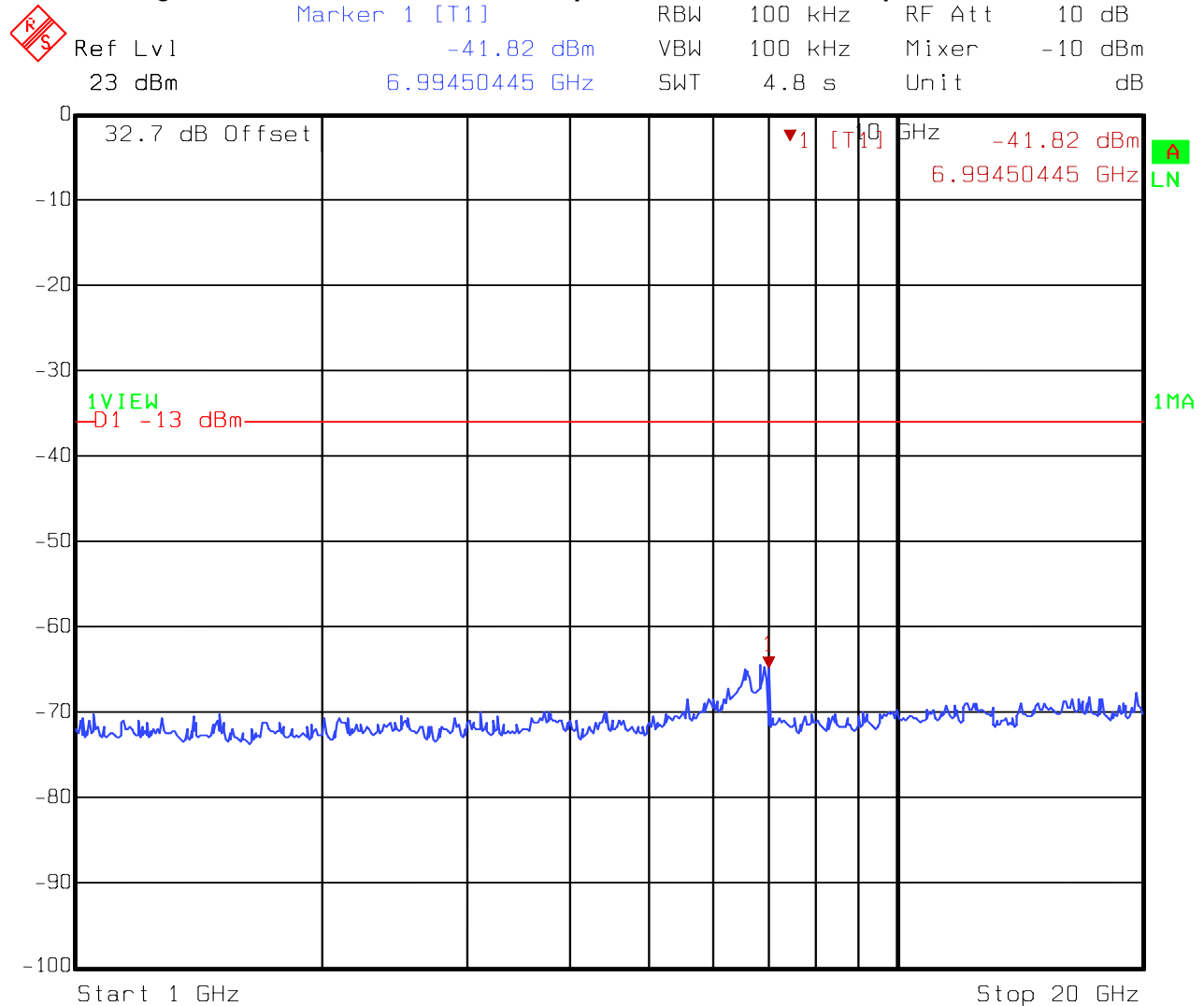
Figure 22 Antenna Conducted Spurious - IS-95 CDMA - Uplink - 1 GHz - 20 GHz
