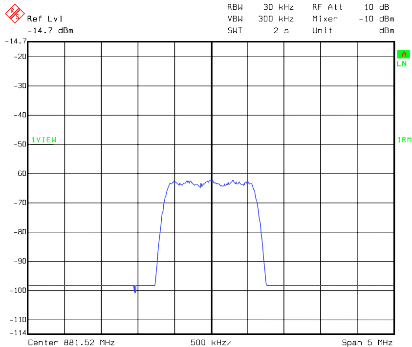
Figure 2 IS-95 CDMA Occupied Bandwidth – Downlink Mid Channel
