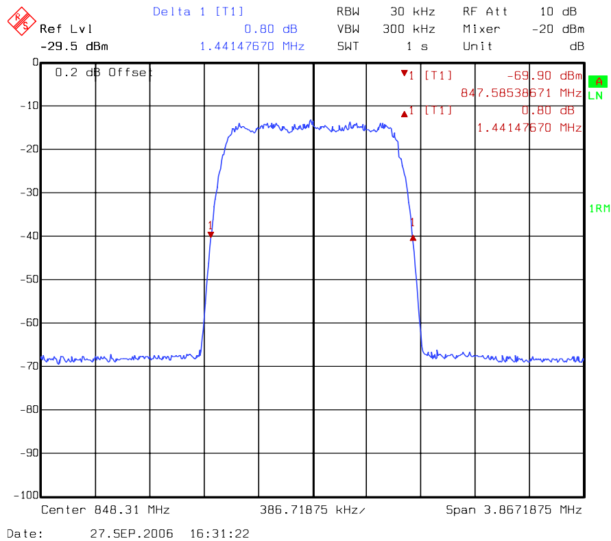
Figure 9 IS-95 CDMA Occupied Bandwidth – Uplink High Channel
