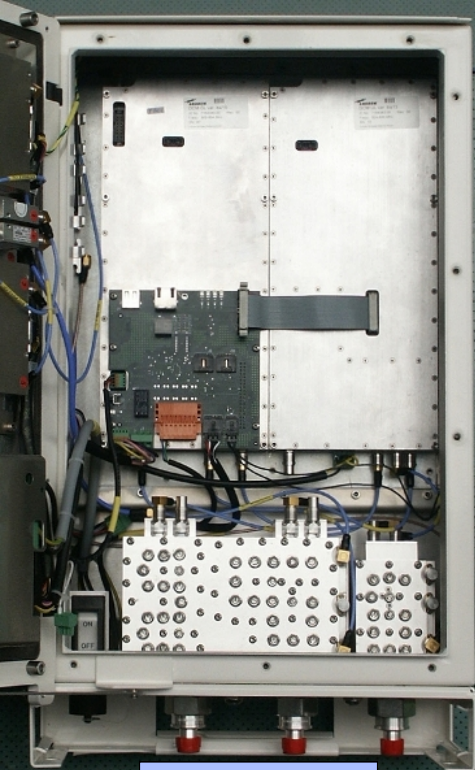
Interior showing components in main chassis
