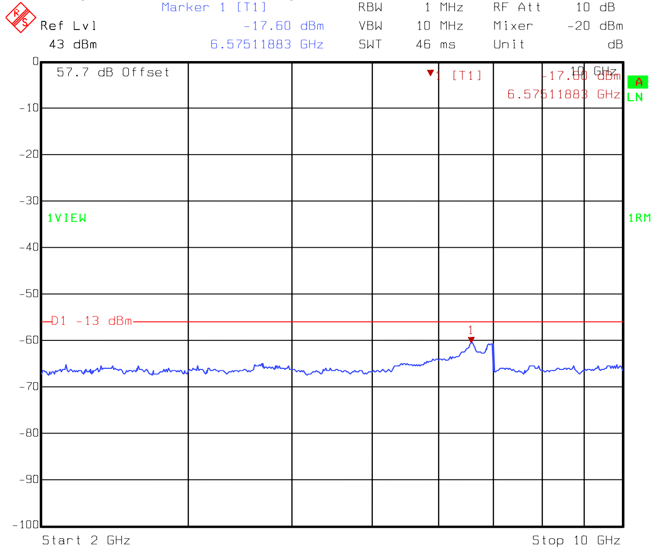
Figure 14 Antenna Conducted Spurious – IS-95 CDMA - Downlink - 2 GHz – 10 GHz
