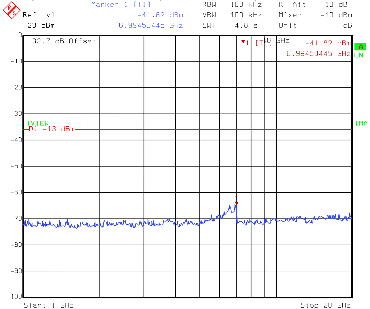
Figure 18 Antenna Conducted Spurious - IS-95 CDMA - Uplink - 1 GHz - 20 GHz
