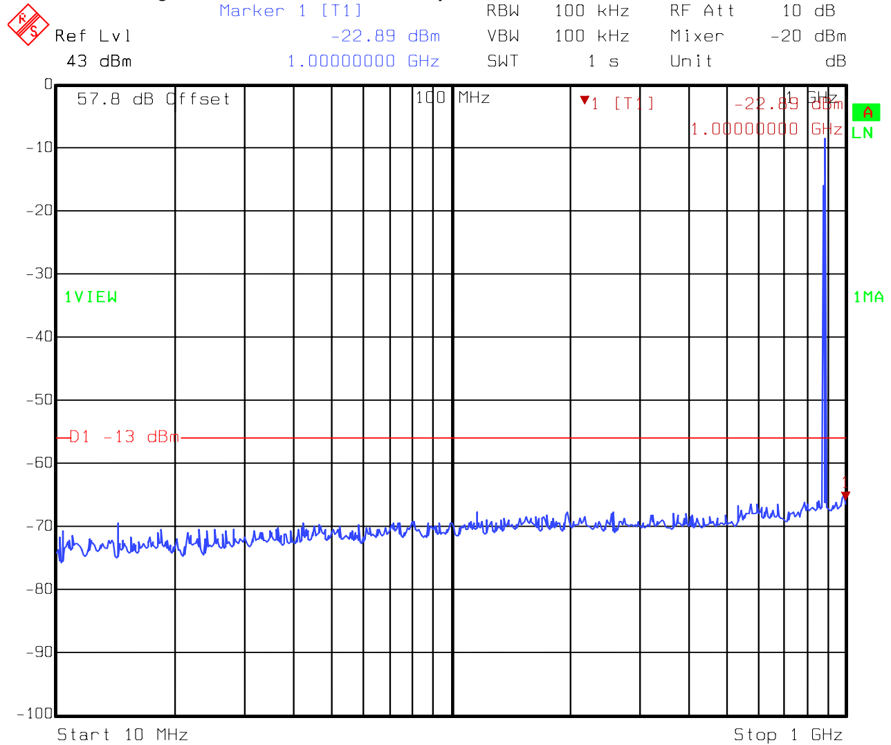
Figure 15 Antenna Conducted Spurious - WCDMA - Downlink - 10 MHz - 1 GHz
