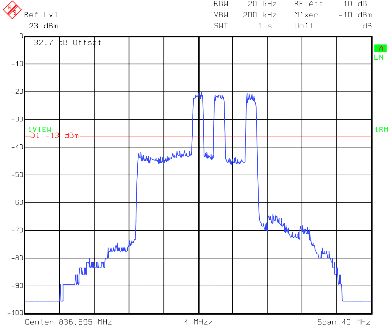
Figure 23 Intermodulation Spurious - IS-95 CDMA - Uplink
