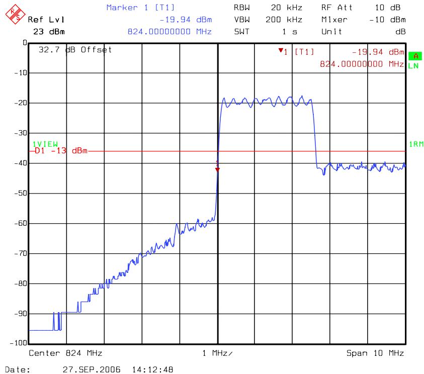
Figure 24 Intermodulation Spurious - IS-95 CDMA - Uplink
