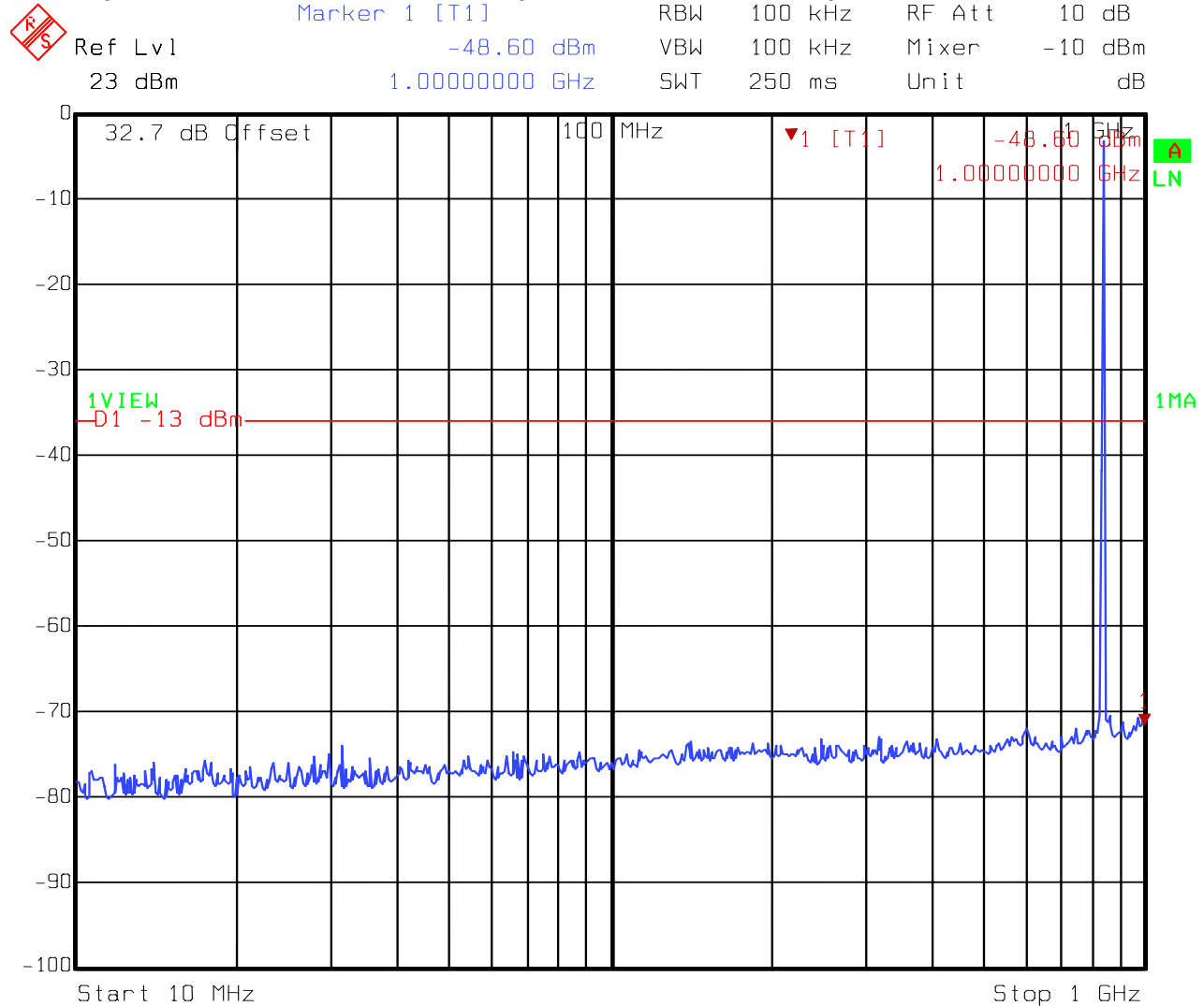
Figure 17 Antenna Conducted Spurious - IS-95 CDMA - Uplink - 10 MHz - 1 GHz
