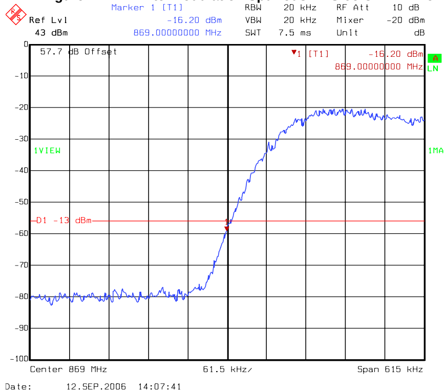
Figure 22 Intermodulation Spurious - IS-95 CDMA - Downlink
