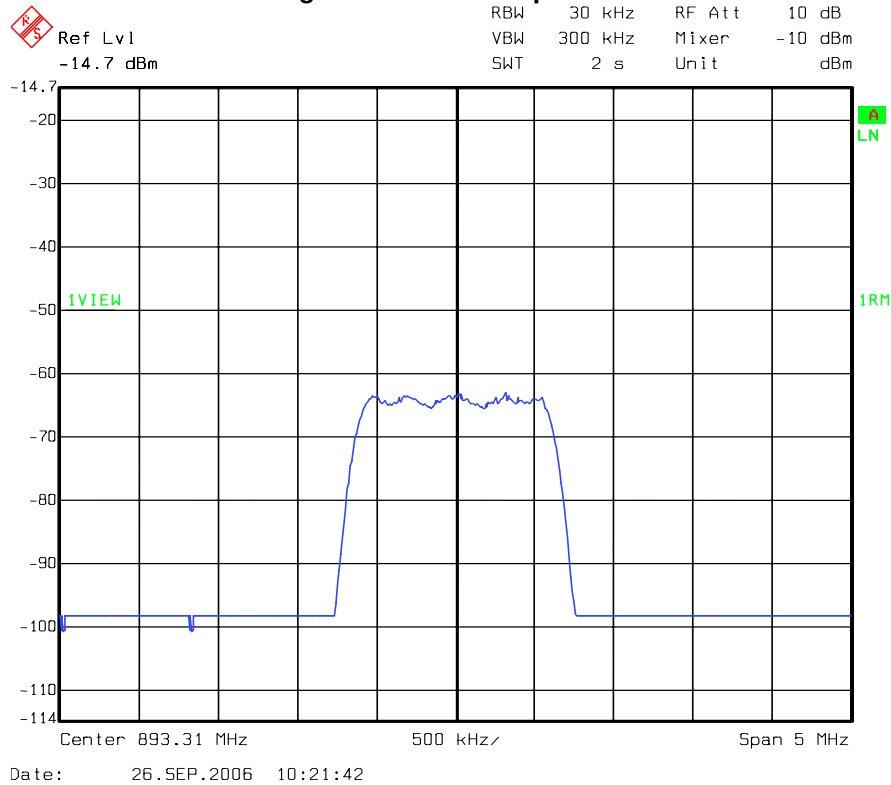
Figure 3 IS-95 Occupied Bandwidth – Downlink High Channel
