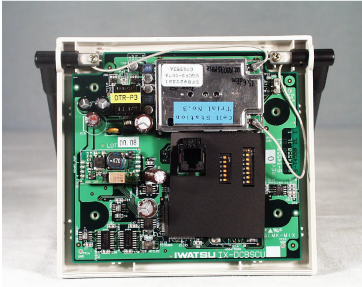
Inside View of the IX-BS5
