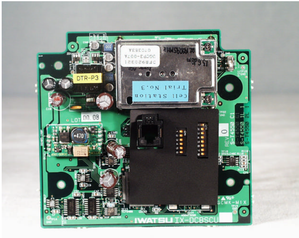
Component side (with RF cans)
