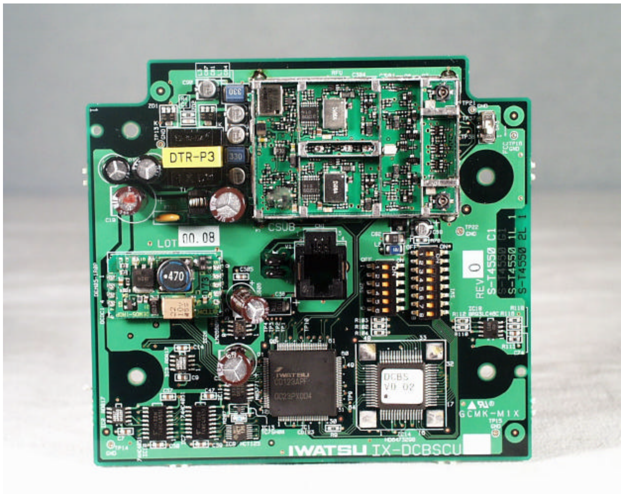
Component side (without RF cans and static protection)
