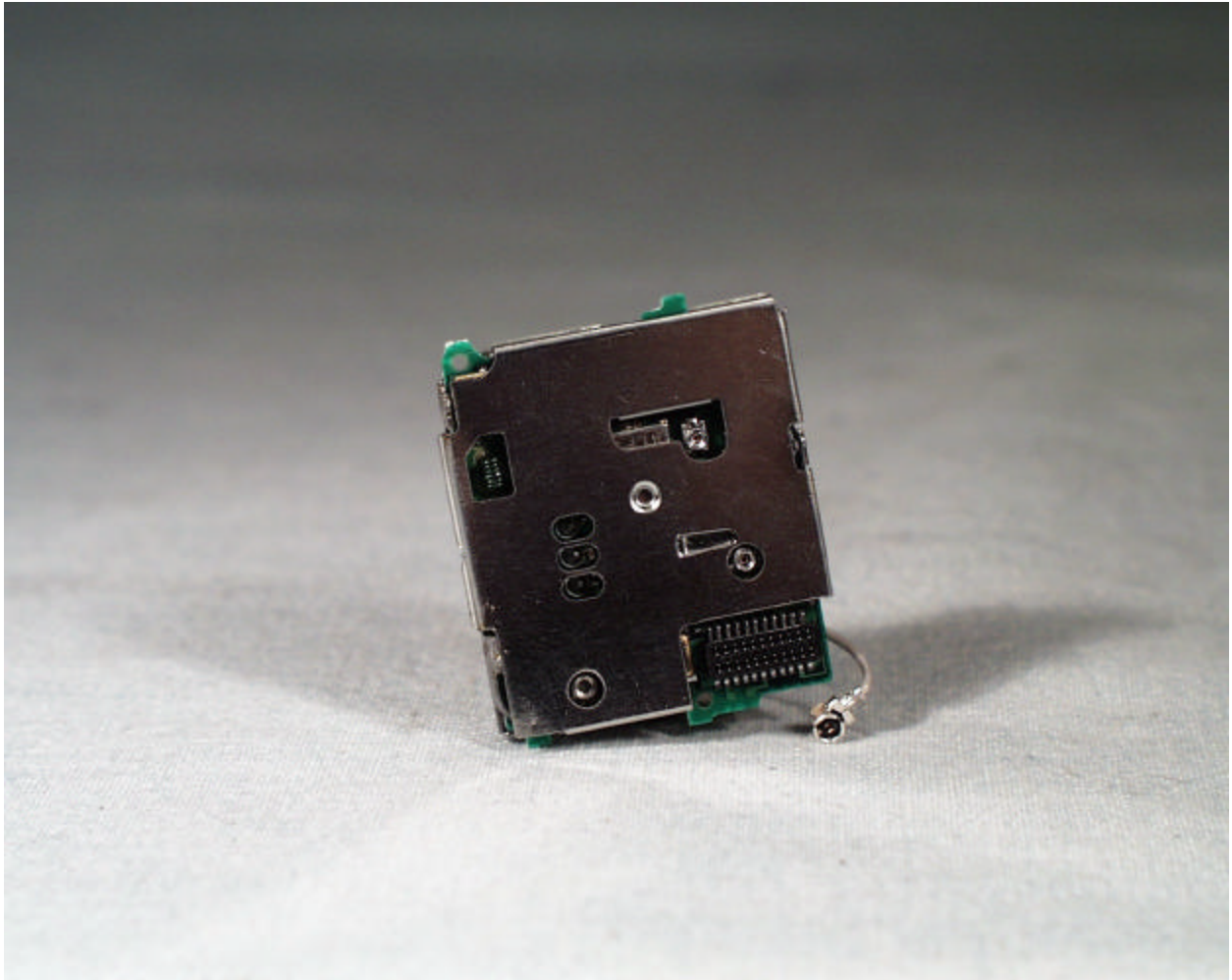
Side A of the RF board (with RF cans)
