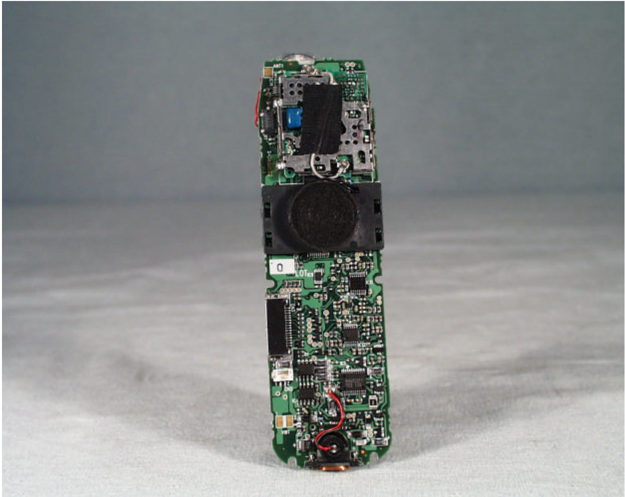
Side A of the Digital board and RF board
