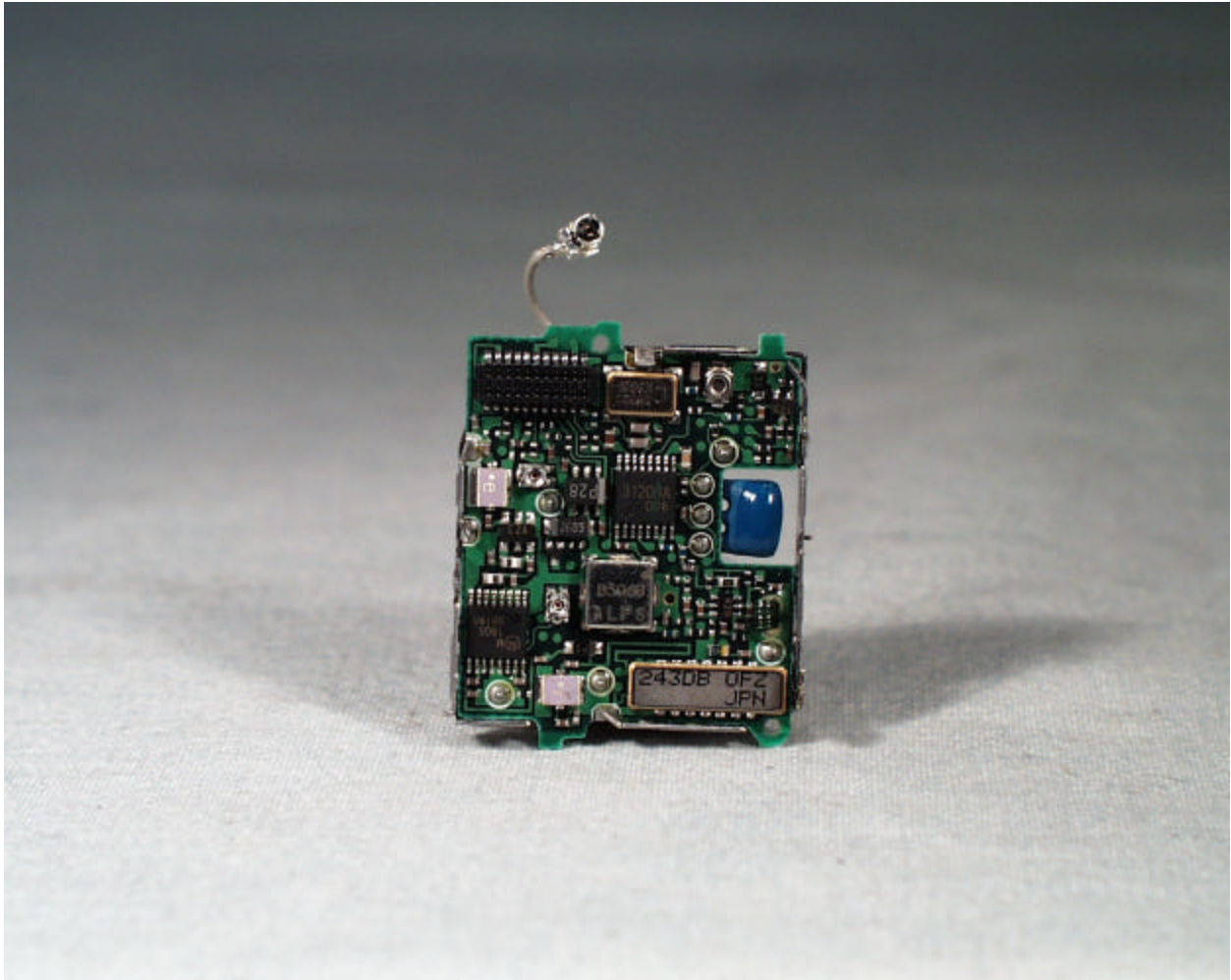
Side A of the RF board (without RF cans)
