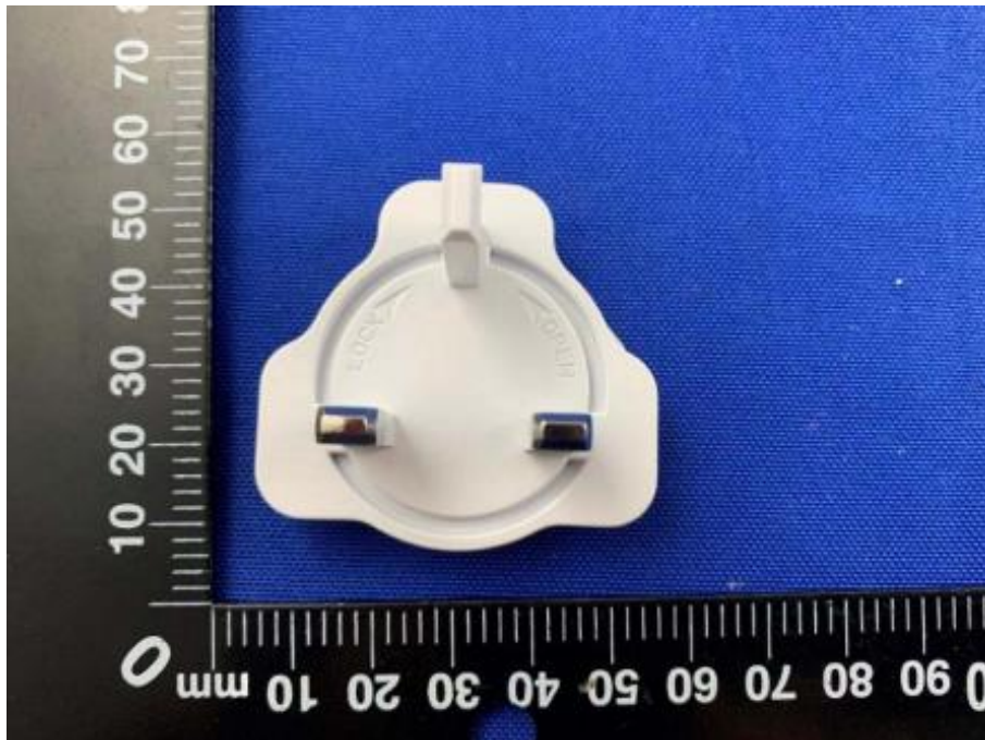
Accessory-Power Adapter 3
