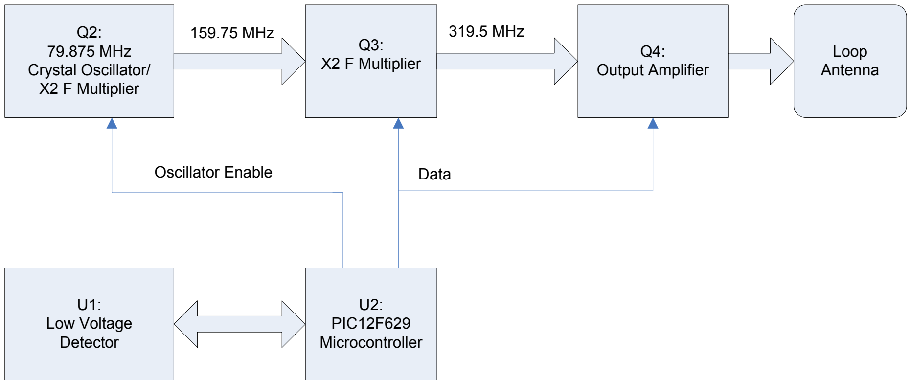
Block Diagram of SX319 PHB
