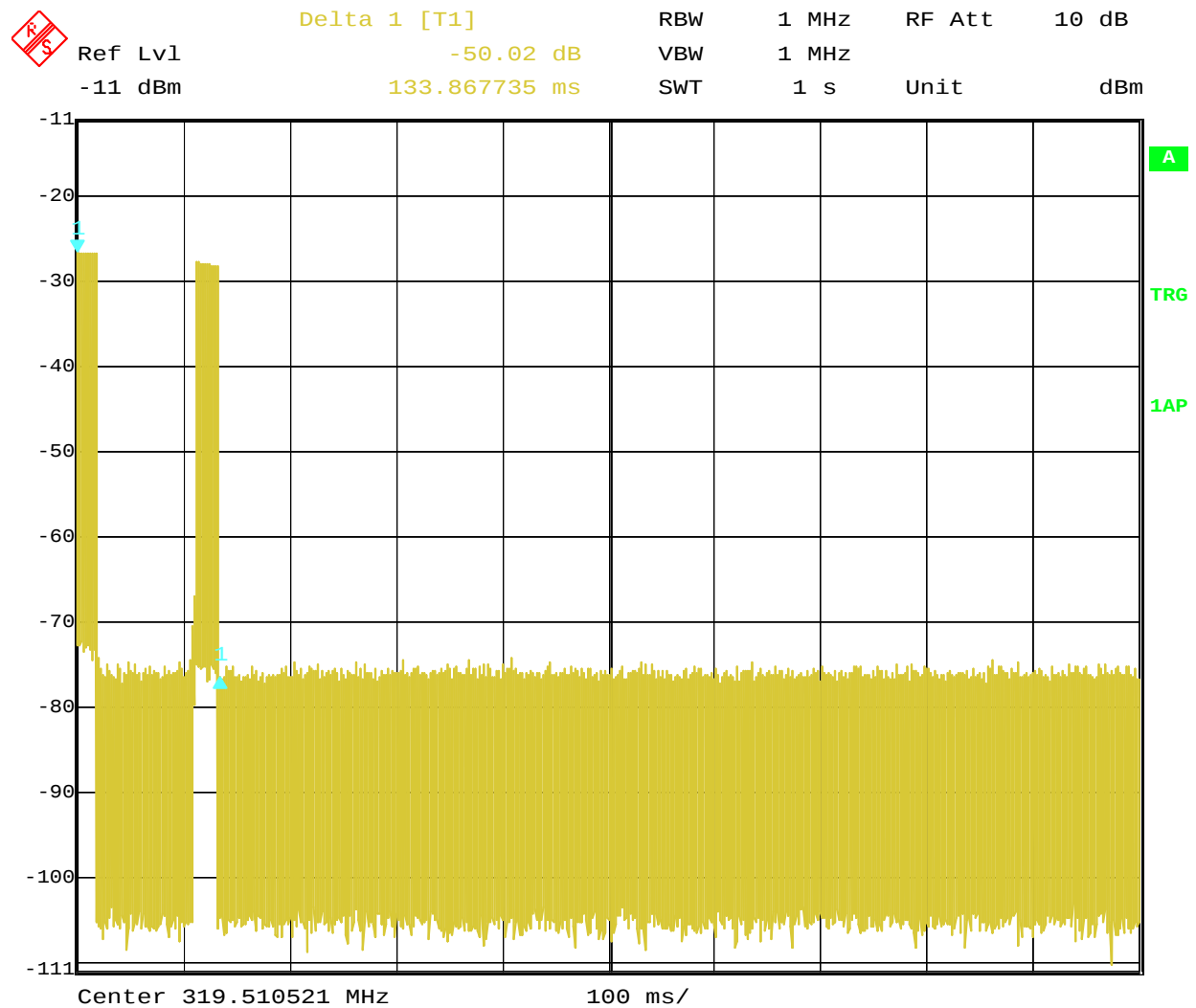
Figure 4-2: Deactivation Plot
