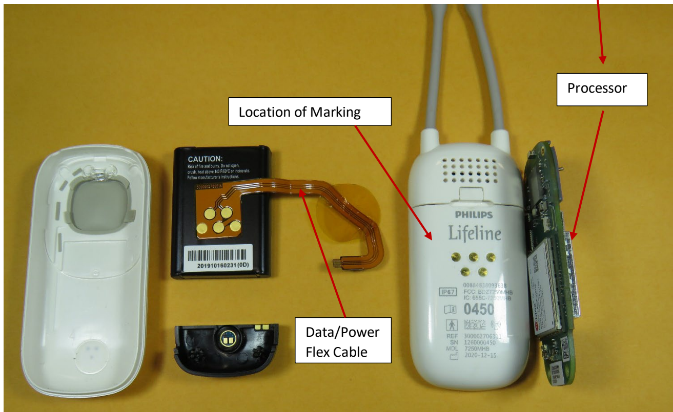
Internal View (PCB, Battery Speaker)
