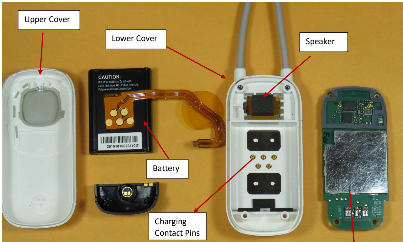
Internal View (PCB, Battery Speaker)
