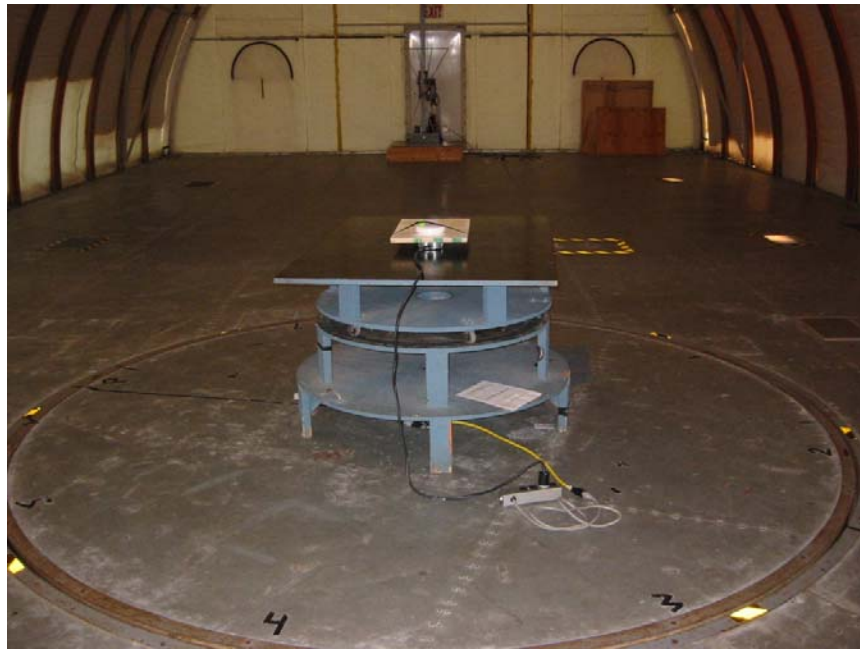
Radiated Spurious Test Setup, Front View
