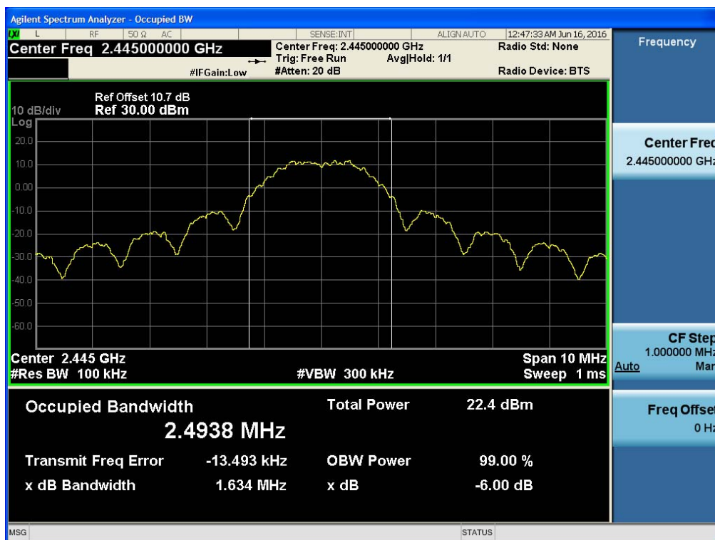
99% Bandwidth plot (CH 19)
