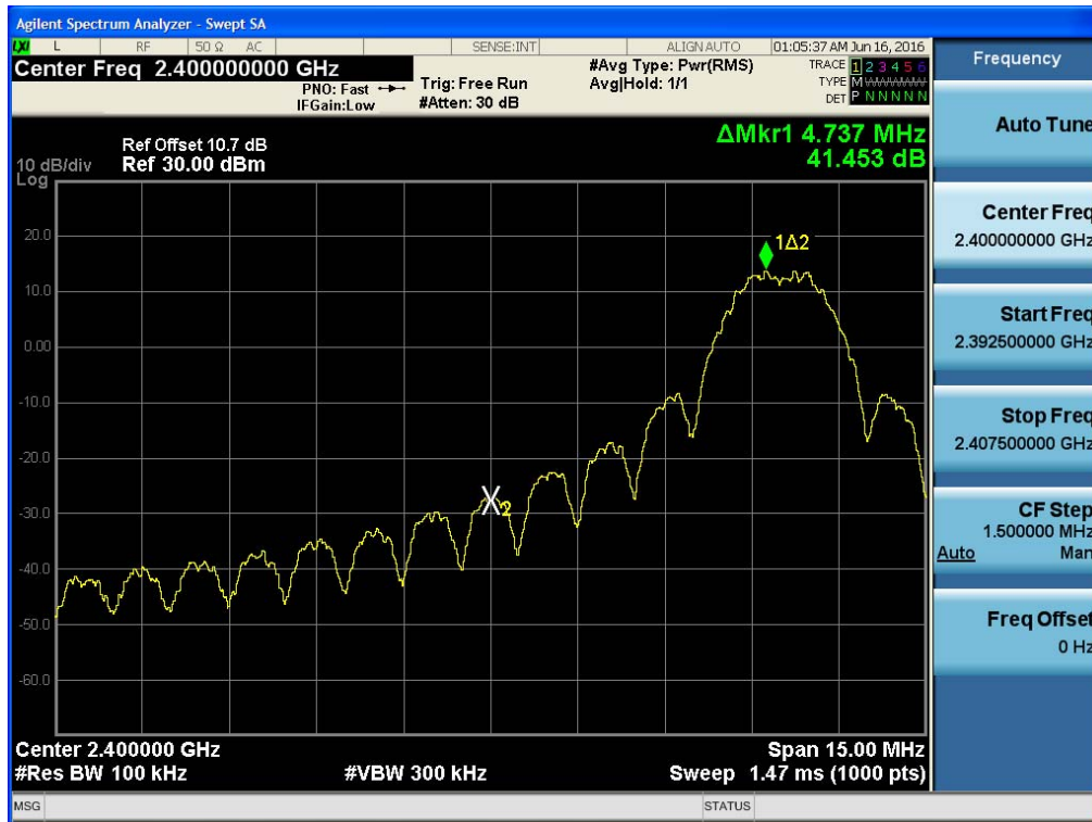
BandEdge (CH 11)
