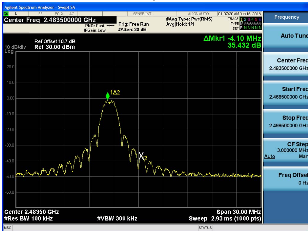
BandEdge (CH 26)
