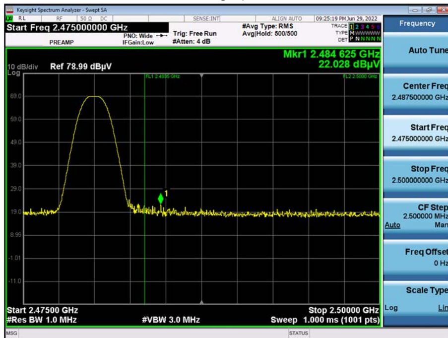
Radiated Restricted Band Edges plot – Peak Result (Ch.39, V)
