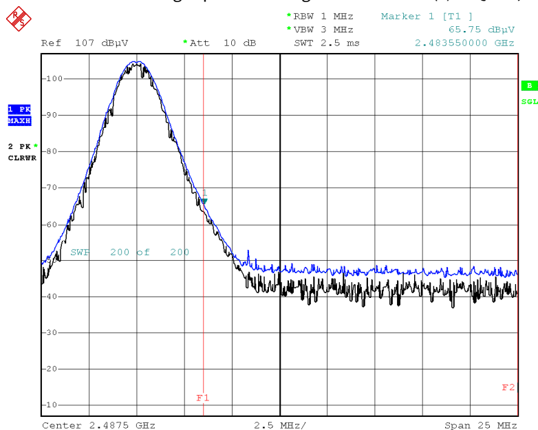
Radiated Restricted Band Edges plot – Average & Peak Result ( \pi/4 DQPSK, Ch.78, V)
