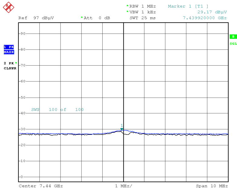
Radiated Spurious Emissions plot – Average Result (GFSK, Ch78 3rd Harmonic, H)
