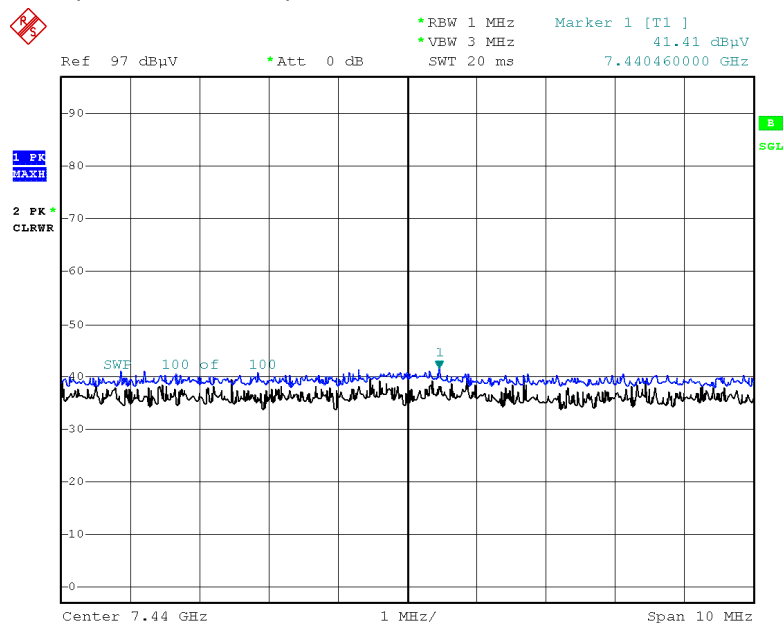
Radiated Spurious Emissions plot – Peak Result (GFSK, Ch.78 3rd Harmonic, H)
