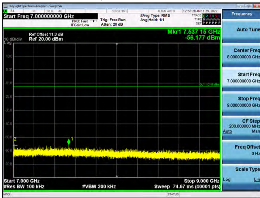
Conducted Spurious Emission (7 GHz ~ 9 GHz)
