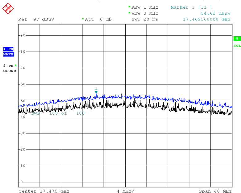
Peak Measured Level (802.11a, Ch.165 3rd Harmonic, Y-H)
