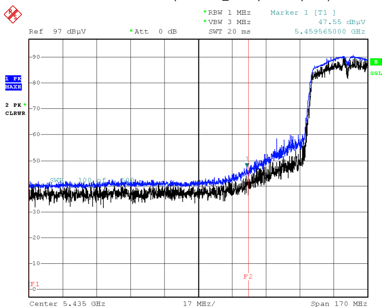
Peak Measured Level (802.11 n_HT40, Ch.102, X-H)
