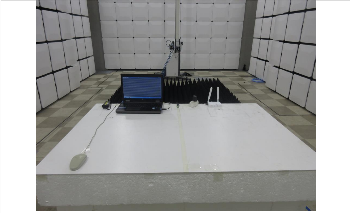
[ 18 GHz to 40 GHz ] Without Case
