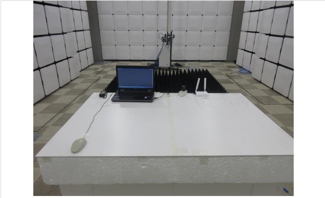
[ 18 GHz to 40 GHz ] With Case
