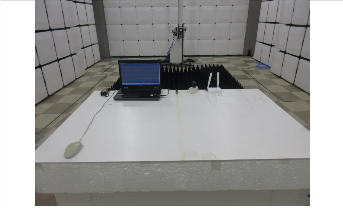
[ 1 GHz to 18 GHz ] Without Case
