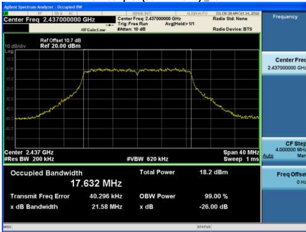
99% Bandwidth plot (802.11n-CH6) _20 MHz BW
