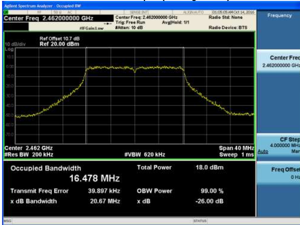
99% Bandwidth plot (802.11g- CH 11)
