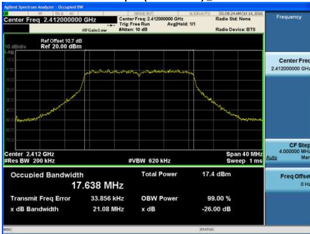
99% Bandwidth plot (802.11n-CH1) _20 MHz BW
