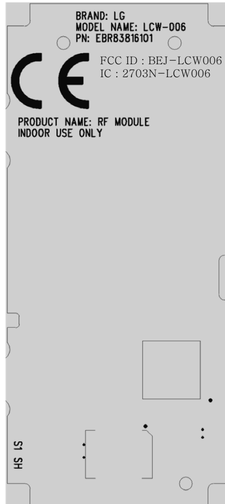
< Bottom side - silk printing >
