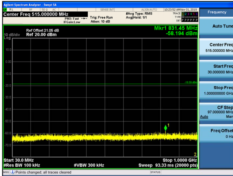
Conducted Spurious Emission (802.11g_Ch.1)
