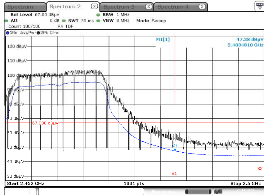
Radiated Restricted Band Edges plot – Average Result (802.11g, 6 Mbps, Ch.11, Y-V)
