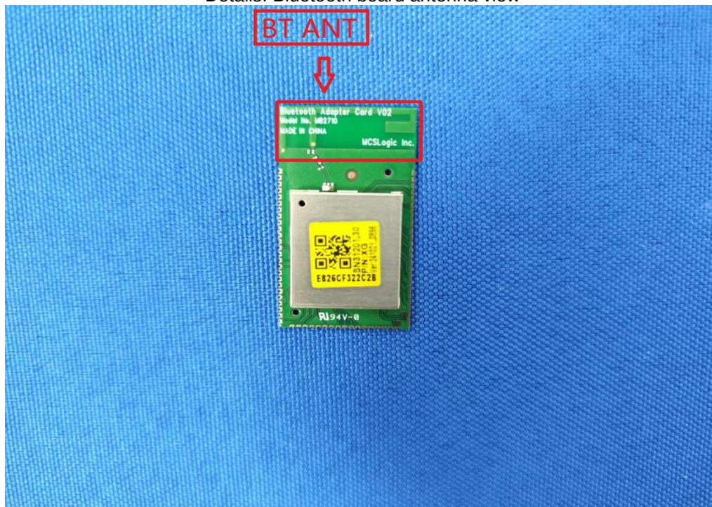
Details: Bluetooth board antenna view
