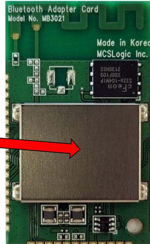
Printed label on the shielding can
