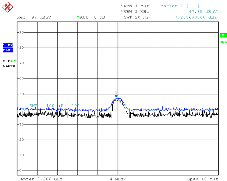
Radiated Spurious Emissions plot – Peak Result (GFSK, Ch.0 3rd Harmonic, Z-H)
