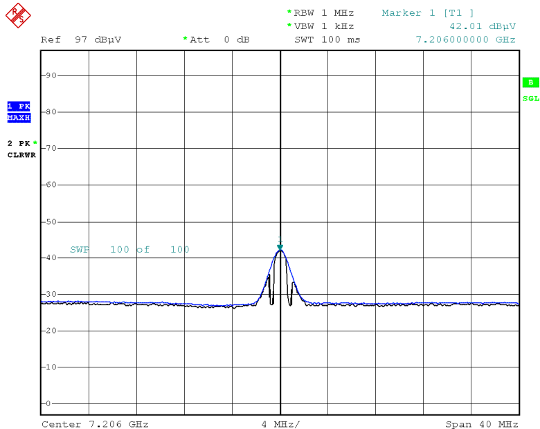
Radiated Spurious Emissions plot – Average Result (GFSK, Ch.0 3rd Harmonic, Z-H)
