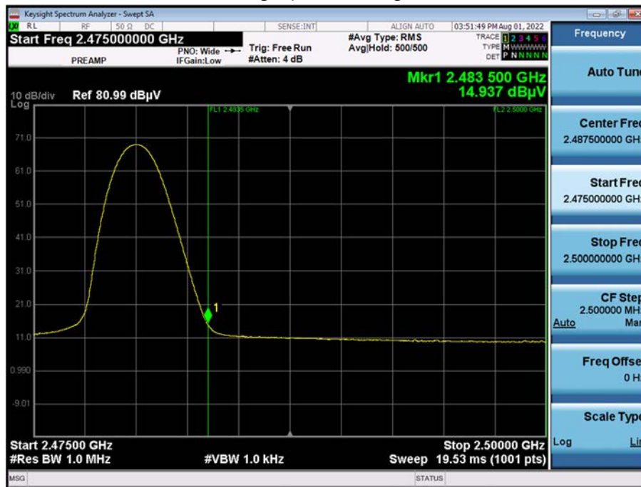
Radiated Restricted Band Edges plot –Peak Result (8DPSK, Ch.78, X-H)
