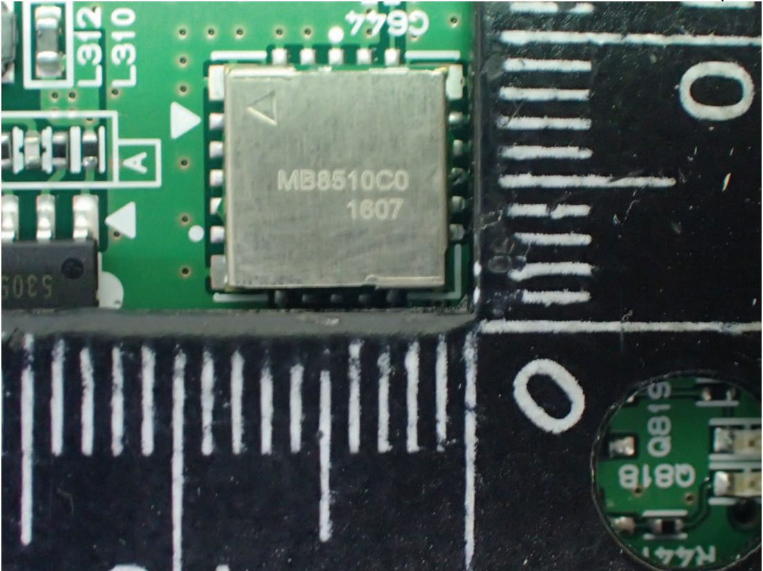
Figure 12 Internal View (BT Module)
