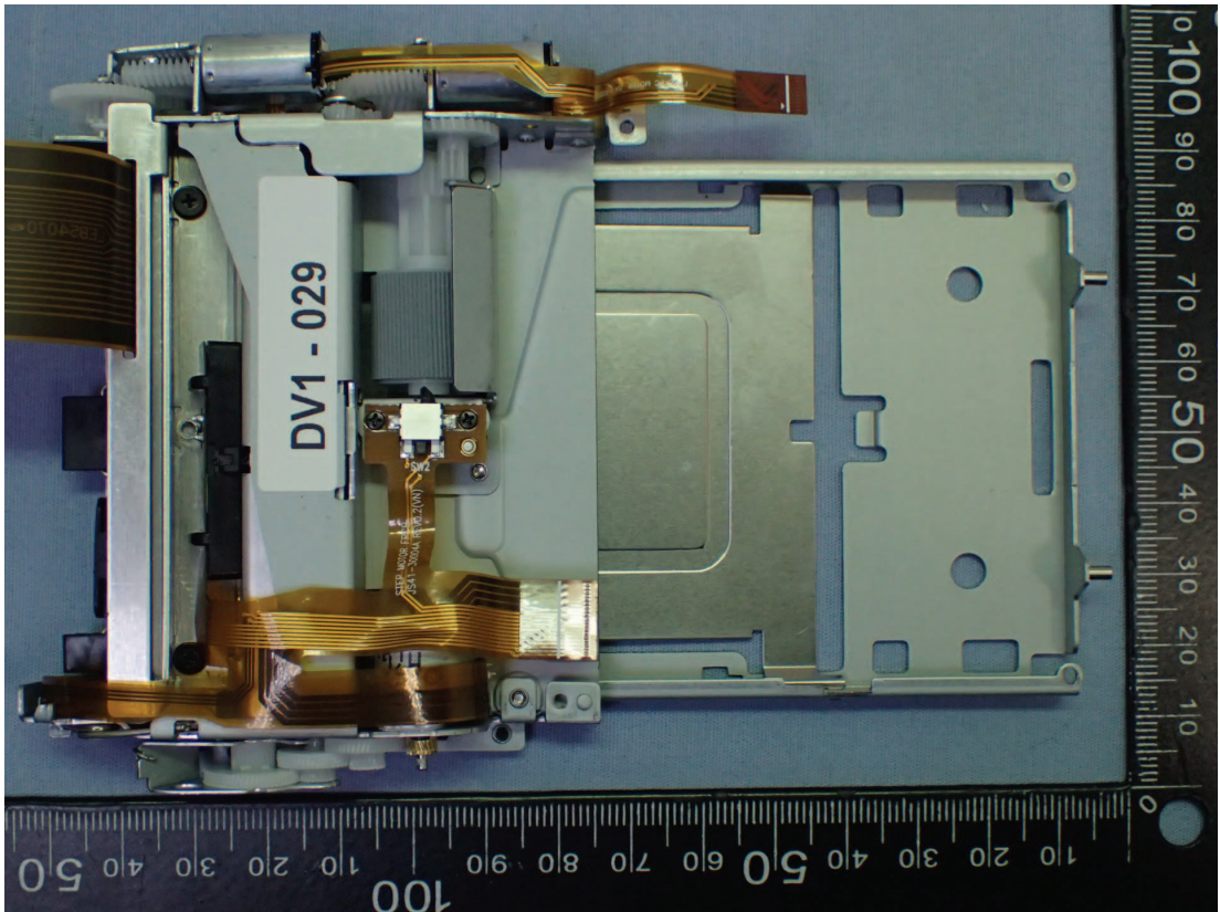
Figure 16 Internal View
