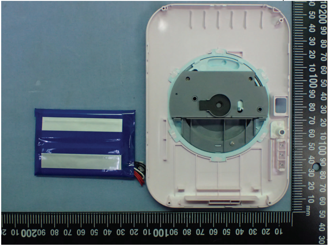
Figure 7 Internal View (Removed Battery)
