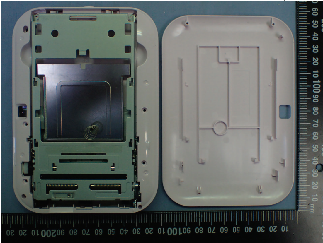
Figure 5 Internal View (Removed Cover)
