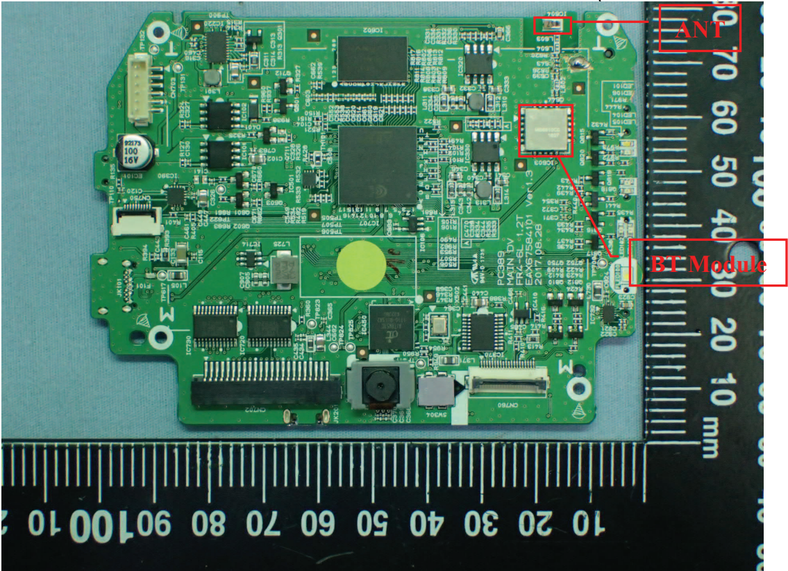
Figure 10 Internal View (Main Board, Front View)
