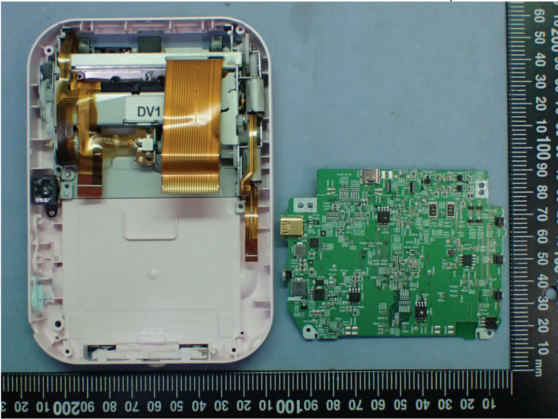
Figure 9 Internal View (Removed Main Board)
