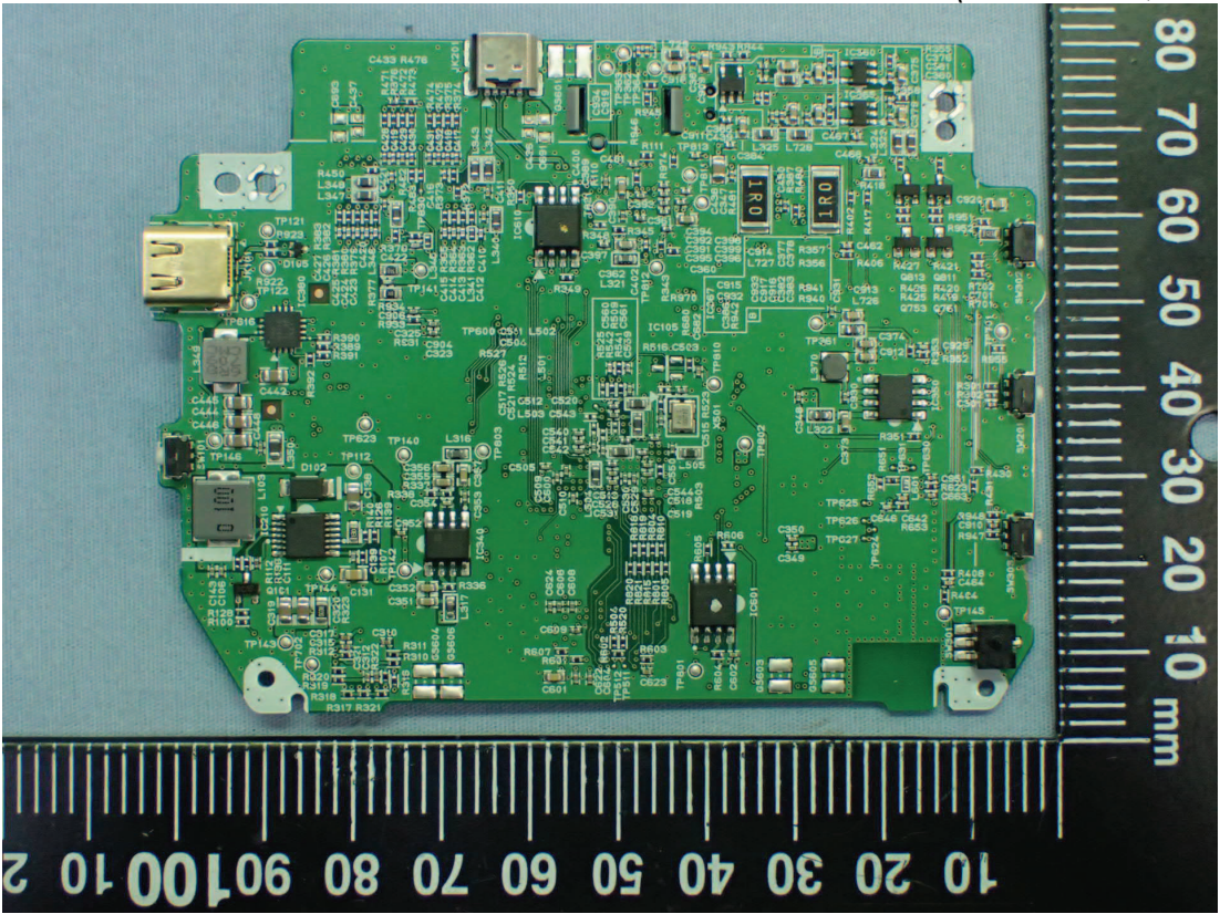
Figure 11 Internal View (Main Board, Back View)
