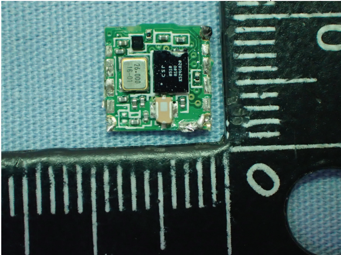
Figure 13 Internal View (BT Module, Front View)
