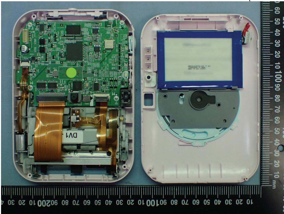
Figure 6 Internal View (Removed Cover)
