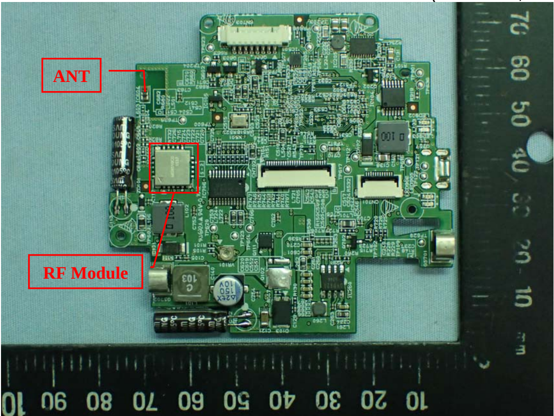
Figure 27 Internal View (Main Board, Front View)
