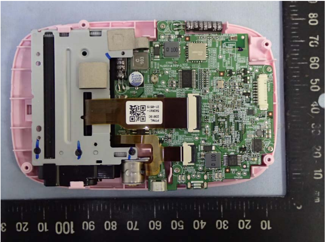
Figure 26 Internal View
