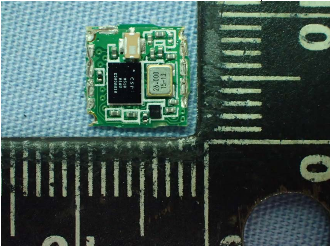
Figure 30 Internal View (RF Module, Front View)
