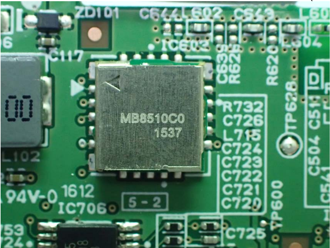
Figure 29 Internal View (RF Module)
