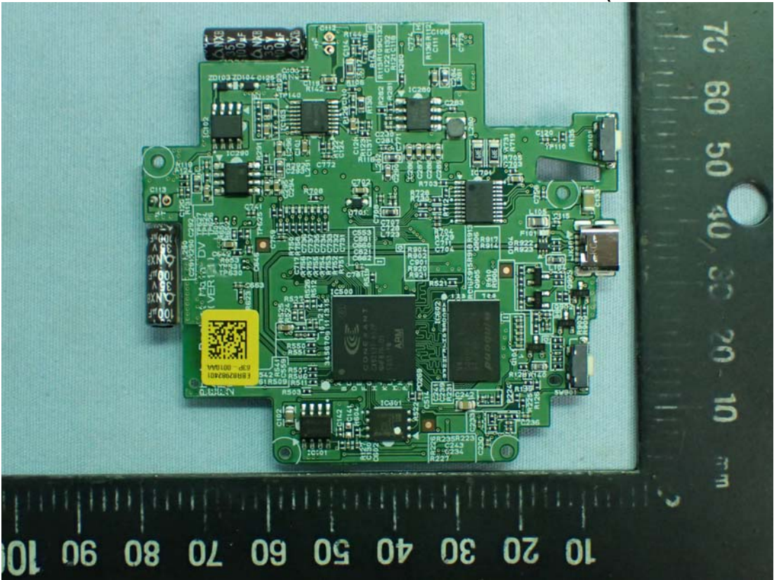
Figure 28 Internal View (Main Board, Back View)
