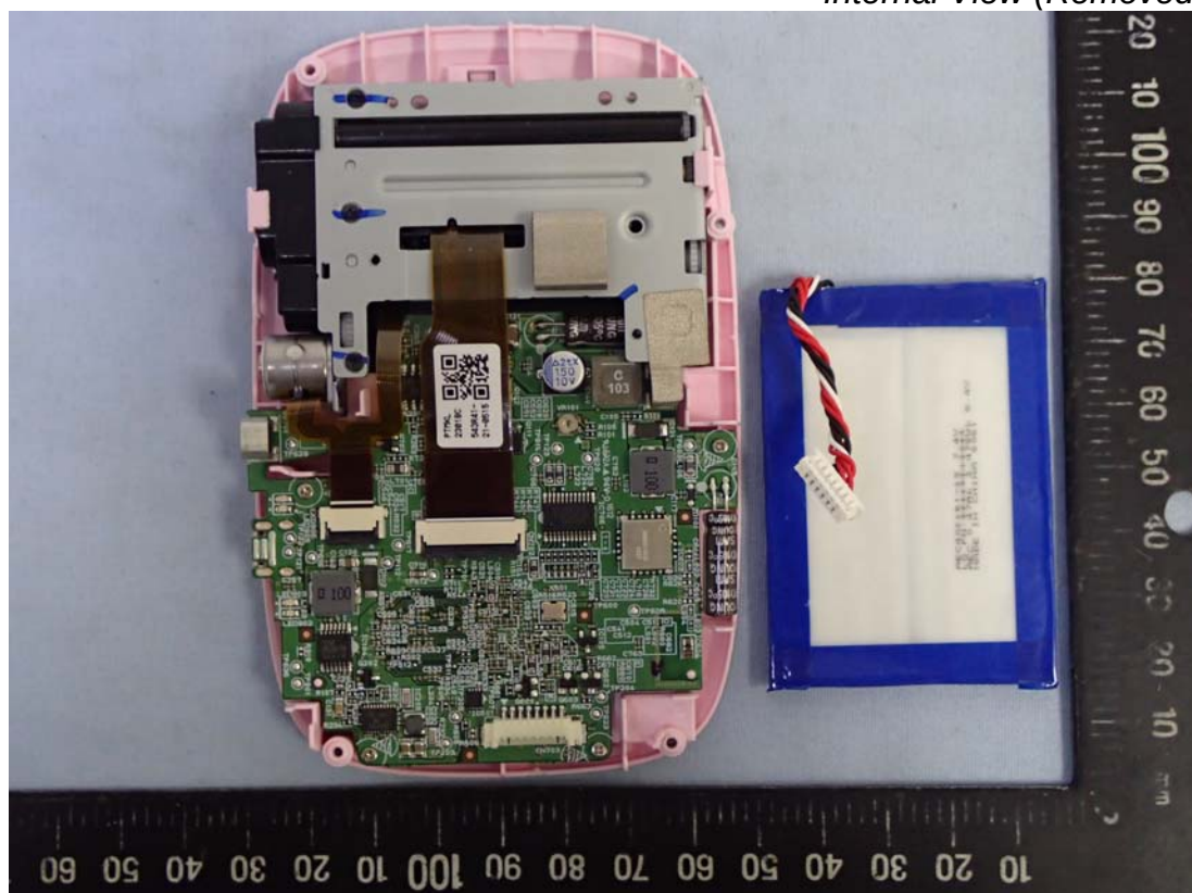
Figure 24 Internal View (Removed Battery)
