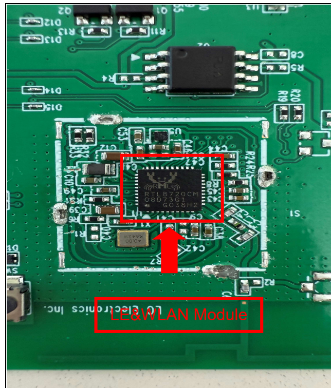
View of Bluetooth & WLAN Module (without shielding)
