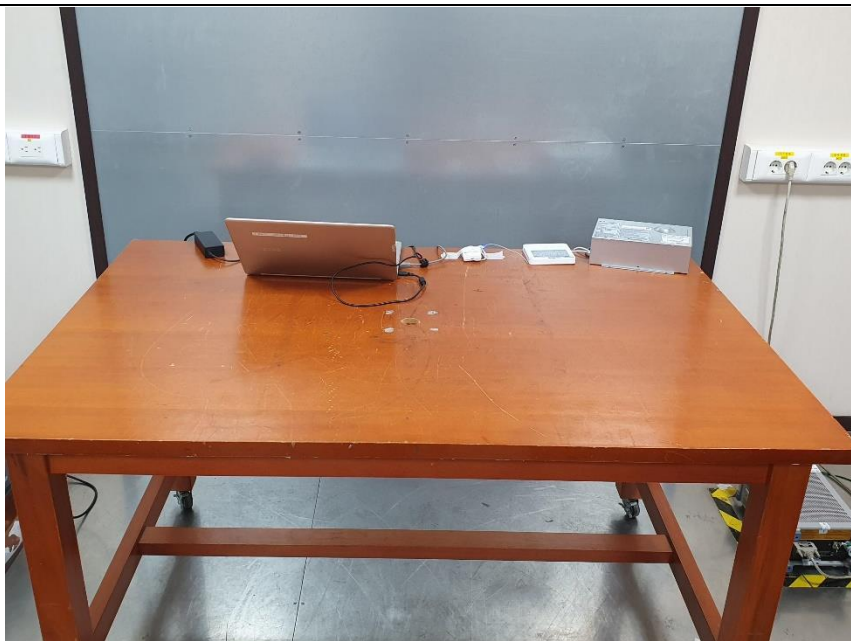
[Rear view of Continuous Conducted Emission at main]
