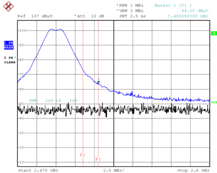
Radiated Restricted Band Edges plot – Peak & Average Reading (CH.26: 2485.5 MHz)
