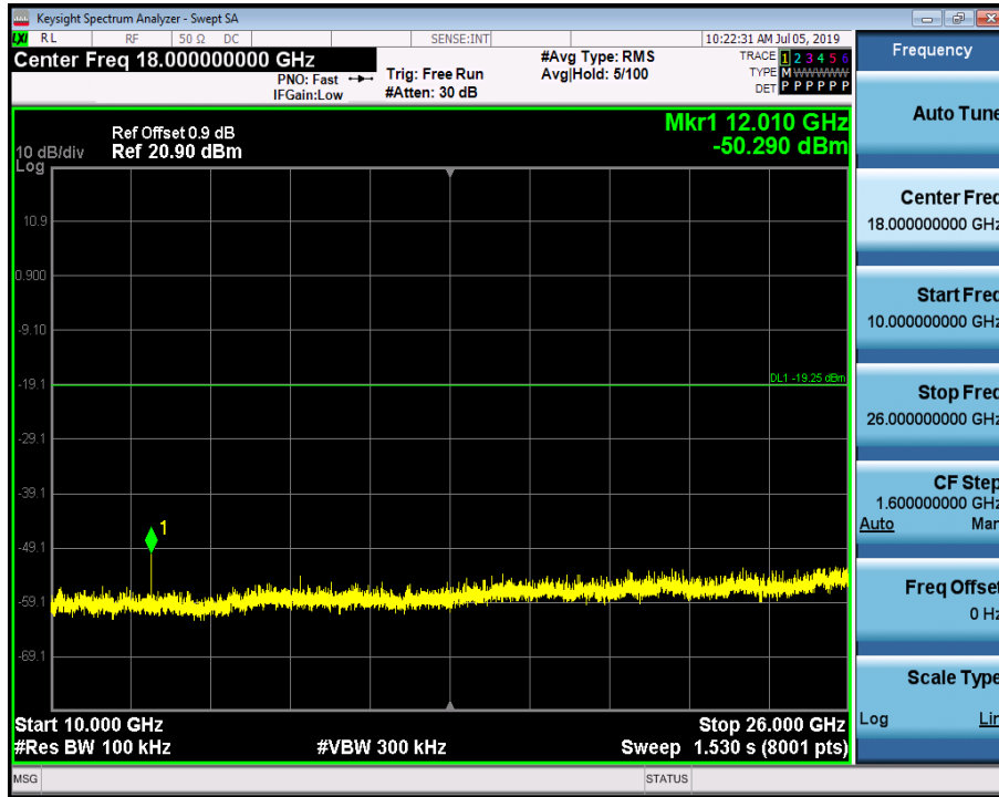
RF Conducted Spurious Emissions_DH5_2441
