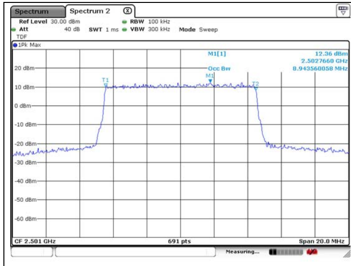
Low Channel
