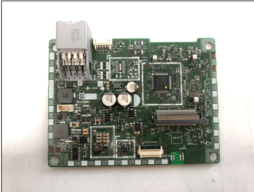
Bottom view of Jig
